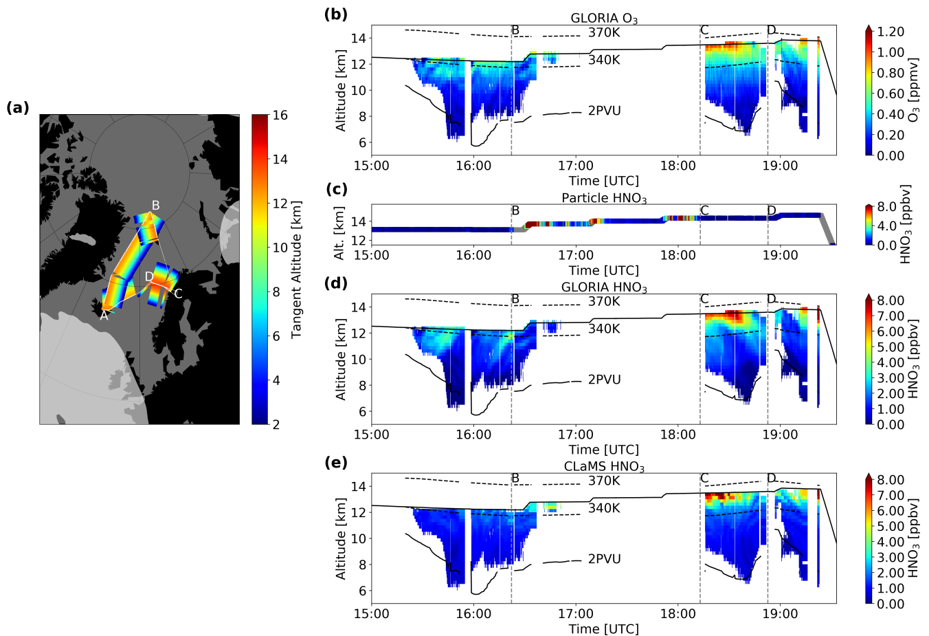
Figure 2. (a) Flight path and vortex filtering according to the Nash criterion at 370 K for flight 8 on 20 January 2016. White line: flight track with characteristic waypoints (A, B, C, D); dark grey shading: areas that are associated with the polar vortex. (b) Cross-section of O 3 distribution derived from GLORIA for flight 8 on 20 January 2016. Flight altitude (bold black line), characteristic waypoints (B, C, D), 340 K and 370 K potential temperature levels (MERRA-2, dashed black lines) and 2 PVU level (MERRA-2, black line). (c) Particulate nitrate measurements at flight altitude for flight 8 on 20 January 2016 (not enhancement corrected). (d) Cross-section of HNO 3 distribution derived from GLORIA and (e) HNO 3 distribution simulated by CLaMS for flight 8 on 20 January 2016. Flight altitude (bold black line), characteristic waypoints (B, C, D), 340 K and 370 K potential temperature levels (MERRA-2, dashed black lines) and 2 PVU level (MERRA-2, black line). The cross-sections and particulate nitrate measurements show only the flight part after waypoint A.
