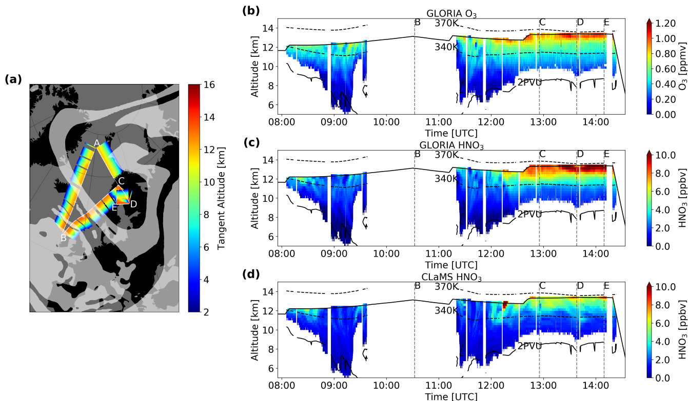
Figure 3. (a) Flight path and vortex filtering according to the Nash criterion at 370 K for flight 12 on 31 January 2016. White line: flight track with characteristic waypoints (A, B, C, D, E); dark grey shading: areas that are associated with the polar vortex. Cross-sections of (b) O 3 and (c) HNO 3 distribution derived from GLORIA and (d) HNO 3 distribution simulated by CLaMS for flight 12 on 31 January 2016. Flight altitude (bold black line), characteristic waypoints (B, C, D, E), 340 K and 370 K potential temperature levels (MERRA-2, dashed black lines) and 2 PVU level (MERRA-2, black line). The cross-sections show only the flight part after waypoint A. Please note the changed colorbar for HNO 3 compared to Figs. 2,4.
