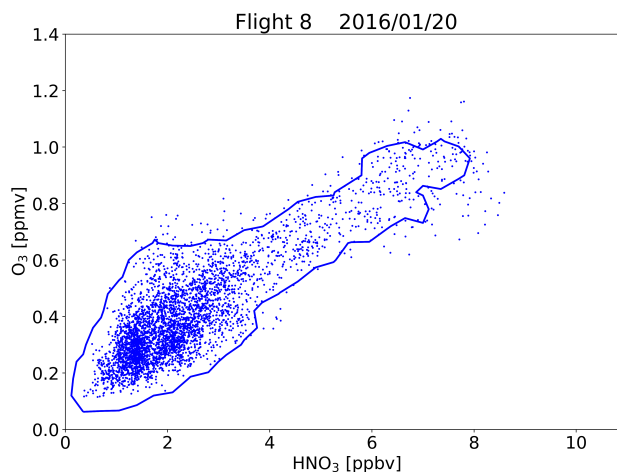
Figure 1. Correlation of \text{HNO}_3 with \text{O}_3 measured by GLORIA during flight 8 on 20 January 2016. The correlation is shown as single points and as RNFD (solid lines).
