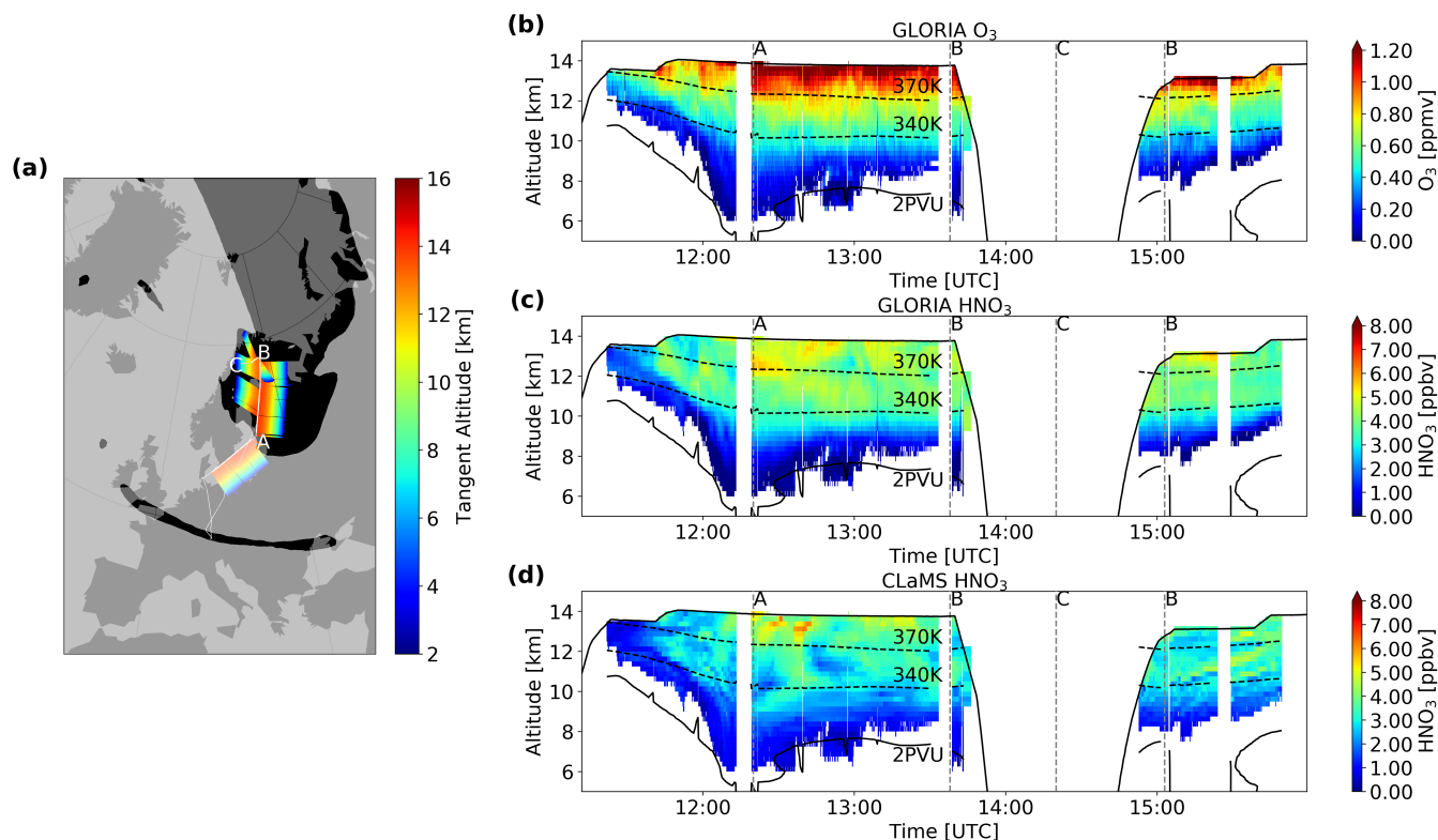
Figure 4. (a) Flight path and vortex filtering according to the Nash criterion at 370 K for flight 21 on 18 March 2016. White line: flight track with characteristic waypoints (A, B, C); dark grey shading: areas that are associated with the polar vortex. Cross-sections of (b) O 3 and (c) HNO 3 distribution derived from GLORIA and (d) HNO 3 distribution simulated by CLaMS for flight 21 on 18 March 2016. Flight altitude (bold black line), characteristic waypoints (A, B, C), 340 K and 370 K potential temperature levels (MERRA-2, dashed black lines) and 2 PVU level (MERRA-2, black line).
