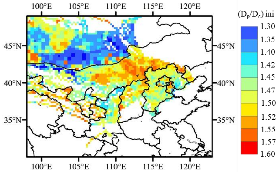
2 Figure S1. The (D_p/D_c)_{ini} of BC particles at emission origins ( 0.25^\circ \times 0.25^\circ ) during the 3 BJNOV2014 campaign period.
