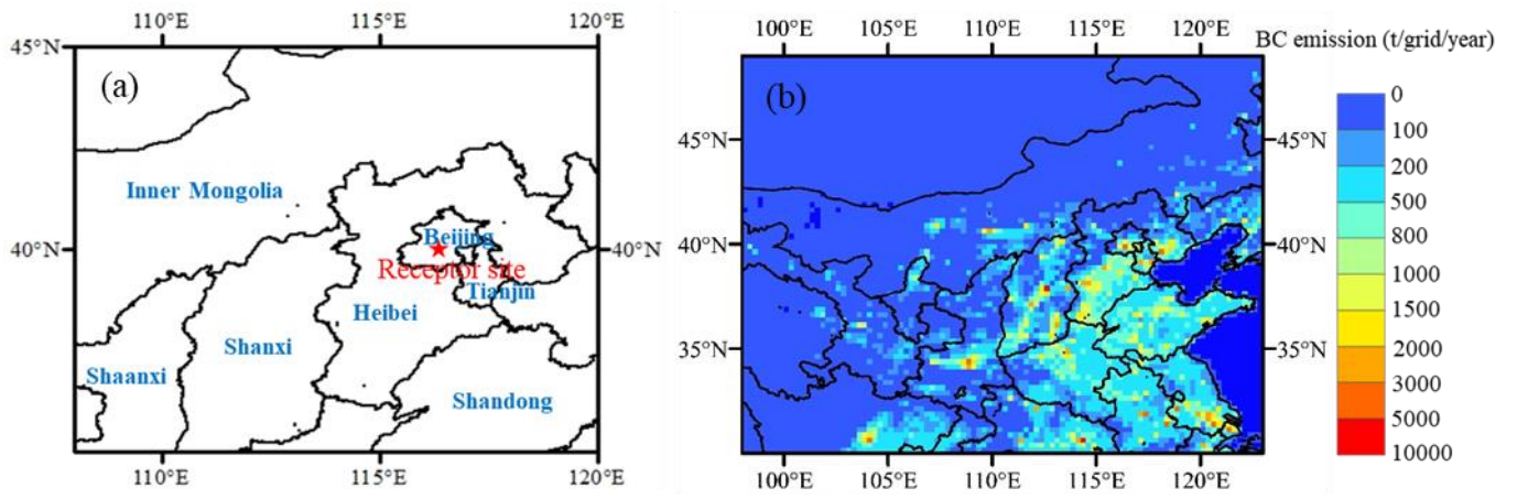
Figure 2. (a) The location of the receptor site (Tsinghua site (40°00'17" N, 116°19'34" E), marked as red star) during the BJNOV2014 measurement period. (b) Spatial distribution (0.25°×0.25°) of BC emission inventory from MIX.
