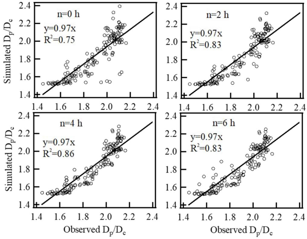
Figure 5. Comparison of the hourly D_p/D_c ratio of BC between the model simulations and observations at our site with different n values in Eq. (15) on 24-30 November 2014 at Tsinghua site. The n values represent the simulated hourly D_p/D_c ratio considering the effects of 0, 2, 4, and 6 hour backward transport using Eq. (15).
