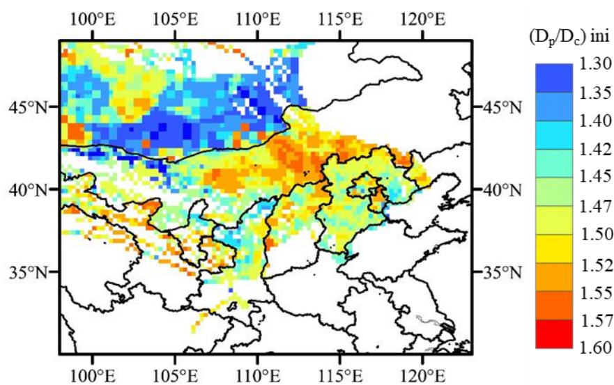
1 2 Figure S1. The (D_p/D_c)_{ini} of BC particles at emission origins ( 0.25^\circ \times 0.25^\circ ) during the BJNOV2014 3 campaign period.
