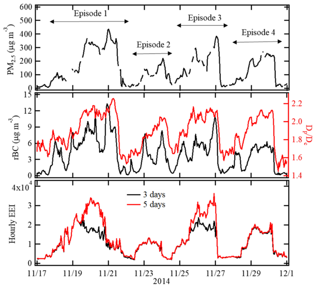
Figure 1. Time series of the PM 2.5 concentration, rBC mass concentration, D_p/D_c ratio of BC-containing particles and the hourly EEI for BC transported to the observation site for 3 and 5 days.
