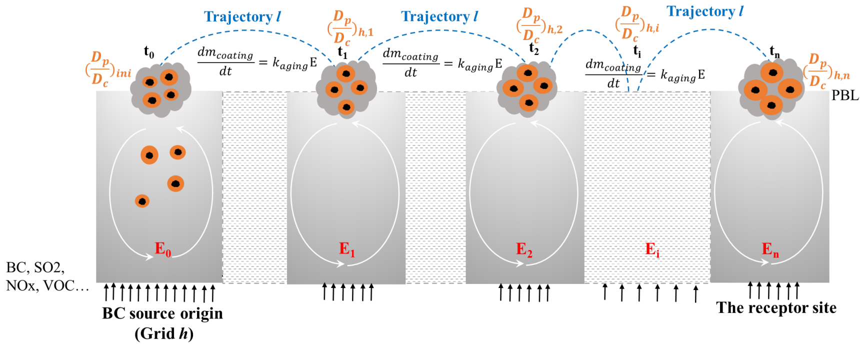
Figure 4. Conceptual scheme of the evolution of the mixing state (i.e., D_p/D_c ratio) of BC from the source origin (i.e., grid h ) to the receptor site following trajectory l .
