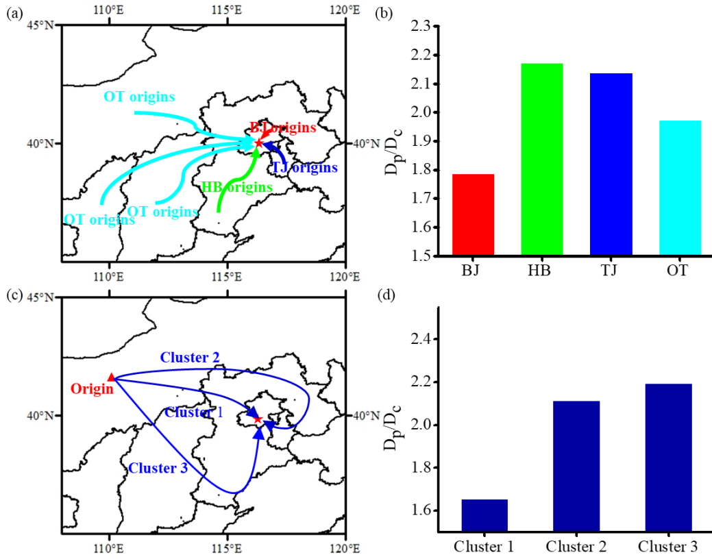
Figure 8. BC aging from emission origins to the receptor site (40°00'17" N, 116°19'34" E; marked with a red star) during the BJNOV2014 measurement period: (a) classification of the BC emission source regions based on political boundaries (i.e., the Beijing source regions (BJ origins), Hebei source regions (HB origins), Tianjin source regions (TJ origins) and other source regions (OT origins)); (b) aging degree (i.e., D_p/D_c ) of BC particles emitted from the four source regions as they are transported to the receptor site; (c) conceptual scheme of trajectories that pass through low emission regions (cluster 1), medium emission regions (cluster 2) and high emission regions (cluster 3) as they transport from clean origins (i.e., Inner Mongolia) to the receptor site; and (d) the degree of aging of BC reaching the receptor site through different trajectories (i.e., Clusters 1, 2 and 3 shown in (c)).
