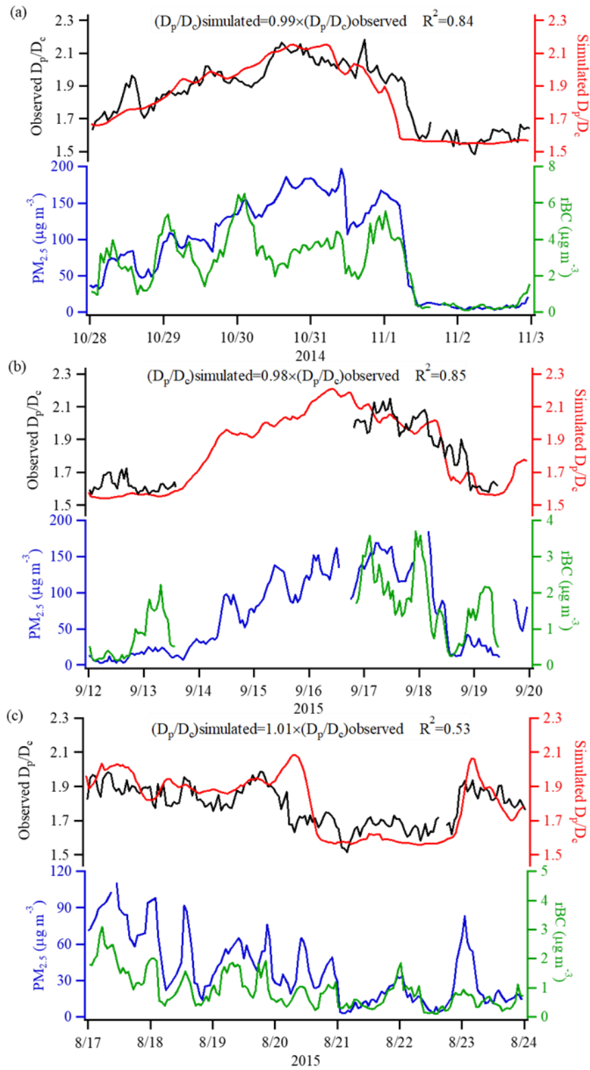
Figure 6. Time series of the observed D_p/D_c ratio, simulated D_p/D_c ratio, and PM_{2.5} and rBC concentrations during the (a) BJOCT2014, (b) BJSEP2015 and (c) BJAUG2015 measurement period.
