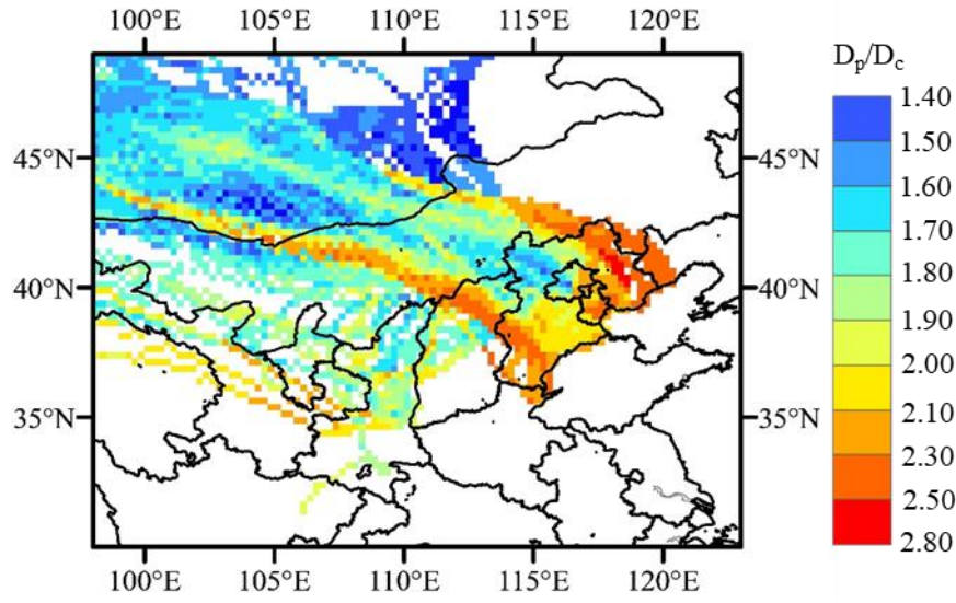
1 2 Figure 7. Aging degree (i.e., D_p/D_c ) of BC particles as they are transported to the receptor site (40°00'17'' N, 116°19'34'' E) 3 from emission origins (0.25°×0.25°) during the BJNOV2014 campaign period. The gridded D_p/D_c ratio was calculated by 4 Eq. (11).
