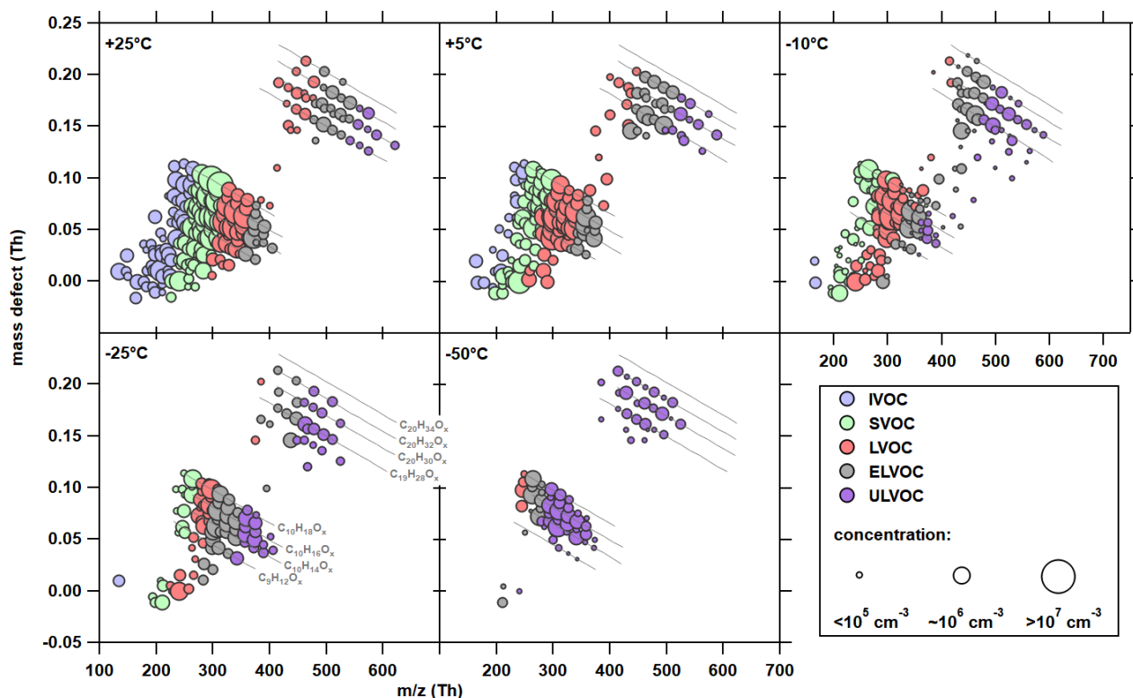
Figure 5: Molecular composition of neutral HOMs at the five temperatures studied and their corresponding volatility.
