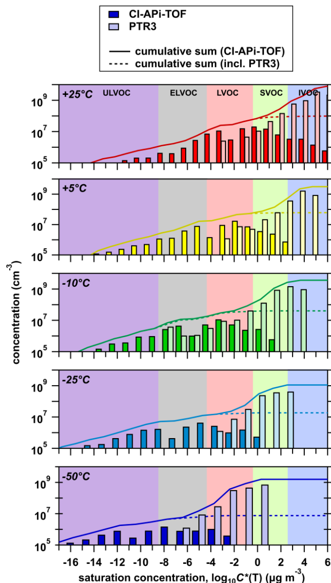
1175 Figure 7: Volatility distribution of the measured oxidation products for five representative temperatures.
