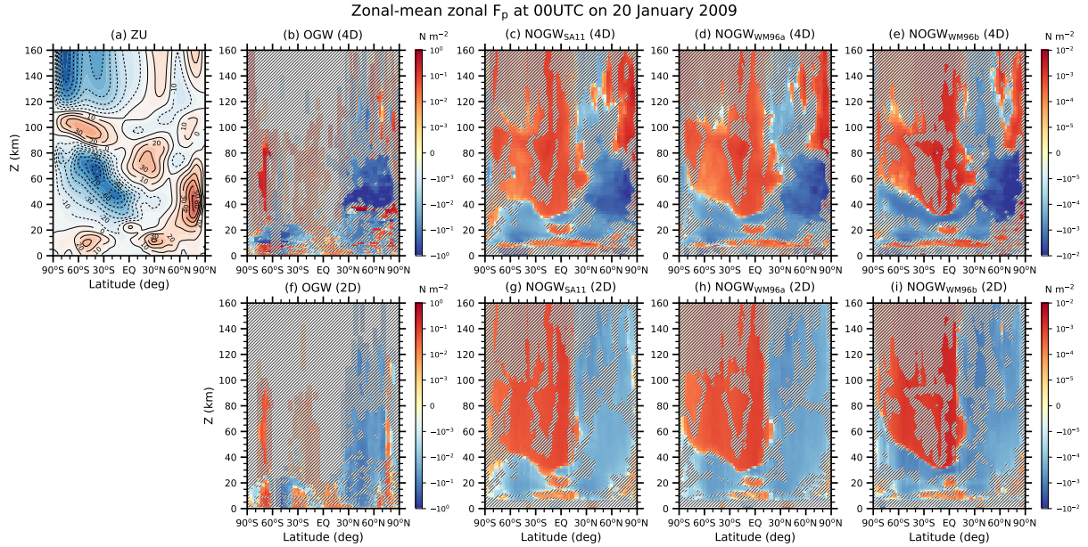
Figure 4. Latitude-height cross-sections of (a) zonal-mean zonal wind (ZU) and (b–i) zonal-mean zonal pseudomomentum fluxes ( F_p s) for OGW and three NOGW-NOGW schemes in the (top) 4D and (bottom) 2D experiments at 00 UTC on 20 January 2009. OGW F_p s are is multiplied by the efficiency factor (0.125). Contour interval of zonal-mean zonal wind is 10 \text{ m s}^{-1} and negative values are plotted in dashed lines. Transparently shaded-Hatched areas on the pseudomomentum fluxes indicate regions where the paired and two-tailed t -test for 20 ensemble members of the 4D and 2D experiments gives p values larger than 0.05 (i.e., no statistical significance at the level of 0.05). Here, the p value means probability that mean values in the 4D and 2D experiments would be similar to each other. The shaded-area-hatched areas are identical in the pair of 4D and 2D experiments for a particular GW scheme. Nonparametric test such as Wilcoxon’s signed rank test, where no probabilistic distribution is assumed, also gives almost similar results as the t -test. For these statistical tests, algorithms presented in Boslaugh (2013) are employed.
