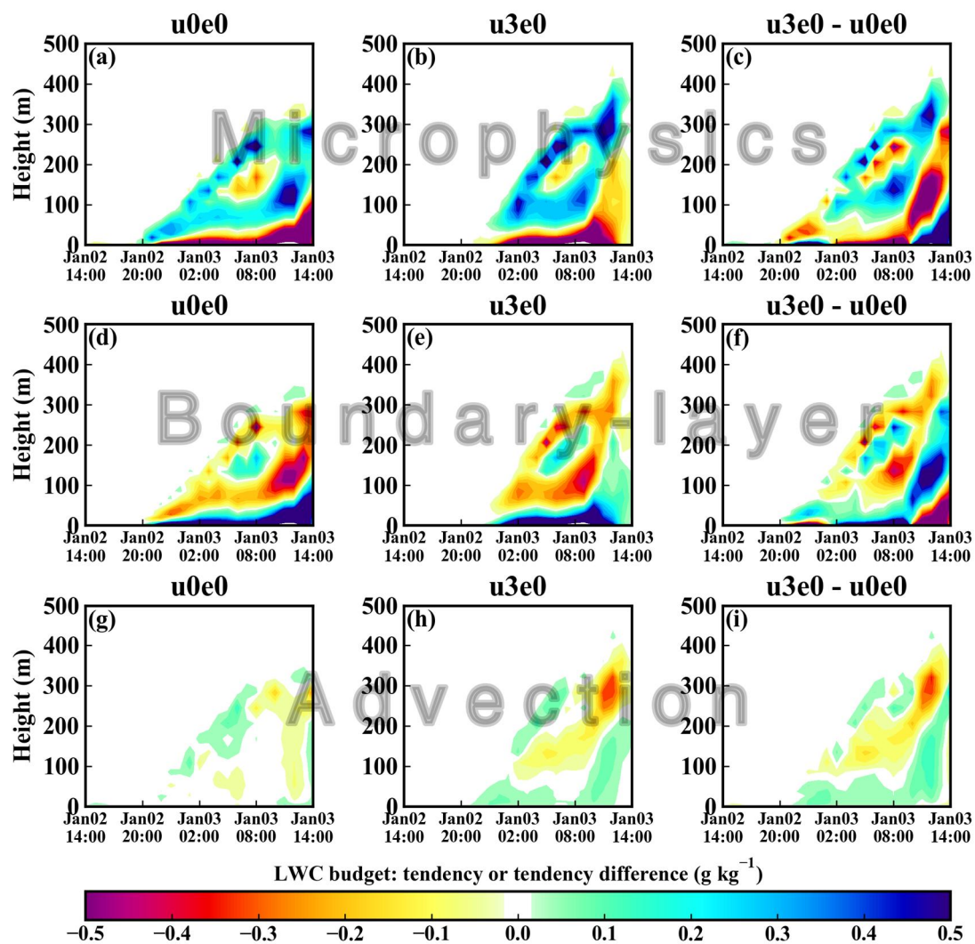
Figure S3. Same as Fig. 10, but for the urbanization effect ( u3e0 minus u0e0 ).
