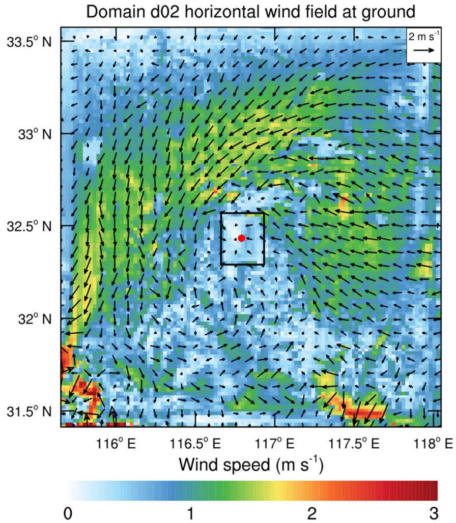
Figure S1. The wind vector (arrows) and wind speed (shaded) in u3e0 at 05:00 03 January. The red dot is SX, and the black box around SX is replaced by urban surface in this experiment. This box shows a wind convergence.
