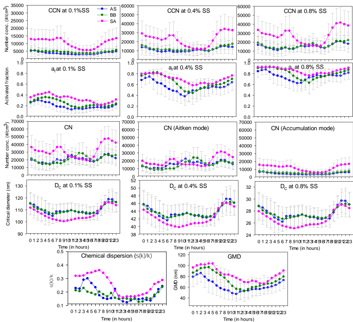
Figure 6: Diurnal variation of (a) N_{CCN} at 0.1%, 0.4%, and 0.8% SS, (b) a_f at 0.1%, 0.4%, and 0.8% SS, (c) N_{CN} , N_{Aitken} and N_{Accumulation} , (d) D_c at 0.1%, 0.4%, and 0.8% SS, (e) Chemical dispersion , and (f) GMD for AS, BB, and SA air masses.
