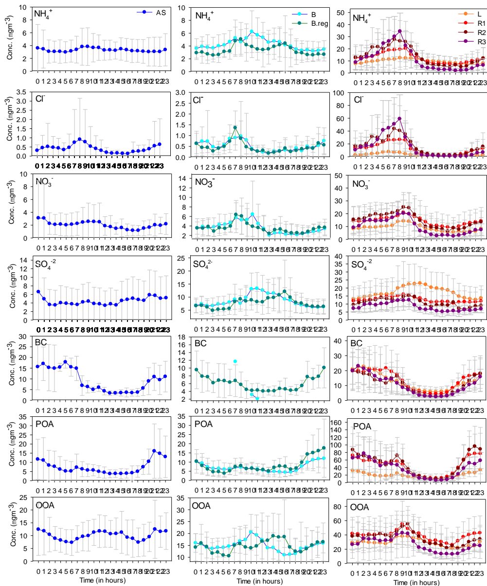
Figure 3: Diurnal variation of NRPM 1 species (NH 4 + , Cl - , NO 3 - , SO 4 2- , POA, and OOA) and BC for AS to the left, BB (B and B.reg) in the middle, and SA ( L , R1 , R2 , and R3 ) air masses to the right.
