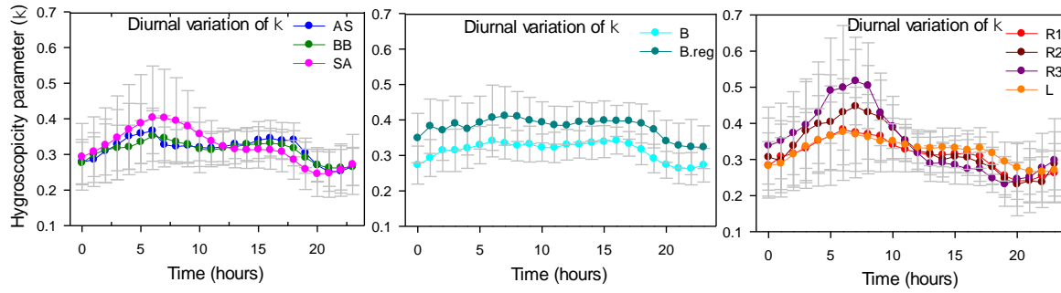
Figure 4: Diurnal variation of \kappa with time. The graph on the left is for AS, BB, and SA, the middle is for BB branches (B and B.reg), and the right is for SA branches (L, R1, R2, and R3).
