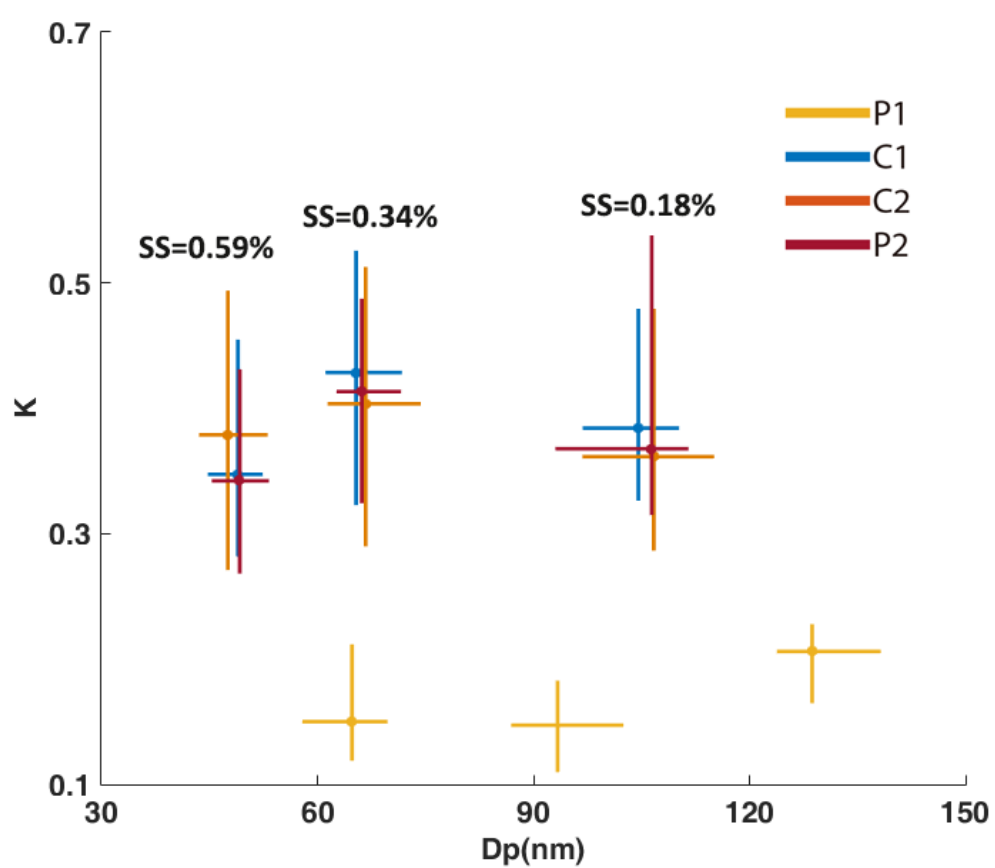
Figure S2. The median and interquartile \kappa value at 0.18%, 0.34% and 0.59% ss during the P1, C1, C2 and P2 periods. Different colors represent different periods.
