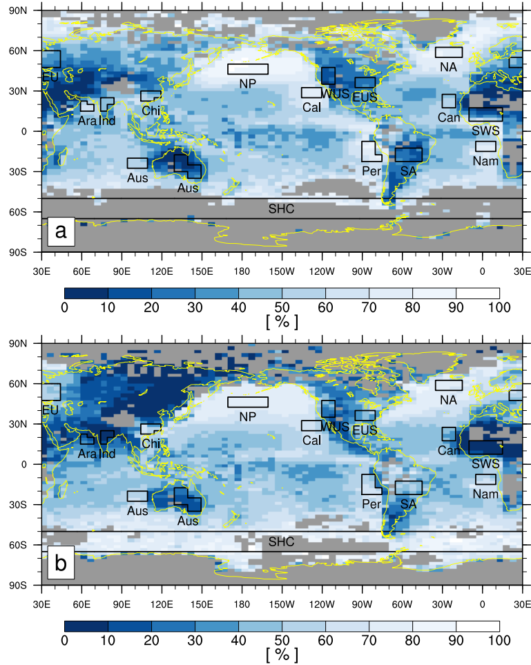
Figure 7. The seasonal climatology of LCA during (a) JJA and (b) DJF in the 2.5^\circ latitude x 5^\circ longitude grid box. The grid boxes with a climatological observation number below 25 in each season are masked by grey color. The domains selected for computing temporal (seasonal-interannual and interannual only) correlation coefficients in Tables 2 and 5 are also plotted: Peruvian [( 7.5^\circ S- 22.5^\circ S, 80^\circ W- 90^\circ W) and ( 17.5^\circ S- 22.5^\circ S, 75^\circ W- 80^\circ W)], Namibian ( 7.5^\circ S- 15^\circ S, 5^\circ W- 10^\circ E), Californian ( 25^\circ N- 32.5^\circ N, 120^\circ W- 135^\circ W), Australian ( 20^\circ S- 27.5^\circ S, 95^\circ E- 110^\circ E), Canarian ( 17.5^\circ N- 27.5^\circ N, 20^\circ W- 30^\circ W), Arabian [( 15^\circ N- 20^\circ N, 60^\circ E- 70^\circ E) and ( 20^\circ N- 22.5^\circ N, 60^\circ E- 65^\circ E)], North Pacific ( 42.5^\circ N- 50^\circ N, 170^\circ E- 200^\circ E), North Atlantic ( 55^\circ N- 62.5^\circ N, 15^\circ W- 35^\circ W), Southern-Hemispheric Circumpolar region ( 50^\circ S- 65^\circ S, 0^\circ E- 360^\circ E), China [( 25^\circ N- 30^\circ N, 105^\circ E- 120^\circ E) and ( 22.5^\circ N- 25^\circ N, 105^\circ E- 115^\circ E)], India [( 20^\circ N- 25^\circ N, 75^\circ E- 85^\circ E) and ( 15^\circ N- 20^\circ N, 75^\circ E- 80^\circ E)], Europe [( 47.5^\circ N- 60^\circ N, 30^\circ E- 45^\circ E) and ( 47.5^\circ N- 55^\circ N, 20^\circ E- 30^\circ E)], Eastern US ( 32.5^\circ N- 40^\circ N, 80^\circ W- 95^\circ W), Western US ( 35^\circ N- 47.5^\circ N, 110^\circ W- 120^\circ W), South America ( 12.5^\circ S- 22.5^\circ S, 45^\circ W- 65^\circ W), Australia [( 25^\circ S- 35^\circ S, 140^\circ E- 150^\circ E) and ( 17.5^\circ S- 30^\circ S, 130^\circ E- 140^\circ E)], and Southwest Sahara ( 7.5^\circ N- 17.5^\circ N, 10^\circ W- 15^\circ E).
