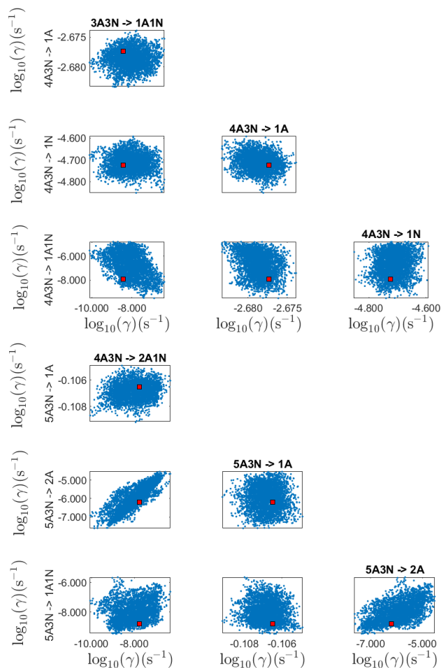
Figure C6. Pairwise marginal posterior distributions (for parameter indexes ranging from 17 to 24) of the base 10 logarithm of the evaporation rates (units given in \text{s}^{-1} ) from time-dependent measurements of the cluster concentrations with time resolution comprising 1.5 minutes at the temperature 278 K. Red rectangles denote the baseline values from Olenius et al. (2013b) used to generate the synthetic data. The notation xAyN corresponds to a cluster with x sulfuric acid and y ammonia molecules.
