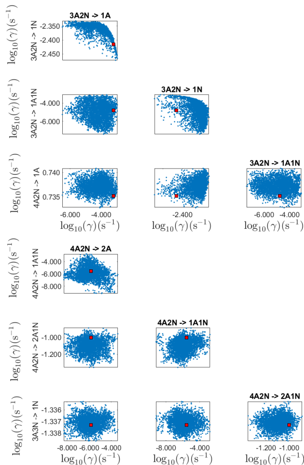
Figure C5. Pairwise marginal posterior distributions (for parameter indexes ranging from 9 to 16) of the base 10 logarithm of the evaporation rates (units given in \text{s}^{-1} ) determined from time-dependent measurements of the cluster concentrations with time resolution comprising 1.5 minutes at the temperature 278 K. Red rectangles denote the baseline values from Olenius et al. (2013b) used to generate the synthetic data. The notation xAyN corresponds to a cluster with x sulfuric acid and y ammonia molecules.
