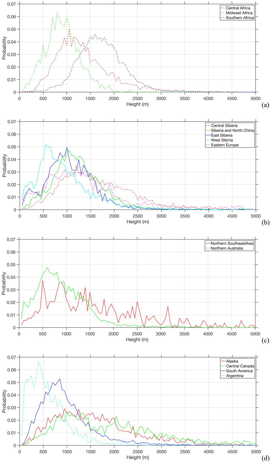
Figure 2: PDFs of all daily MISR plume height measurements from January 2008 through June 2011 (which are 5000m or less) over each of the following geographic regions: (a) Africa, (b) Eurasian High Latitudes, (c) Tropical Asia, and (d) the Americas. Solid lines correspond to regions which have a successful regression model, while dashed lines are regions which do not.
