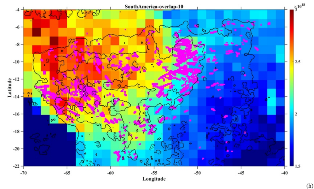
Figure 5: Spatial distribution of annual fires (magenta dots), mean NO 2 column loading on days where there are fires (black isopleths [ \times 10^{15} mol/cm 2 ]), and mean CO column loading on days where there are fires (Colorbar, mol/cm 2 ). The corresponding regions are: (a) 2010 Central Canada, (b) 2010 East Europe, (c) 2009 and (d) 2010 Northern Southeast Asia, (e) 2010 East Siberia, (f) 2008 and (g) 2011 Siberia and Northern China, and (h) 2010 South America.
