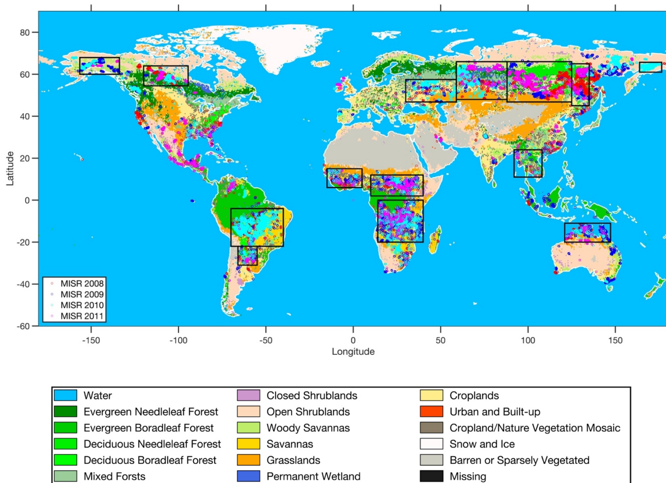
950 Figure 1: Land surface type at each of the daily MISR measurements from January 2008 to June 2011. Each dot corresponds to an individual aerosol plume, with different colors representing different years.
