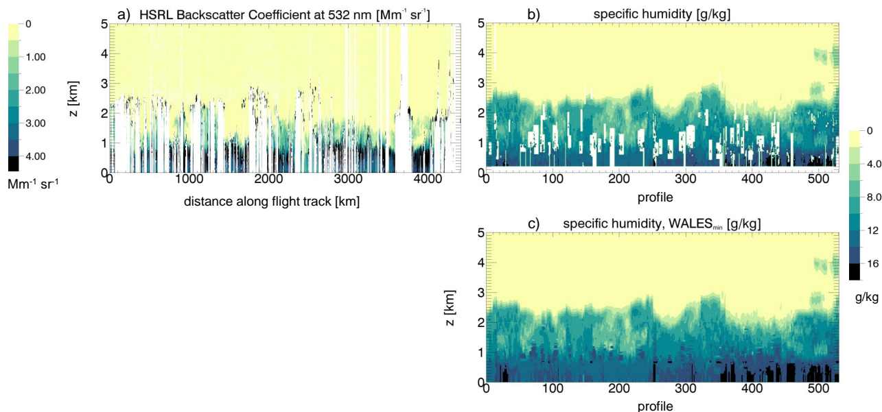
Figure 1. Lidar profiles of the flight on 11. December 2013: (a) atmospheric backscatter for the full flight, and (b,c) specific humidity for those 531 profiles where more than 50 % of the lidar data within the cloud layer and below are available. The remaining gaps in the original data set in (b) are filled by assuming saturation in clouds, and by nearest neighbor values elsewhere, resulting in a gap-filled representation in (c). See text for details. Note that the aspect ratio is 1:500 in (a) and 1:150 in (b) and (c).
