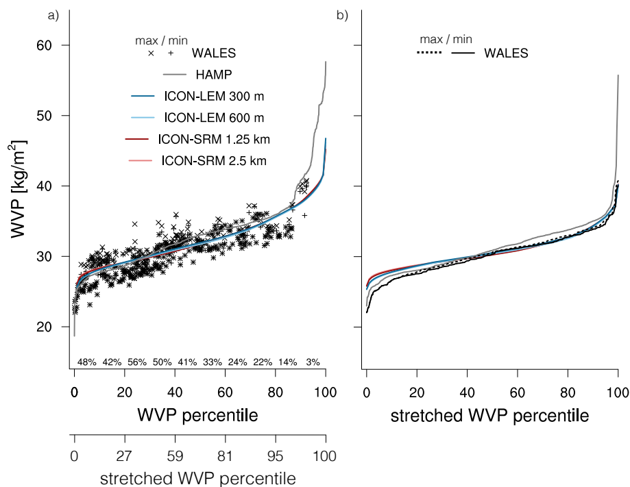
Figure 4. Water vapor path (WVP) on 11th of December 2013 in WVP space. (a) ICON simulations and HAMP observations of WVP are sorted by each one's WVP values. WALES data is plotted as co-located with HAMP. Percentages above the x axis tell how many valid WALES measurements have been obtained in each 10 % interval of HAMP's WVP space. (b) ICON results and HAMP data is randomly selected according to those percentages in each 10 % interval resulting in a stretched WVP space, which is also shown as an additional x axis in (a). In (b) WALES data is sorted by its own WVP instead of being co-located with HAMP. Further details are discussed in the text.
