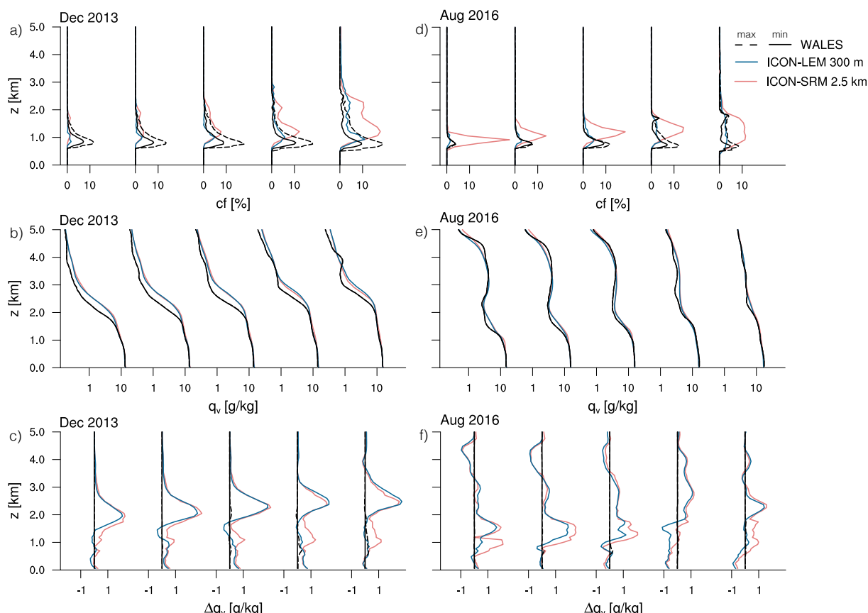
Figure 9. Profiles of (a,d) cloud fraction, (b,e) water vapor and (c,f) the difference to water vapor WALE_{S_{min}} for flight composites (a-c) December 2013 and (d-f) August 2016. Each profile shows the mean for a 20-percentile range of WVP in stretched moisture space from driest profiles on the left to moistest profiles on the right (see Fig. 7).
