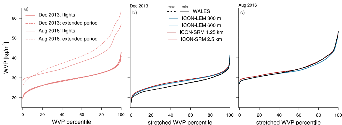
Figure 7. WVP as a function of WVP percentiles (a) for ICON-SRM 2.5 km and the flight period and domain in December 2013 and August 2016 (see Table 1) as well as for an extended period that includes a longer time period for a domain with mean borders (see text for details); (b) for the flight composite in December 2013; and (c) for the flight composite in August 2016.
