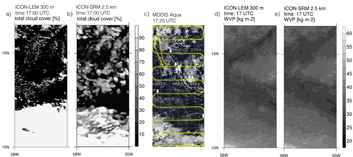
Figure 2. Cloud cover and water vapor path (WVP) in the flight domain on 11 December 2013. Cloud cover at 17:00 UTC from (a) ICON-LEM 300 m and (b) ICON-SRM 2.5 km; (c) MODIS Aqua corrected reflectance at 17:25 UTC overlaid with the flight path which was flown from north to south; WVP at 17:00 UTC from (d) ICON-LEM 300 m and (e) ICON-SRM 2.5 km.
