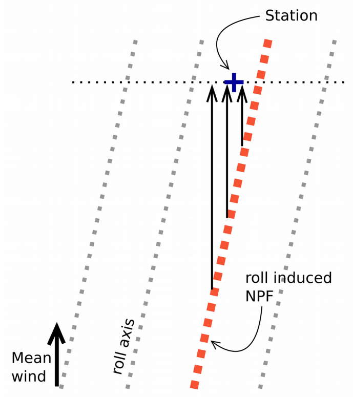
410 Figure 7: Schematic diagram illustrating how a difference in the direction of the mean wind and the roll axis causes the rolls (and the roll-induced NPF) to move over a stationary point perpendicular to the mean wind direction.
