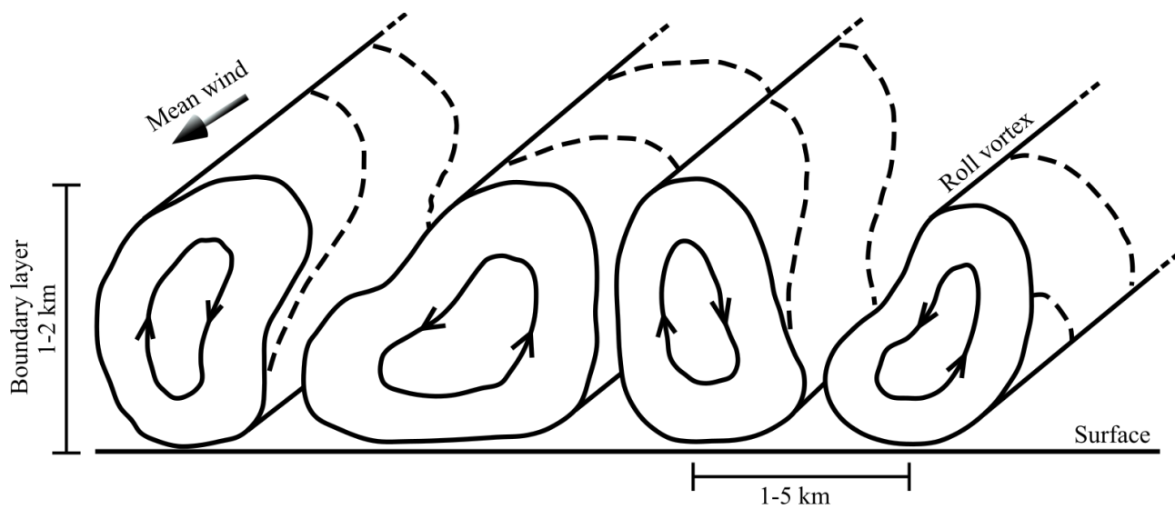
385 Figure 1: A schematic drawing of roll vortices in the boundary layer.
