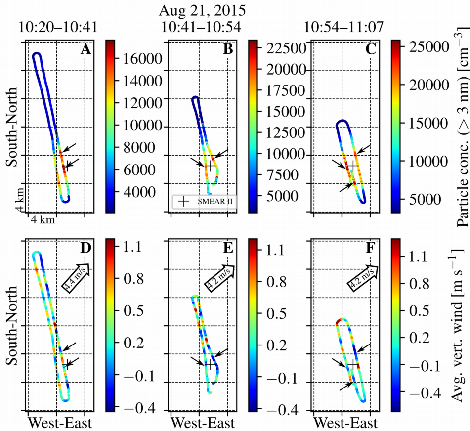
395 Figure 5: In panels A-C the sections of the measurement airplane's flight track are colored by >3 \text{ nm} particle number concentration. The grids have a 4-by-4 km spacing, the plus sign marks the position of the SMEAR II station and the time intervals for the flight track sections are displayed on top of the panels. In panels D-F the same flight tracks are colored by vertical wind speed smoothed using 30-sec 400 moving average. The positive sign refers to updraft and the negative sign to downdraft. The large arrows show the mean wind speed and direction measured on board the airplane. The flight tracks were flown inside the convective BL between 120 m and 620 m above ground. The small arrows show that the maxima in the particle number concentration were located in the roll downdrafts.
