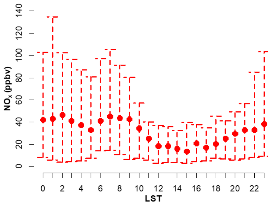
RC 8 Diurnal variation of NO x during the entire measurement period
