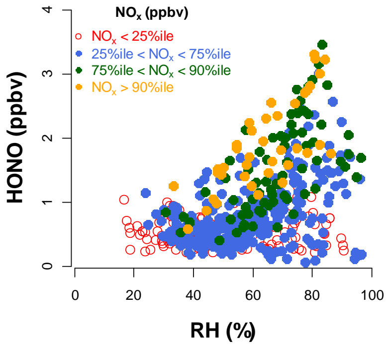
RC 4 The relationship between HONO and RH color-coded by NO x concentrations.
