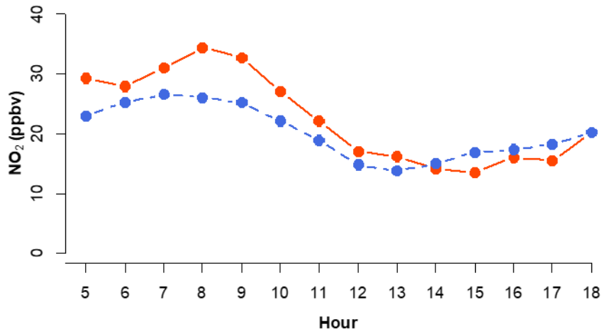
RC 2 Diurnal variation of NO 2 in high O 3 episodes (red) and non-episode (blue).
