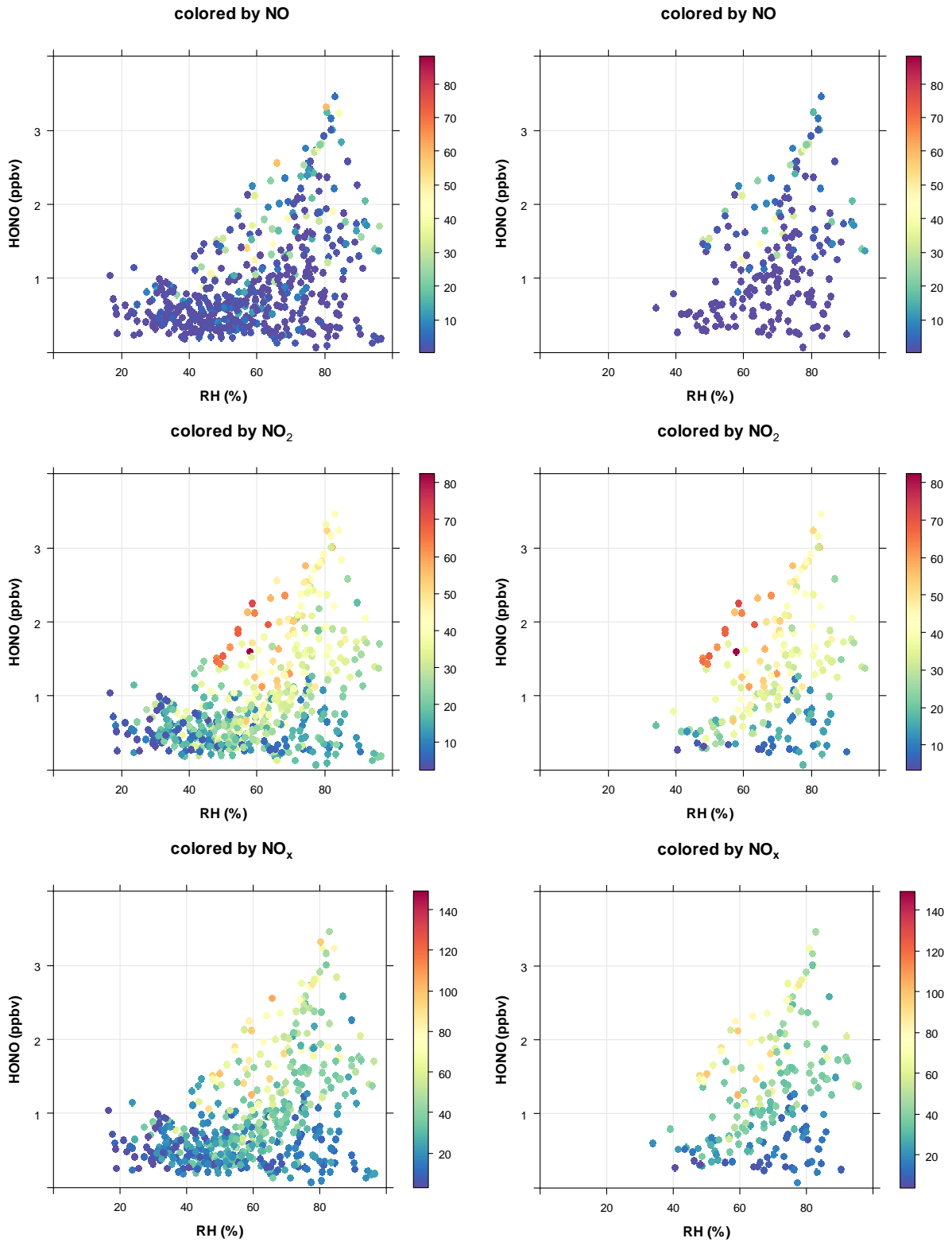
RC 3 The relationship of HONO with relative humidity (RH) color-coded by NO, NO 2 , and NO x concentrations during the entire period (left) and nighttime (right, 19–05 LST only).
