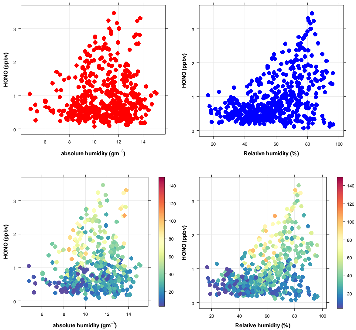
RC 7 The relationship of HONO with absolute humidity (AH) and relative humidity (RH) color-coded by NO x concentration.
