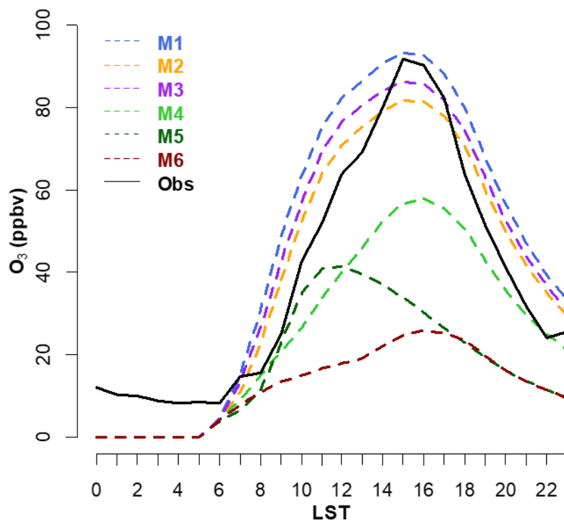
RC 5 The diurnal variation of O 3 simulated by F0AM model.
