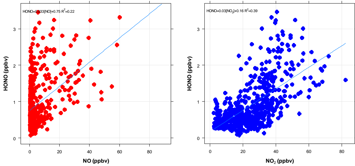
RC 1 A correlation of HONO with NO (red) and NO 2 (blue).
