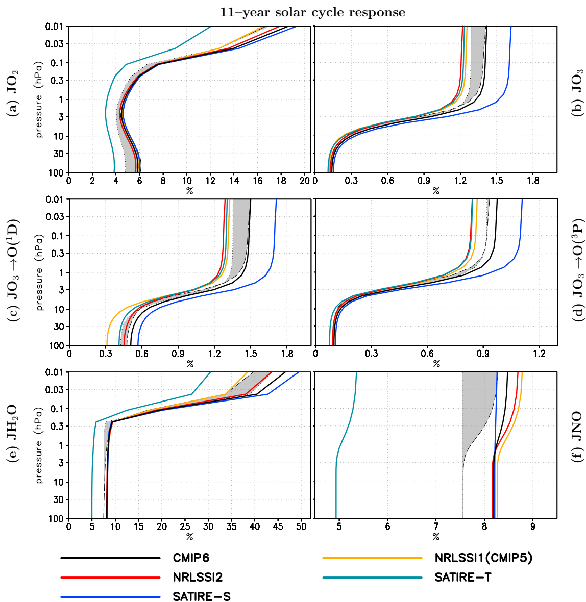
Figure 3. Percentage change of the photolysis rates from solar minimum to maximum of (a) oxygen ( \text{JO}_2 ), (b) ozone ( \text{JO}_3 = \text{JO}_3 \rightarrow \text{O}(^1\text{D}) + \text{JO}_3 \rightarrow \text{O}(^3\text{P}) ), (c) \text{O}_3 producing \text{O}(^1\text{D}) ( \text{JO}_3 \rightarrow \text{O}(^1\text{D}) ), (d) \text{O}_3 producing \text{O}(^3\text{P}) ( \text{JO}_3 \rightarrow \text{O}(^3\text{P}) ), (e) water vapour ( \text{JH}_2\text{O} ), and (f) nitric oxide ( \text{JNO} ) for a single time step at 180^\circ\text{E} averaged from 60^\circ\text{S} to 60^\circ\text{N} . Changes are derived for an average of WACCM and EMAC simulations using five SSI data sets at solar maximum NRLSSI1(CMIP5) (yellow), NRLSSI2 (red), SATIRE-S (blue), SATIRE-T (dark blue), and CMIP6 (black) relative to the average of the WACCM and EMAC reference solar minimum simulations. The shaded area indicates the range of the WACCM (black long dash contour) and EMAC (black dotted contour) ensemble means.
