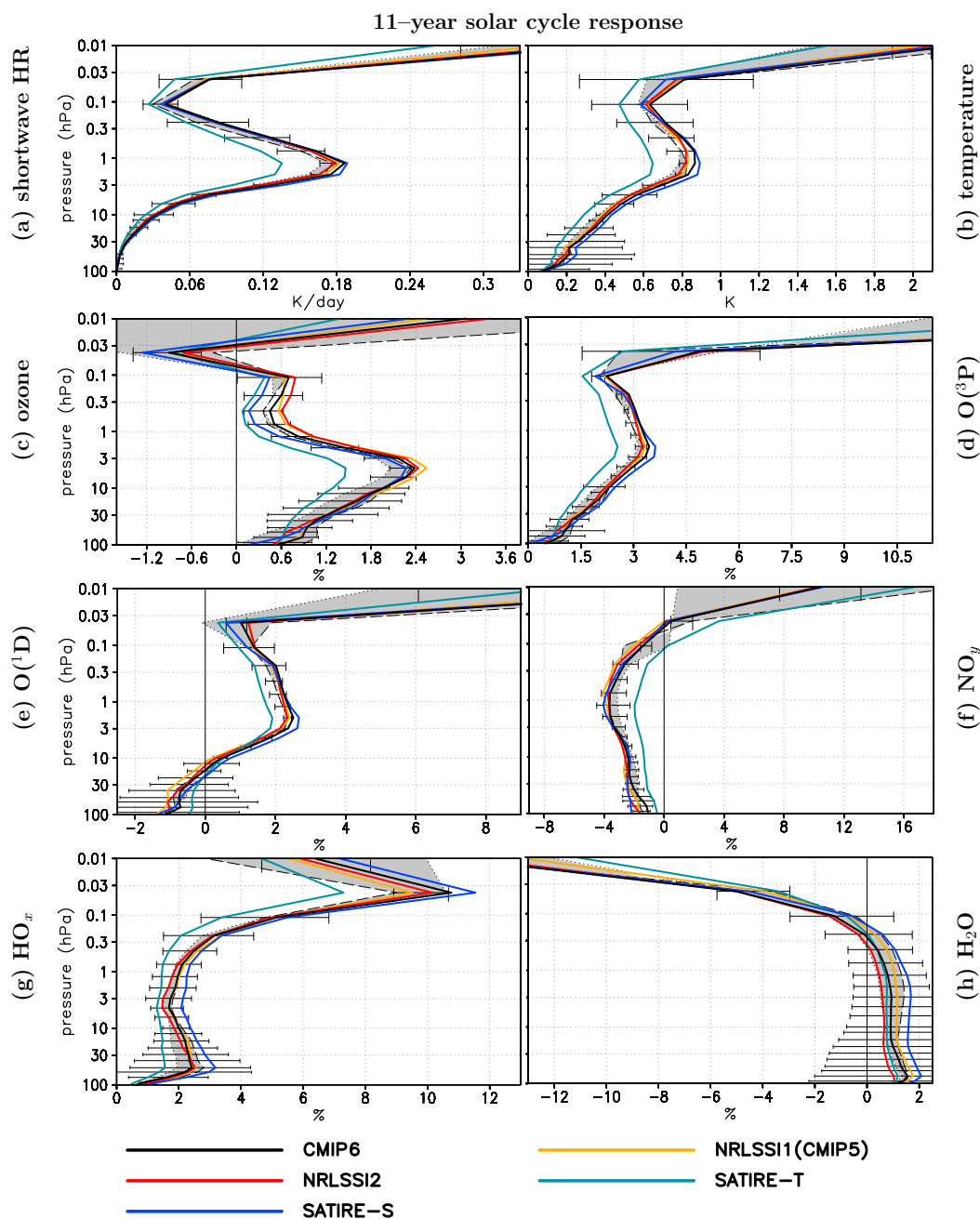
Figure 2. Annual mean 11-year solar cycle response ( 60^{\circ}\text{S} – 60^{\circ}\text{N} ) in (a) shortwave heating rates, (b) temperature, (c) ozone concentrations, (d) atomic oxygen ( \text{O}(^3\text{P}) ), (e) atomic oxygen ( \text{O}(^1\text{D}) ), (f) \text{NO}_y , (g) \text{HO}_x , and (h) \text{H}_2\text{O} . Solar responses are derived for an average of WACCM and EMAC simulations using five SSI data sets at solar maximum NRLSSI1(CMIP5) (yellow), NRLSSI2 (red), SATIRE-S (blue), SATIRE-T (dark blue), and CMIP6 (black) relative to the average of the WACCM and EMAC reference solar minimum simulations. The shaded area indicates the range of the WACCM (black long dash contour) and EMAC (black dotted contour) ensemble means. The 95% uncertainty error bar is given for the model average using the CMIP6 data set, calculated with a Student’s t test.
