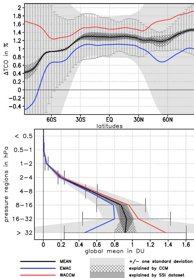
Figure 8. Top: Ensemble average, annual and zonal mean 11-year solar cycle response in partial column ozone in % (solid black) and the 95% confidence interval as error bars; WACCM simulations only (solid red); EMAC simulations only (solid blue); light grey shading denotes the standard deviation of the ensemble mean solar response; hatched region denotes the part of the standard deviation explained by the models; dark shading denotes the part of the standard deviation explained by the SSI data sets. Bottom: As top for annual, global mean 11-year solar cycle response in TCO in DU (solid black) for pressure regions as indicated on the y-axis.
