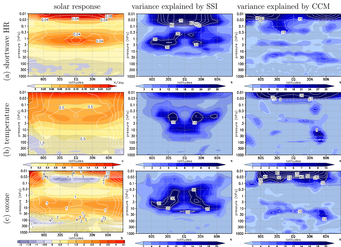
Figure 1. Left column: Annual mean 11-year solar cycle response (shaded) and signal variance (white contours) in terms of the solar response annual standard deviation for shortwave heating-rates (top), temperature (middle), and ozone mixing ratios (bottom). Solar signal derived as ensemble mean over both models and all SSI data sets; solar minimum SSI based on ATLAS3 reference state. Middle column: Percentage of signal variance (square of white contours of left figures) explained by systematic differences between forcing data sets (blue shading). The white contours indicate levels of explained variance larger than the range of shading. Right column: as middle column but for systematic differences between CCMs. The grey hatching masks areas where signal or ratio of explained variance does not pass a test for statistical significance ( p > 5\% ).
