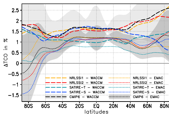
Figure 6. Annual mean zonally averaged 11-year solar cycle response in total column ozone (TCO) in % for WACCM (long dashed) and EMAC (dotted) for prescribed SSI data sets NRLSSI1(CMIP5) (yellow), NRLSSI2 (red), SATIRE-S (blue), SATIRE-T (light blue), and CMIP6 (black). The 95% uncertainty range is given for simulations with the CMIP6 data set for WACCM (light grey shaded) and EMAC (dark grey shaded).
