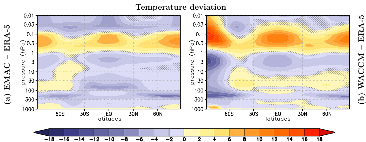
Figure 4. Annual mean temperature deviation of EMAC and WACCM to ERA-5 climatology. (a) EMAC – ERA-5 and (b) WACCM – ERA-5 climatology. The ensemble mean for each CCM consists of the solar minimum reference simulation (included 5 times in the ensemble mean) and the 5 simulations of the solar maximum. The ERA-5 data consists of annual mean data from 1982 to 2018. Grey hatching masks areas where differences does not pass a test for statistical significance ( p > 5\% ), for differences relative to ERA-5.
