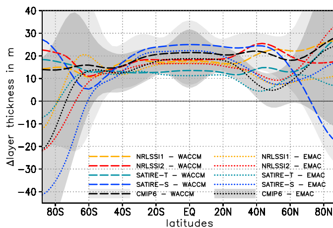
Figure 7. Annual mean zonally averaged 11-year solar cycle response in layer thickness from 100 to 10 hPa in m for WACCM (long dashed) and EMAC (dotted) with prescribed SSI data sets NRLSSI1(CMIP5) (yellow), NRLSSI2 (red), SATIRE-S (blue), SATIRE-T (light blue), and CMIP6 (black). The 95% uncertainty range is given for simulations with the CMIP6 data set for WACCM (light grey shaded) and EMAC (dark grey shaded).
