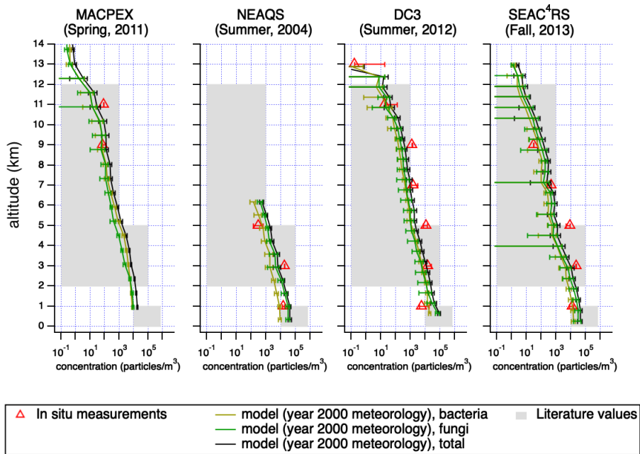
Figure 1: Flight tracks (A) and altitude-resolved concentrations of particles categorized as bioaerosol (B) during four aircraft studies: MACPEX, NEAQS, DC3 and SEAC 4 RS. The PALMS size range is 0.3 – 2 \mu\text{m} for MACPEX and 0.3 – 4 \mu\text{m} for all other campaigns. Note there was no MACPEX data for altitudes less than 2 km. The error bars on PALMS data correspond to particle type assignment confidence estimated using laboratory data and SVM algorithm. Results are shown for the GLOMAP model using year 2000 meteorology sampled at the measurement locations. Error bars on model results correspond to standard deviations in the model estimates in each altitude bin. Concentrations for both model and PALMS measurements are reported in particles per ambient \text{m}^3 . Typical literature values are estimated using Burrows, et al (2009) for surface values (< 1 km), Twohy, et al (2016) and Bowers, et al (2012) for 2 km – 5 km and Twohy, et al (2016) for 5 km – 12 km.
