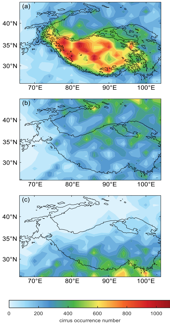
395 Figure 1: Distribution of cirrus occurrence numbers during the June-August period from 2012 - 2016. The cirrus top height is (a) below 9 km, (b) 9 - 12 km (c) above 12 km. In (a), the inner and outer black curves represent the topographic height of 4500 m and 3000 m, respectively. In (b) and (c), the black curves represent the topographic height of 3000 m.
