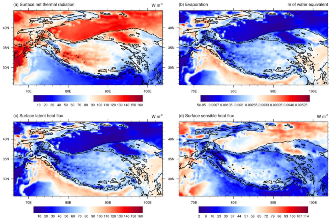
400 Figure 2: Geographical distribution of monthly mean surface (a) radiation cooling, (b) surface evaporation (c) latent heat flux, and (d) sensible heat flux over Tibetan Plateau. The study period is June, July and August from 2012 to 2016.
