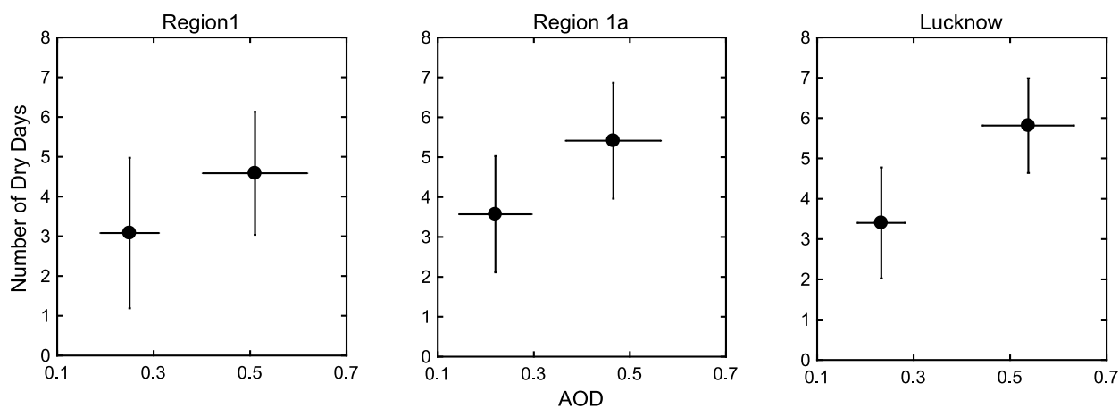
Figure 5. Sequential association between AOD cluster (16-30 July) and DDF (1-15 August) for Region 1, 1a and Lucknow
