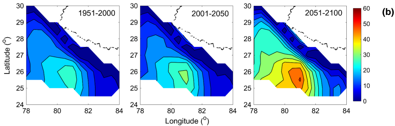
1062 Figure 10. (a) Climatic variations in dry day frequency over Region 1 and 3 containing both historical data (upto 2005) and RCP8.5 projections 1063 (2006-2100) of multi model mean from 3 selected GCMs (b) Projected lat-lon maps of DDF for all three 50 year periods from 1951-2100.
