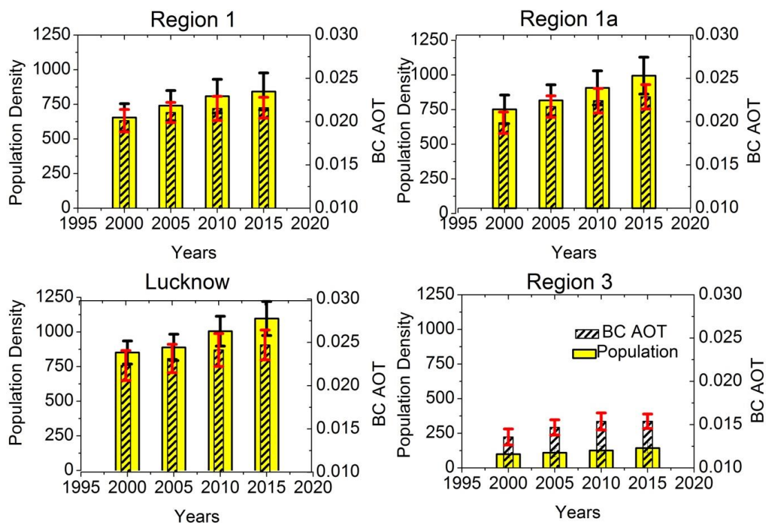
Figure 9. Region-wise population densities and BC AOT values (during August) for Region 1, 1a, Lucknow and Region 3 during (2000-2015), vertical bars represent the corresponding 1 sigma standard deviations values.
