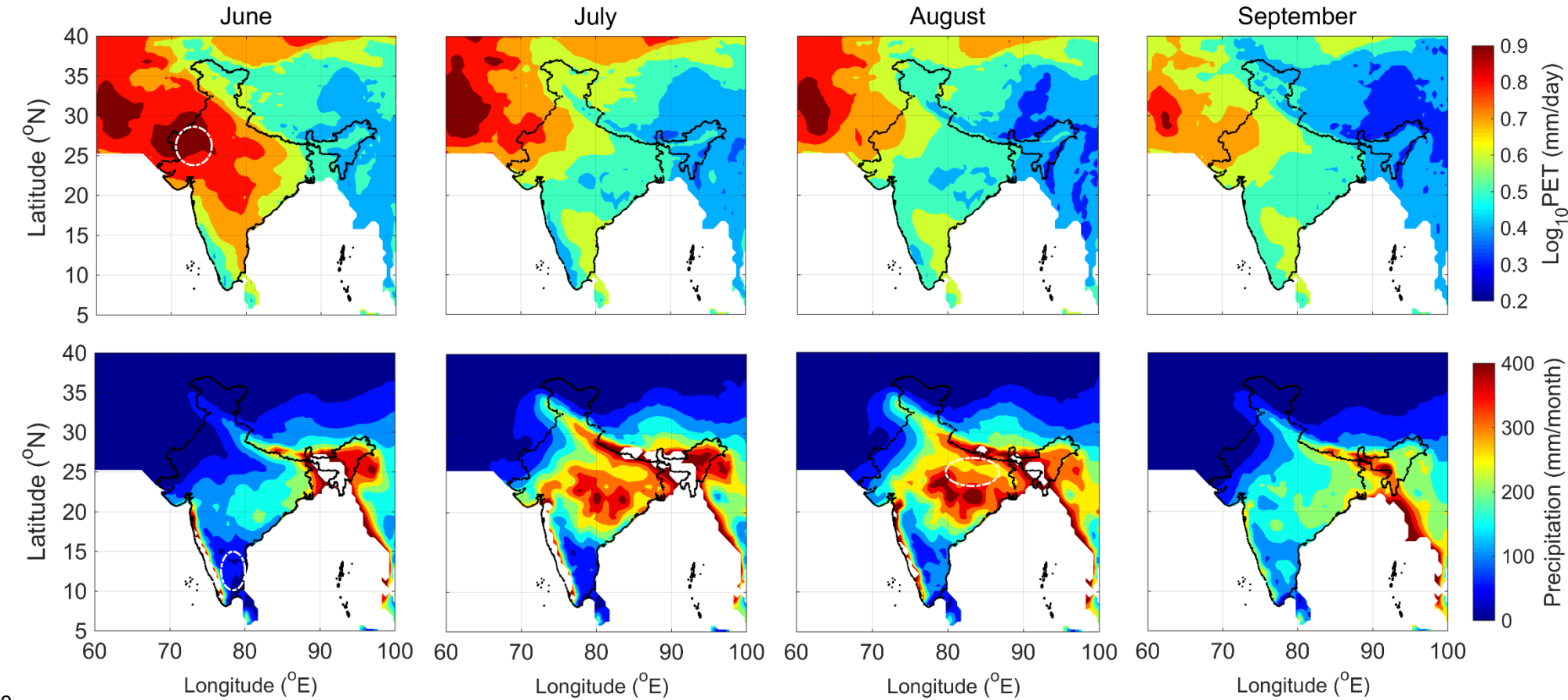
955 Figure 1. Monthly averaged maps of potential evapo-transpiration rate and precipitation during June-September.
