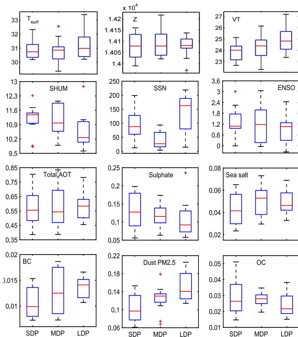
Figure 7. Frequency distribution analysis results of various controlling factors behind DDF evolution for various types of dry phase lengths over region 3, namely: Surface temperature, Geopotential, VT, Humidity, SSN, ENSO, Total aerosols, Sulphates, Sea Salt, BC, Dust PM 2.5 and OC.
