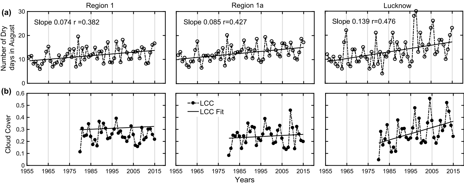
1011 Figure 6. Statistical comparison of the climatology of all parameters during August for region 1, region 1a, Lucknow during various time spans 1012 (a) Dry Day Frequency values between 1956-2015 and (b) Low cloud cover during 1980-2015 .
