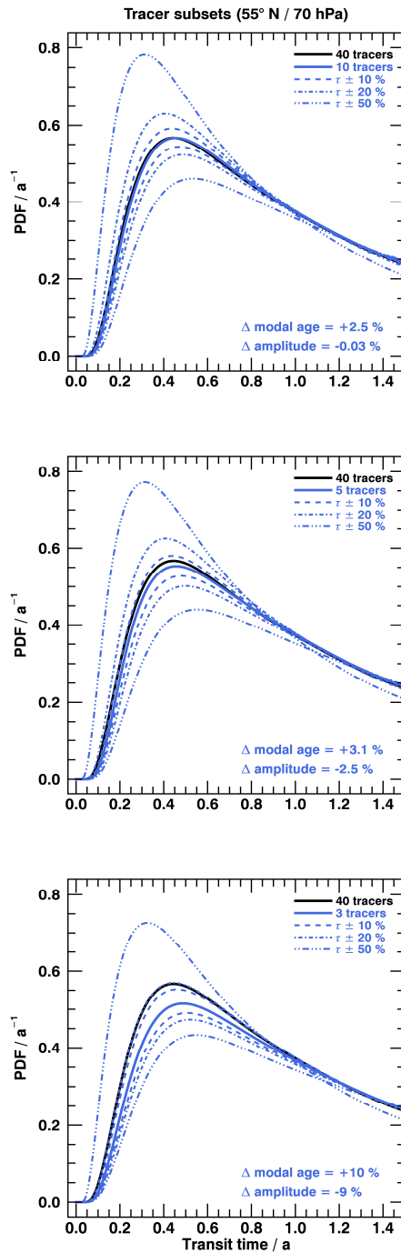
Figure 12: Annual mean age spectra from radioactive tracer subsets compared to full set at 55° N and 70 hPa. Black The black solid line corresponds to the full set (40 tracers), while the solid blue line denotes spectra of a subset with 10 tracers (top), 5 tracers (mid) and 3 tracers (bottom). The changes in modal age and amplitude for the solid blue lines relative to the black lines are given in each panel in the bottom right corner. The three dashed and dash-dotted spectra in each panel include an error in the knowledge of the local chemical lifetimes of \pm 10\% , \pm 20\% and \pm 50\% (see text for details).
