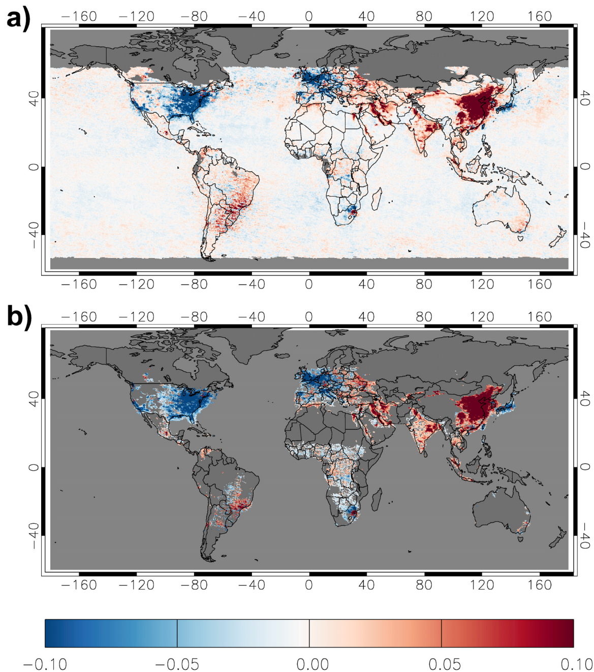
Figure 2: (a) Satellite-based trends of tropospheric NO 2 VCD (in 10^{15} molecules \text{cm}^{-2} \text{yr}^{-1} ) for the period 4/1996-9/2017. Only trends calculated for timeseries with at least 8 months per year are taken into consideration. (b) Same as (a) but for statistically significant trends at the 95% confidence level and for grid cells with a long term tropospheric NO 2 VCD mean of at least 1 \times 10^{15} molecules \text{cm}^{-2} .
