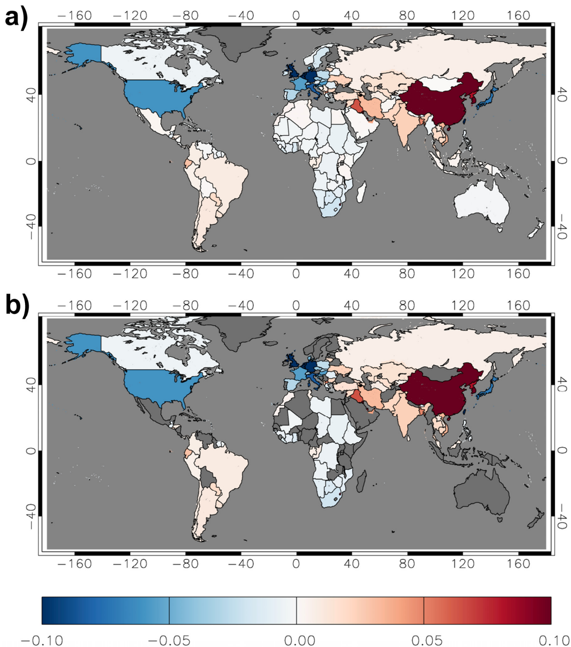
Figure 5: (a) Satellite-based trends of tropospheric NO 2 VCD (in 10^{15} molecules \text{cm}^{-2} \text{yr}^{-1} ) on a country basis for the period 4/1996-9/2017. Only trends calculated for timeseries with at least 8 months per year are taken into consideration. (b) Same as (a) but for statistically significant trends at the 95% confidence level.
