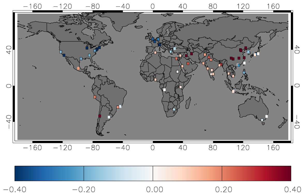
Figure 8: Satellite-based trends of tropospheric NO 2 VCD (in 10^{15} molecules \text{cm}^{-2} \text{yr}^{-1} ) for megacities and large urban agglomerations of the world for the period 4/1996-9/2017. The spots with a statistically significant trend at the 95% confidence level are marked with a black outline.
