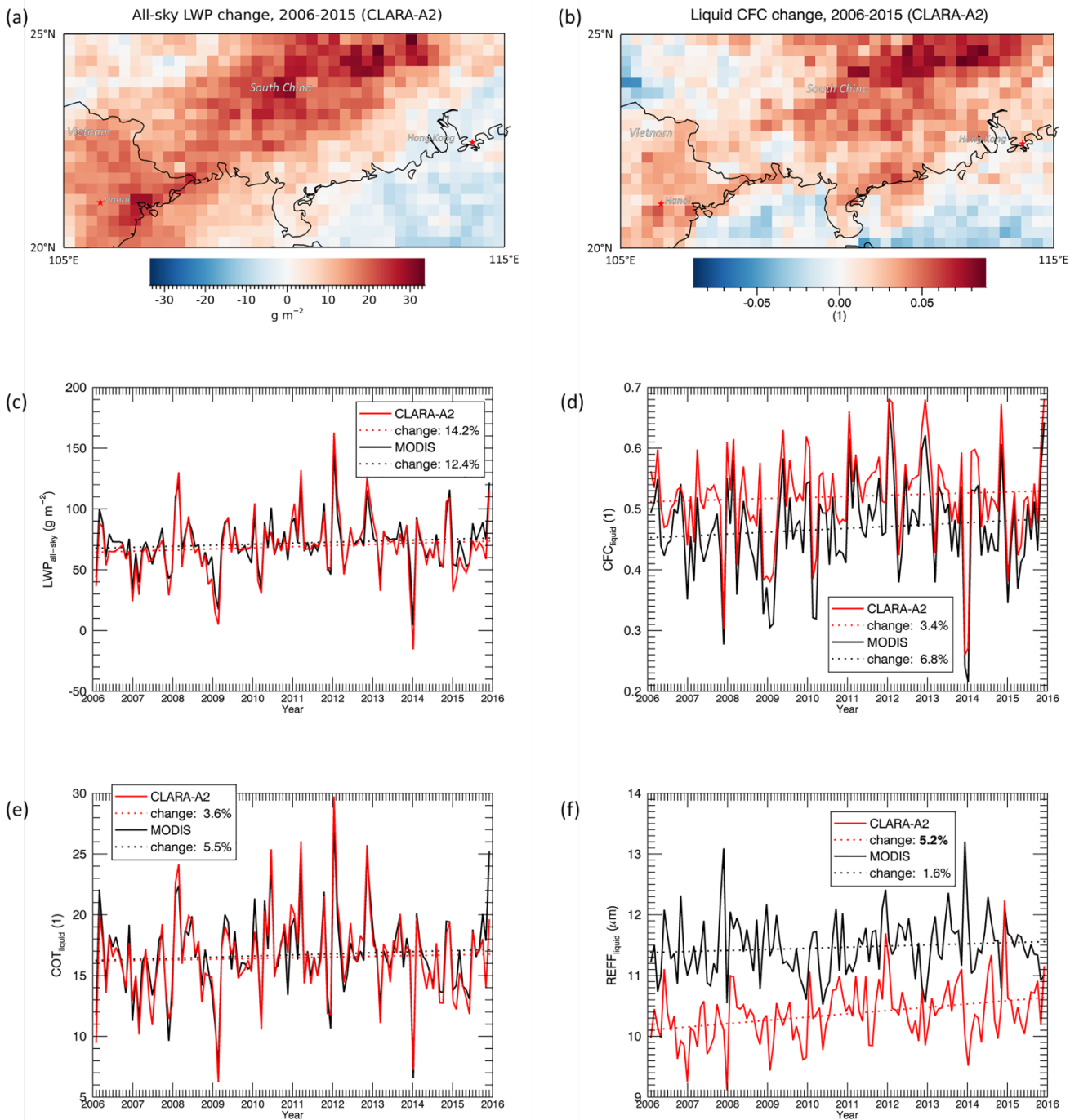
Figure 7. Changes in cloud properties over southern China from 2006 to 2015, based on CLARA-A2 and MODIS data. (a), (b) Spatial distributions of changes in all-sky LWP and liquid CFC based on CLARA-A2 data. Spatially averaged monthly deseasonalized values of all-sky LWP (c), liquid CFC (d), liquid COT (e) and REFF (f). Percent changes during the period examined are also shown, with the statistically significant ones (only CLARA-A2 liquid REFF) indicated in bold.
