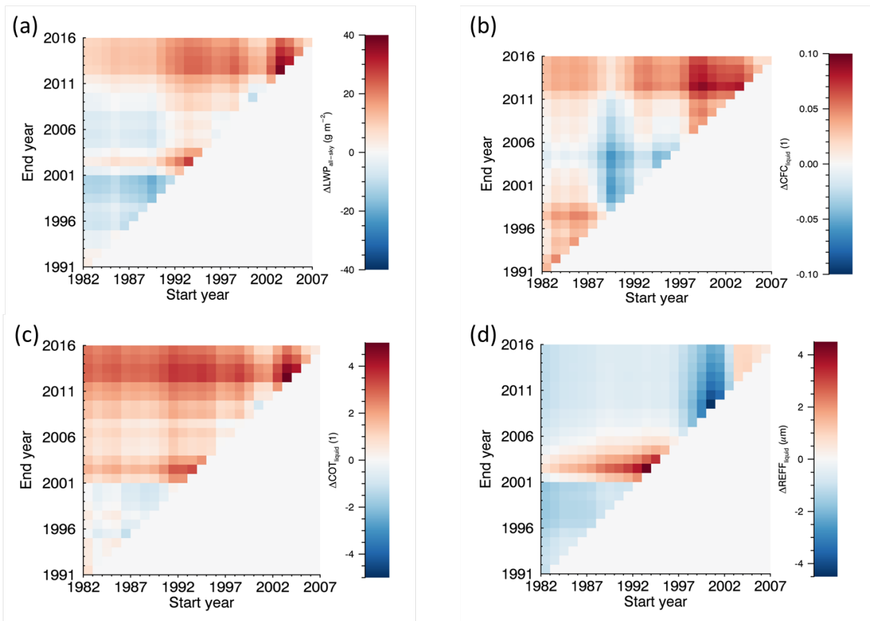
Figure 8. Changes in liquid cloud properties over southern China, based on 34 years of CLARA-A2 data (1982-2015) and estimated for all possible combinations of start and end years, with a minimum time range of 10 years. The four plots show corresponding changes in (a) all-sky LWP, (b) liquid CFC, (c) liquid COT and (d) liquid REFF.
