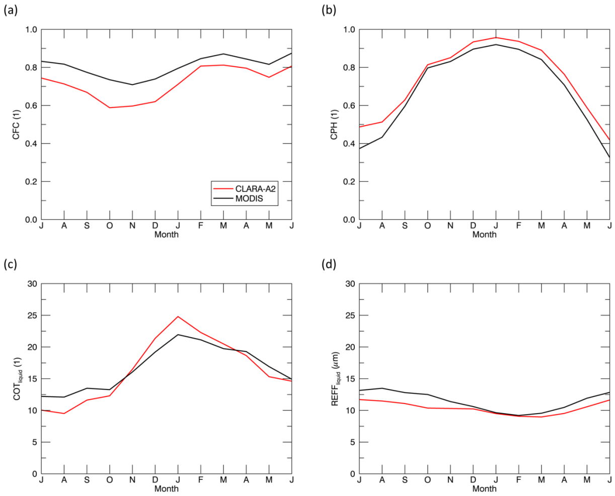
Figure 6. Seasonal variations in cloud properties over southern China, based on CLARA-A2 and MODIS data, during the period 2006-2015. (a) Total CFC, (b) cloud phase (CPH; fraction of liquid clouds relative to total CFC), (c) COT for liquid clouds and (d)
