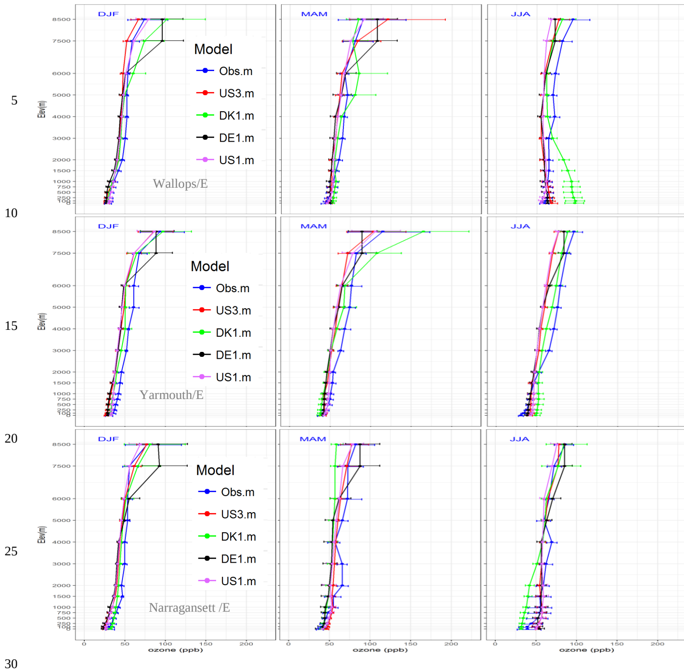
Figure 3: Seasonal vertical profiles of ozone mixing ratios for 2010 (left: winter; middle: spring; right: summer), for stations located in the eastern part of the domain. The horizontal lines indicate the 95% bootstrapped confidence interval for each vertical layer. Note: Narragansett has limited amount of ozonesondes for all seasons (less than 10 for each season) and the results should be viewed with caution.
