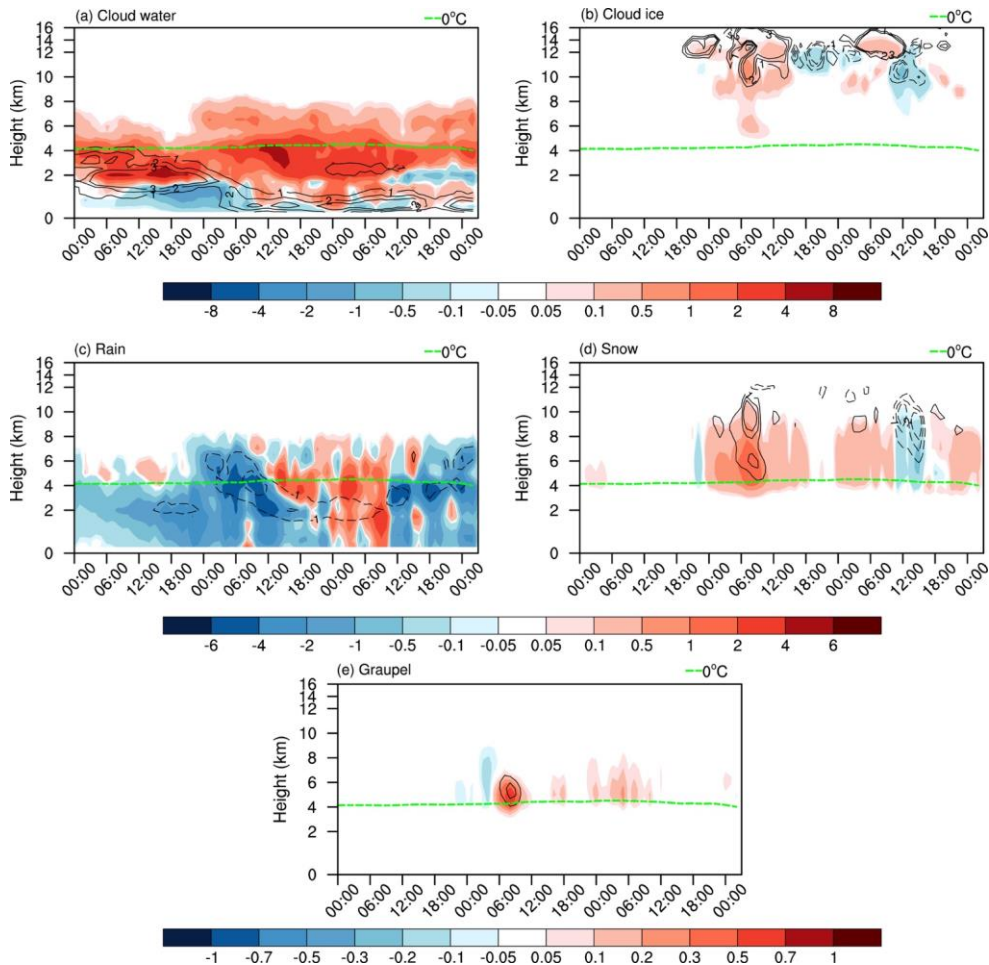
Figure 6. Differences with time (abscissa) and height (ordinate) in (a) cloud water (shading; 10^{-5} kg kg ^{-1} ) and CDNC (contour; 10^7 kg ^{-1} ), (b) cloud ice (shading; 10^{-5} kg kg ^{-1} ) and CINC (contour; 10^4 kg ^{-1} ), (c) rain (shading; 10^{-5} kg kg ^{-1} ) and rain number concentration (contour; 10^5 kg ^{-1} ), (d) snow (shading; 10^{-4} kg kg ^{-1} ) and snow number concentration (contour; 10^3 kg ^{-1} ), and (e) graupel (shading; 10^{-4} kg kg ^{-1} ) and graupel number concentration (contour; 10^3 kg ^{-1} ) between CTL and CLEAN averaged over R1.
