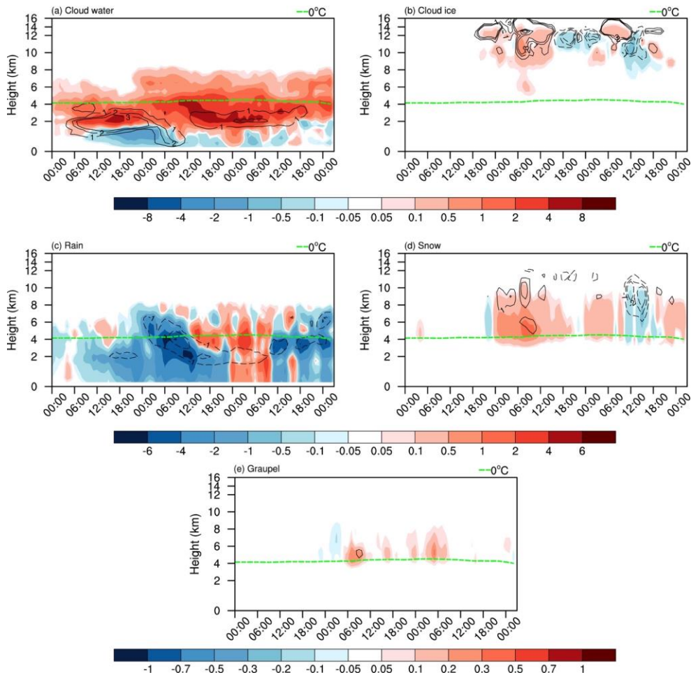
Figure 9. Differences with time (abscissa) and height (ordinate) in (a) cloud water (shading; 10^{-5} kg \text{kg}^{-1} ) and CDNC (contour; 10^7 \text{kg}^{-1} ), (b) cloud ice (shading; 10^{-5} kg \text{kg}^{-1} ) and CINC (contour; 10^4 \text{kg}^{-1} ), (c) rain (shading; 10^{-5} kg \text{kg}^{-1} ) and rain number concentration (contour; 10^5 \text{kg}^{-1} ), (d) snow (shading; 10^{-4} kg \text{kg}^{-1} ) and snow number concentration (contour; 10^3 \text{kg}^{-1} ), and (e) graupel (shading; 10^{-4} kg \text{kg}^{-1} ) and graupel number concentration (contour; 10^3 \text{kg}^{-1} ) between D1 and CLEAN averaged over R1.
