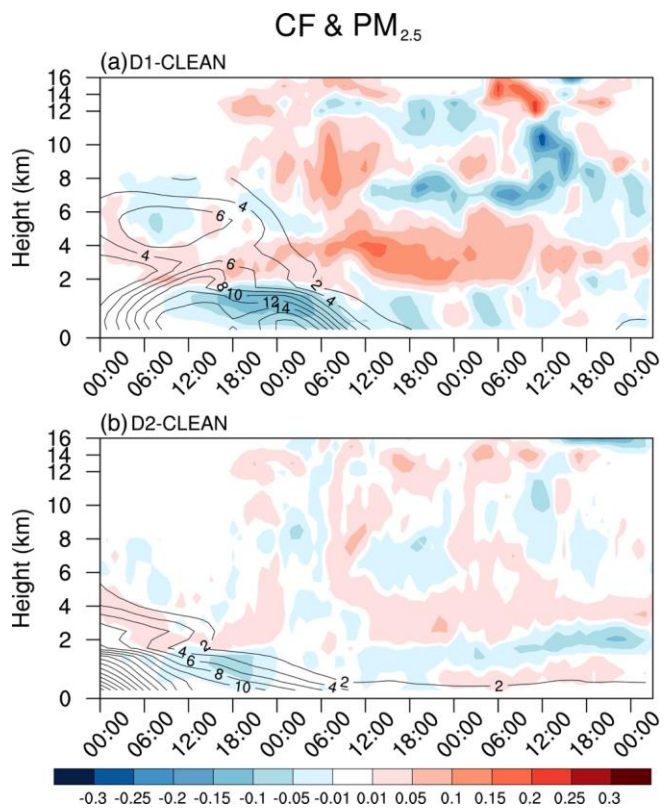
Figure 8. Differences in time-height cross section of CF (shading; unitless) and PM 2.5 concentration (contour; µg m -3 ) averaged over R1 between (a) D1 and CLEAN and (b) D2 and CLEAN.
