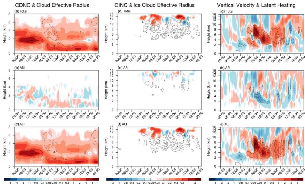
Figure 5. Differences with time (abscissa; from 00Z on December 14 to 02Z on December 17) and height (ordinate) in (a) cloud droplet number concentration (CDNC, shading; 10^7 \text{ kg}^{-1} ) and cloud effective radius (contour; \mu\text{m} ), (d) cloud ice number concentration (CINC, shading; 10^5 \text{ kg}^{-1} ) and ice cloud effective radius (contour; \mu\text{m} ), and (g) vertical velocity (shading; \text{cm s}^{-1} ) and latent heating (contour; \text{K d}^{-1} ) averaged over R1 between CTL and CLEAN. (b, e, h) Same as (a, d, g) but for differences between CTL and ARIOff. (c, f, i) Same as (a, d, g) but for differences between ARIOff and CLEAN. For CINC and ice cloud effective radius, only cloud ice is considered. Zero-value contour lines are omitted, and negative values are dashed.
