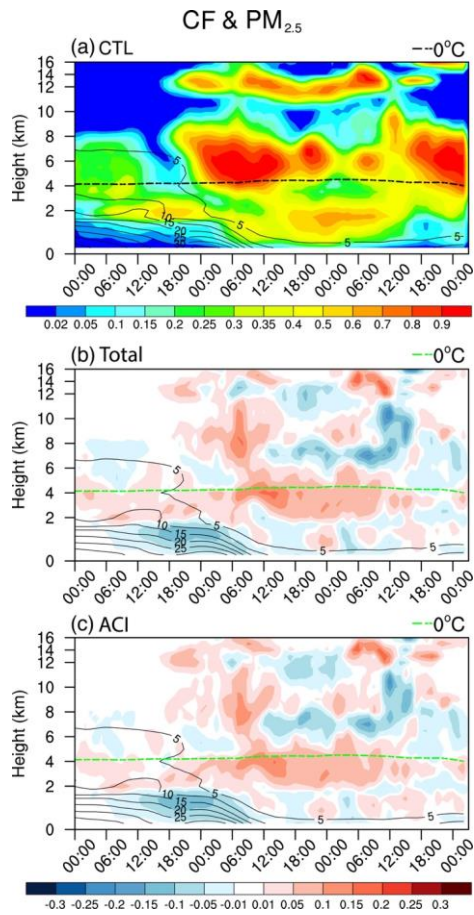
Figure 4. (a) Time-height cross section of cloud fraction (CF; shading; unitless) and PM 2.5 concentration (contour; \mu\text{g m}^{-3} ) averaged over R1 in CTL run. Differences in the time-height cross section of CF (shading; unitless) and PM 2.5 concentration (contour; \mu\text{g m}^{-3} ) averaged over R1 shown in Figure 3 between (b) CTL and CLEAN and (c) ARIoff and CLEAN. The cloud fraction is calculated as sum of cloud water, cloud ice and snow. Dashed lines denote 0°C isotherm calculated as the averaged zero-layer height over R1.
