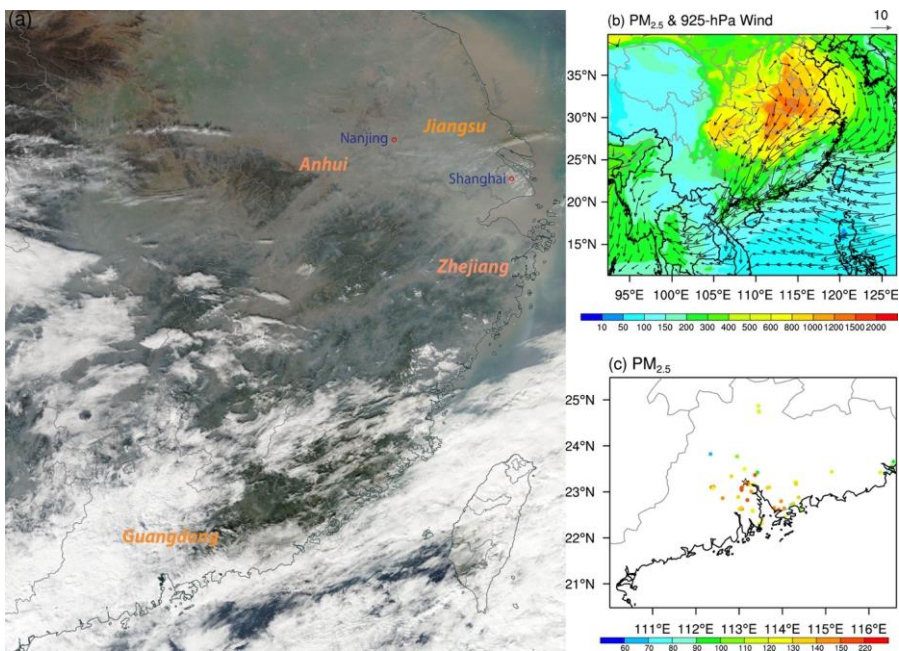
Figure 1. (a) Terra satellite true-color image of east China on December 13, 2013 (UTC), provided by NASA's Worldview (source: https://worldview.earthdata.nasa.gov/ ). Red circles denote city locations, blue fonts denote cities, and orange fonts in bold italic denote provinces. (b) Spatial distribution of 3-day averaged column-integrated PM 2.5 concentration (shading; \mu\text{g m}^{-2} ) and 925-hPa wind (vector; \text{m s}^{-1} ) during December 14–16, 2013, in control run. The red box denotes the analysis region. (c) Hourly-averaged PM 2.5 concentration on December 13, 2013, observed in Guangdong Province. Colored circles denote in situ station locations, and black star denotes Guangzhou.
