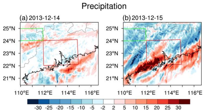
5 Figure 11. Differences in precipitation (mm) between 10x and CLEAN on (a) December 14 and (b) December 15.
