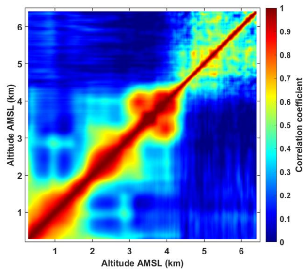
Figure 6: Lidar-derived correlation matrices for a) the entire measurement period between 24 June and 17 July, 2014, and b) the undisturbed period (without aerosol load anomaly in the free troposphere). These matrices are symmetric by construction.
