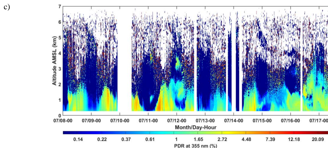
Figure 3: Same as Figure 2, for the period between 8 and 17 July.
