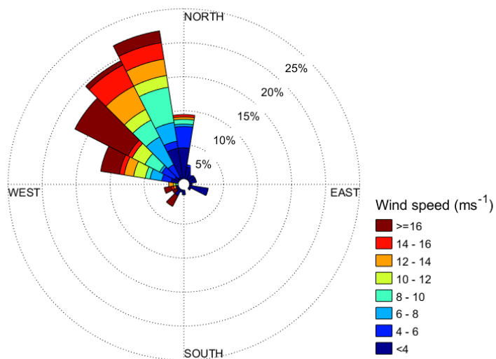
Figure 8: Same as Figure 7, for the pressure level of 700 hPa (~3 km AMSL).
