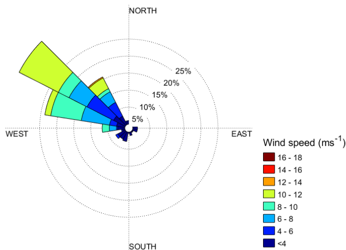
5 Figure 7: Frequency of counts (%) by wind speed direction at 975 hPa (~0.4 km AMSL) for a) disturbed cases, days with aerosol anomaly within the free troposphere and b) undisturbed cases, days without anomaly. The hourly data are from the Era5 reanalyzes at 0.25° of horizontal resolution.
