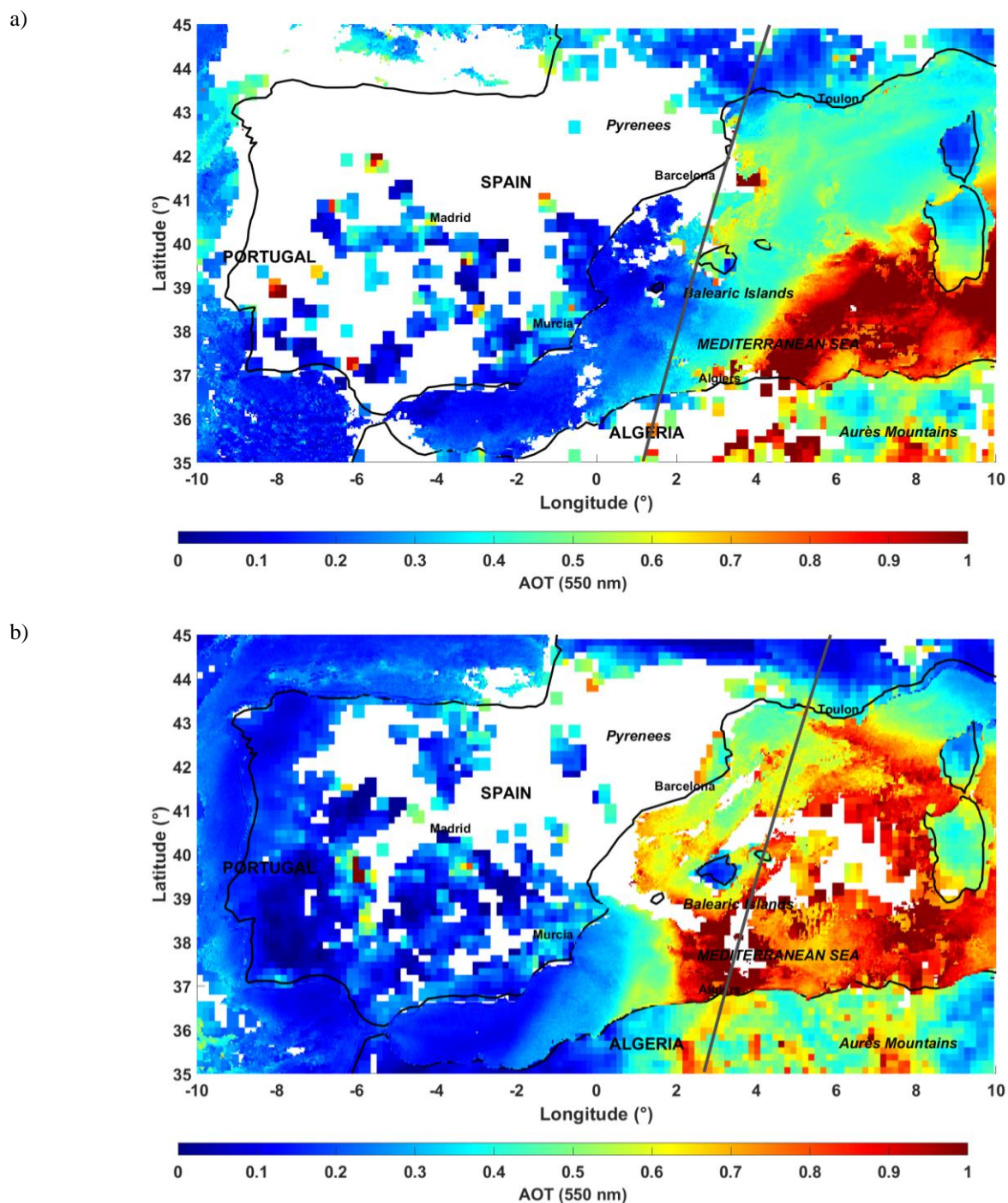
Figure 14: AOT at 550 nm derived from the composition between MODIS over land and SEVIRI over sea observations: a) is on 24 June, 2014 and b) on 3 July, 2014. The nearest night time (~0200 UTC) ground tracks of CALIOP are given in dark-grey continuous lines.
