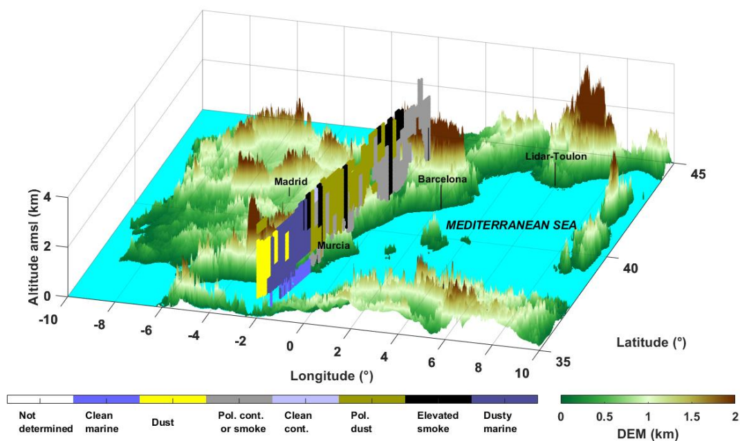
Figure 12: a) AOT at 550 nm derived from the composition between MODIS over land and SEVIRI over sea observations on 25 August, 2014. The nearest night time (~0215 UTC) ground tracks of CALIOP are given in dark-grey continuous lines. b) CALIOP-derived aerosol typing (version 4.10) as observed on August, 2014. DEM is the digital elevation model.
