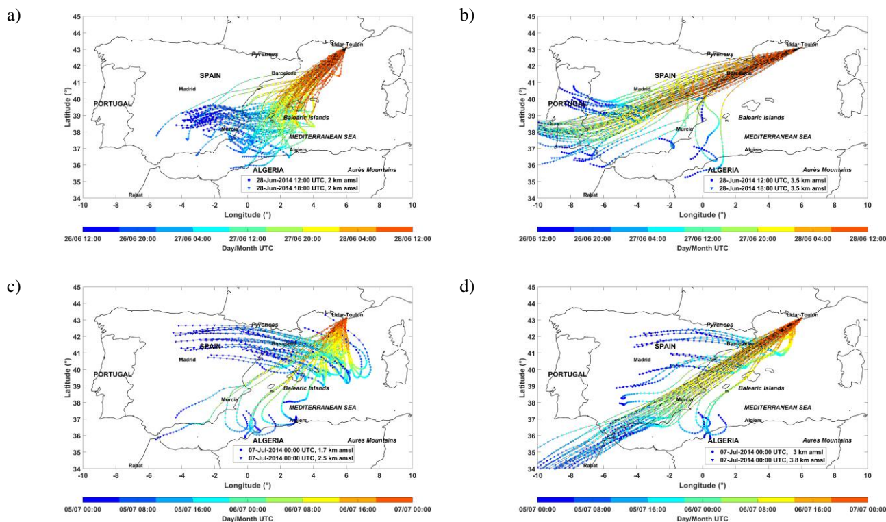
Figure 10: Two-days back trajectories from the French Riviera (Toulon, 43.13556 ° N, 6.00944 ° E). The altitudes of the end locations of the air mass trajectories are in the main pollution plumes detected by the ground-based N 2 -Raman lidar on a) 28 June, 2014 for an end location of 2 km, b) 28 June, 2014 for an end location of 3.5 km, c) 7 July, 2014 for end locations of 1.7 and 2.5 km, and d) 7 July, 2014 for end locations of 3 and 3.8 km. The Hysplit model worked in its ensemble mode, i.e. 27 back trajectories computed for each end location.
