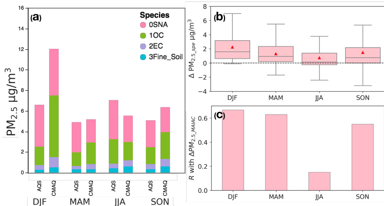
5 Figure 6 (a) Seasonal average PM 2.5 speciation from CMAQ vs. AQS observations in 2011 evaluated at 54 CSN and IMPROVE sites. (b) Box plots showing the distribution of estimated biases of daily satellite-derived PM 2.5 due to model biases in PM 2.5 speciation ( \Delta PM_{2.5\_spe} ) by season for 2011. Red triangles show the seasonal mean biases. (c) Pearson correlation coefficient between the biases in PM 2.5_MAIAC ( \Delta PM_{2.5\_MAIAC} ) and \Delta PM_{2.5\_spe} .
