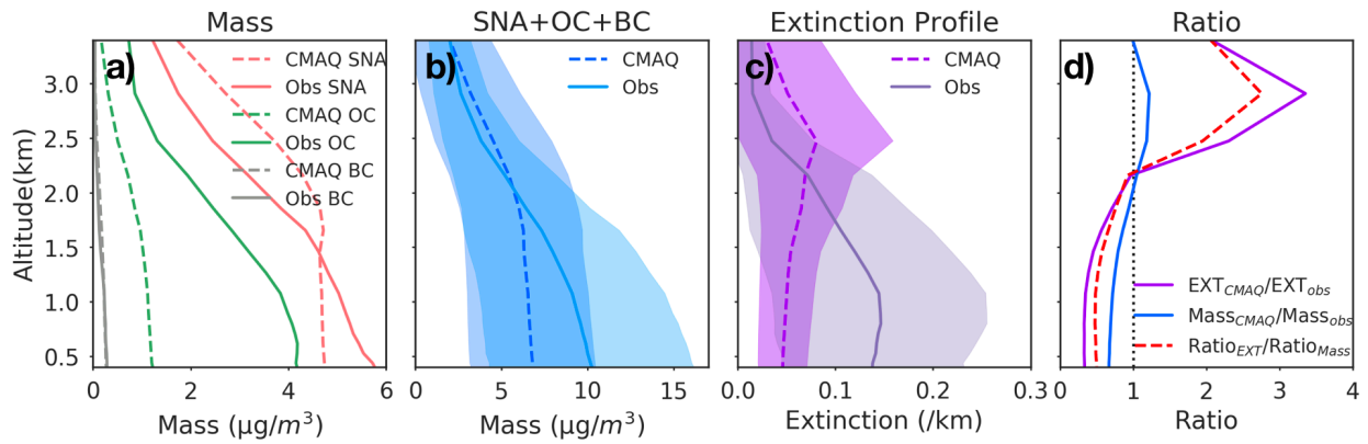
Figure 7 Campaign-mean vertical profiles of: (a) aerosol composition, (b) total mass 5 (SNA+OC+BC), and (c) extinction from CMAQ vs. observations from the DISCOVER-AQ 2011 Baltimore-Washington D.C. campaign. (d) Campaign-mean vertical profile of the model-to- observation ratio of extinction ( \text{Ratio}_{\text{EXT}} ), total aerosol mass ( \text{Ratio}_{\text{Mass}} ) and \text{Ratio}_{\text{EXT}}/\text{Ratio}_{\text{Mass}} . Aircraft observations are first aggregated to match model layers, and corresponding model values are sampled concurrently with the time of observations. CMAQ modeled extinction is estimated 10 with FlexAOD using the default parameters in Table 1. The shading in (b) and (c) shows the standard deviation of the day-to-day variability.
