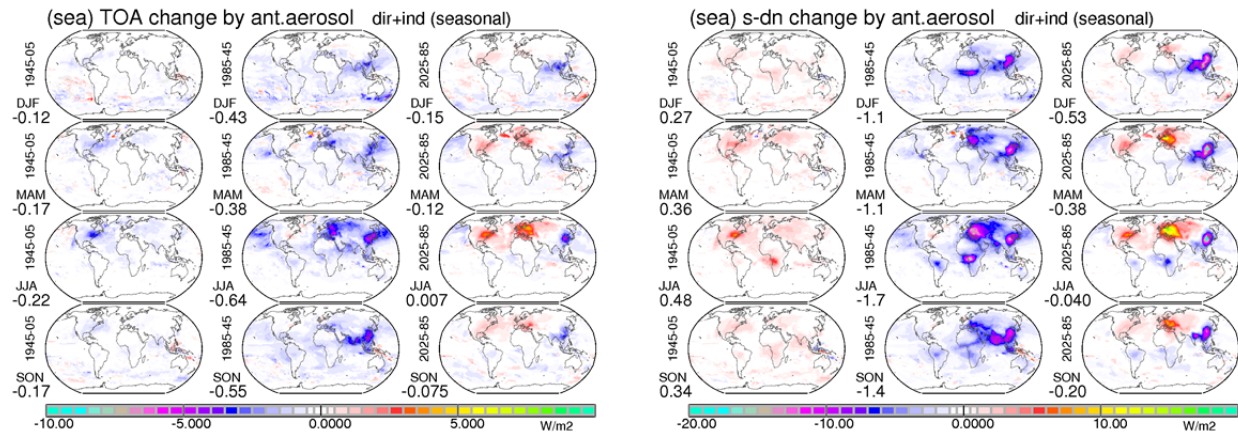
12 Figure 18. Seasonal changes over 20 year periods (1945-1905, 1985-1945, 2025-1985) in aerosol forcing 13 (left block) and to solar downward fluxes by anthropogenic aerosol (right block). Blue colors indicate 14 time-periods of increased cooling aerosol or a dimming (decreases to the solar surface fluxes), while red 15 colors indicate time-periods of a reduced cooling by aerosol or a brightening (increases the solar surface 16 fluxes). Values below the labels indicate global average changes for the selected time periods.
