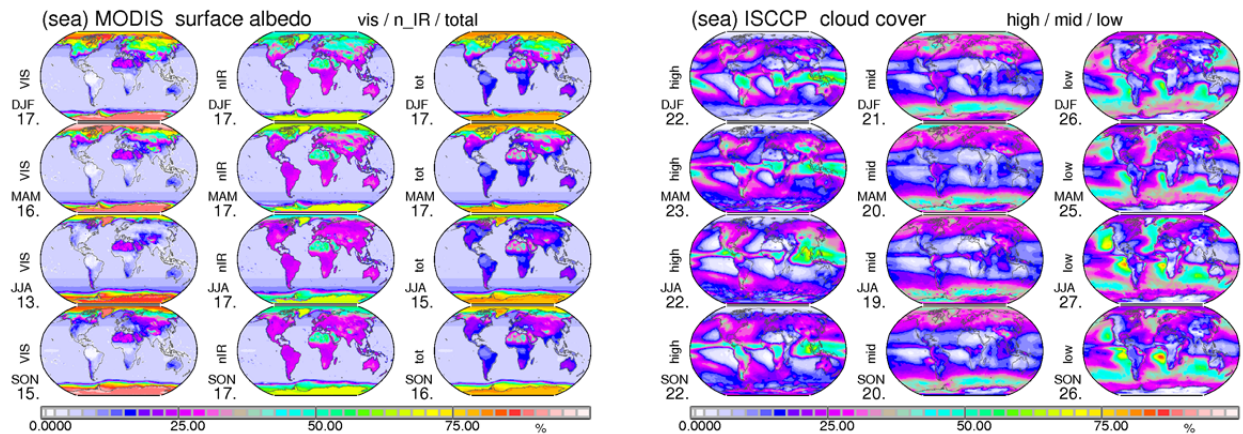
29 Figure 4 Seasonal averages for applied environmental properties to (1) solar surface albedo (left block) 30 for the UV/VIS, the near-IR and the total spectral range based on MODIS satellite sensor data and (2) 31 ISCCP based cloud cover (right block) for high (<440hPa), mid (440-680hPa) and low (>680hPa) altitudes.
