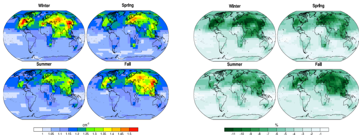
1 2 3 Figure A4 seasonal CDNC factor increases (left) and associated droplet radius reductions in % (right) due 4 to today's anthropogenic aerosol and the pre-industrial fine-mode background as defined by MACv2. 5 6
