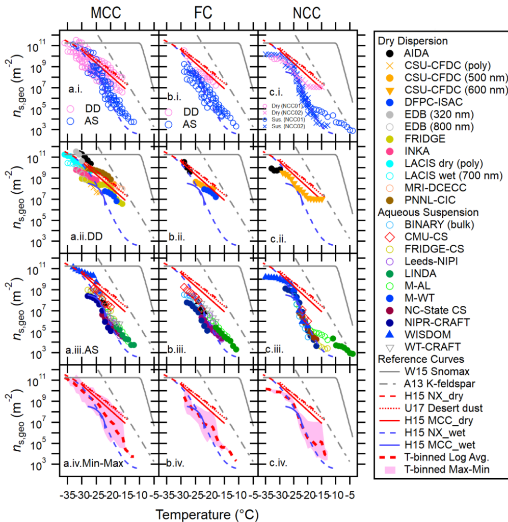
Figure 1. Immersion freezing n_{s,geo}(T) spectra for MCC (a), FC (b) and NCC (c) from different techniques. Dry dispersion results (DD, pink markers) and aqueous suspension results (AS, blue markers) are shown in (i) to highlight the difference between these two subsets. Inter-comparisons of DD and AS for each cellulose sample type using T -binned n_{s,geo} are presented in (ii) and (iii), respectively. The log average of all results as well as the deviation between maxima and minima of n_{s,geo}(T) are shown in (iv). Reference immersion freezing n_s(T) spectra for MCC (H15a) illite NX (H15b), Snomax ( Wex et al. , 2015), desert dusts (U17; Ullrich et al. , 2017) and K-feldspar (A13; Atkinson et al. , 2013) are also shown (See Sect. 4.1 ). For NCC, the results from two different batches (NCC01 from Dec 2014 and NCC02 from May 2015) are shown.
