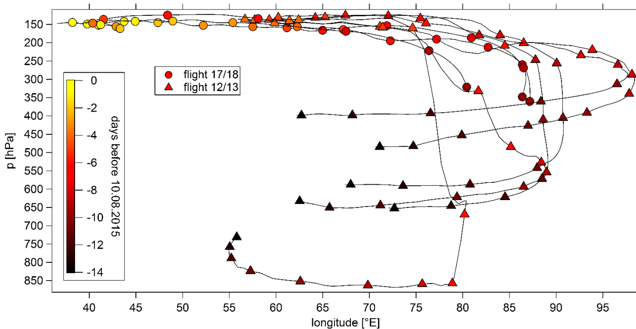
5 Figure 27: Centroid back trajectories for enhanced CH 4 mixing ratios during flight 12/13 (triangles) and flight 17/18 (circles) with colour coded days before the release on August 10, 2015.
