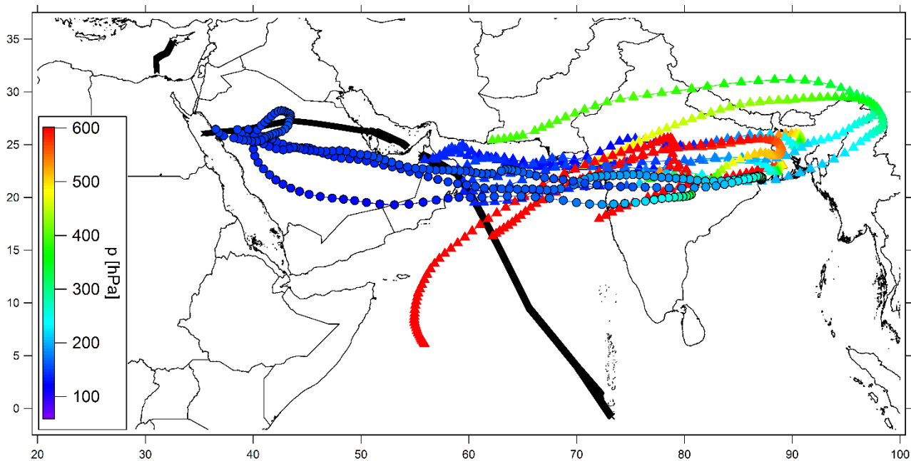
Figure 26: Centroid back trajectories for enhanced CH 4 mixing ratios during flight 12/13 (triangles) and flight 17/18 (circles) with colour coded height.
