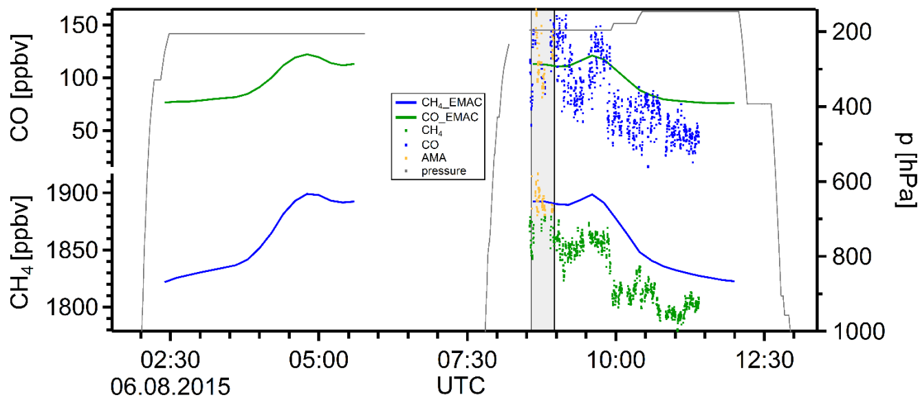
Figure 24: Flight 12/13 (August 6, 2015) in situ CH 4 and CO data and EMAC results along the flight track, as well as the flight altitude. The AMA is colour coded by CH 4 >1879.8 ppbv.
