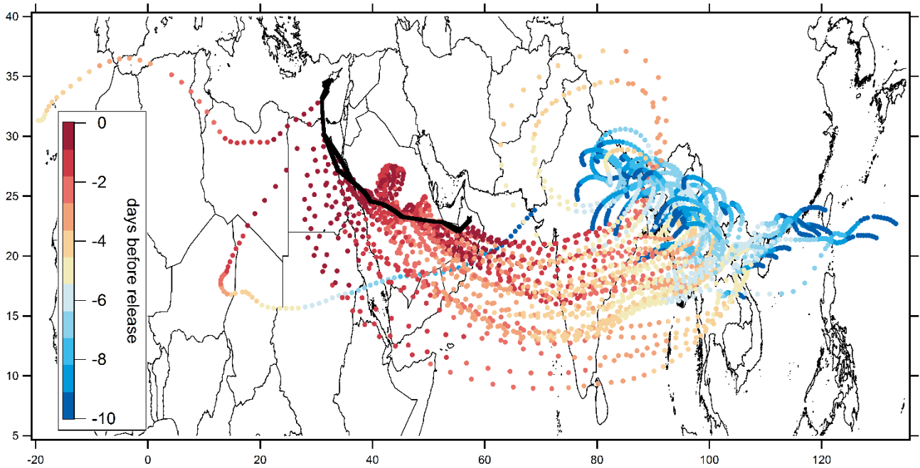
5 Figure 5: Centroid trajectories for flight 19 (August 13, 2015) with colour coded transport time.
