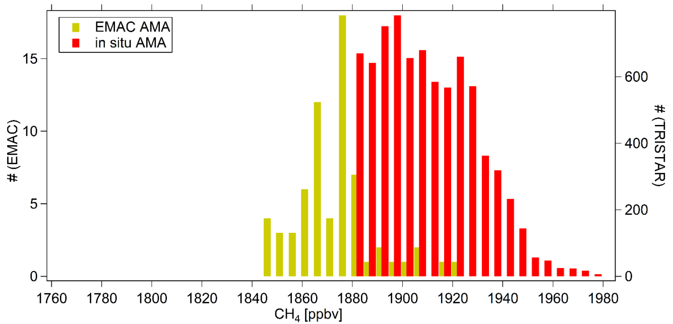
Figure 16: Histogram for in situ measured and EMAC modelled CH 4 within the altitude range 300-140 hPa, both for background and AMA air.
