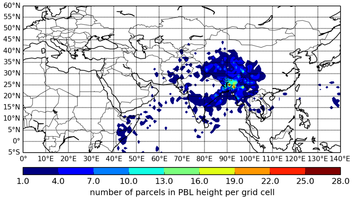
Figure 13: Last boundary layer contact of parcels before they were transported to the track of flight 19 (10 days prior to flight).
