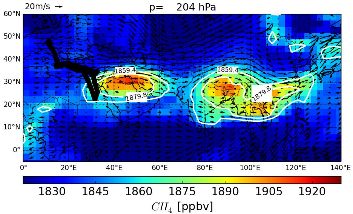
Figure 21: Double anticyclone mode illustrated with wind field and CH_4 EMAC daily means at 204 hPa (August 25, 2015) and the associated flight tracks. White contours represent CH_4 threshold and background values according to section 3.1.
