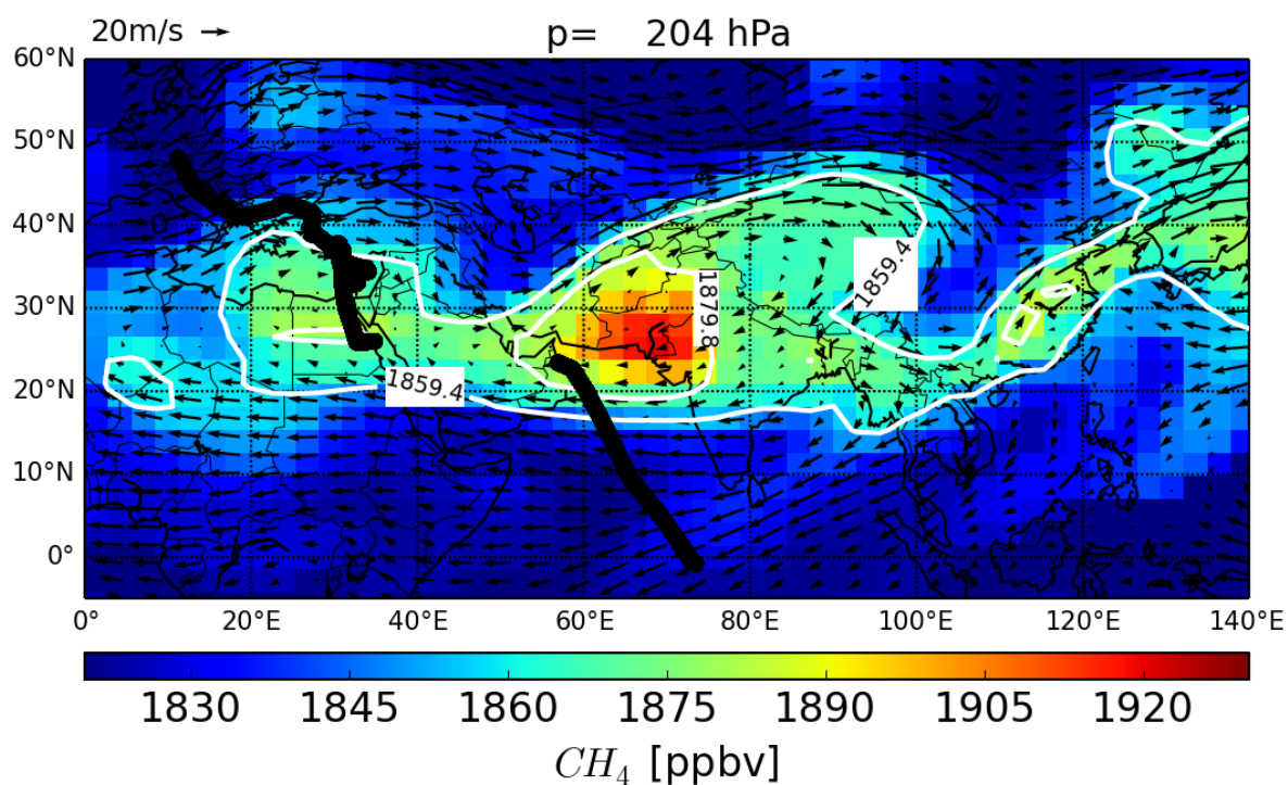
5 Figure 18: Double anticyclone mode illustrated with wind field and CH 4 EMAC daily means at 204 hPa (July 25, 2015) and the associated flight tracks. White contours represent CH 4 threshold and background values according to section 3.1.
