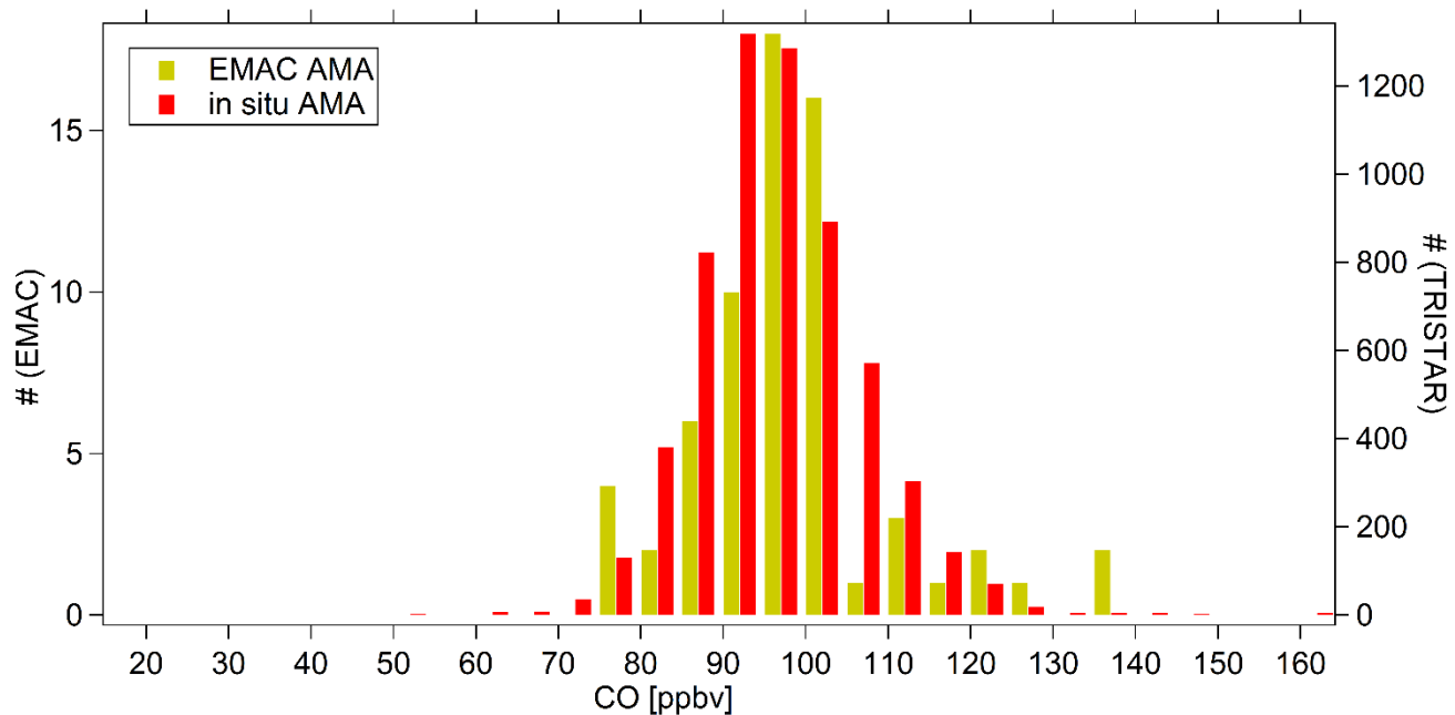
Figure 17: Histogram for in situ measured and EMAC modelled CO within the altitude range 300-140 hPa, both for background and AMA air.
