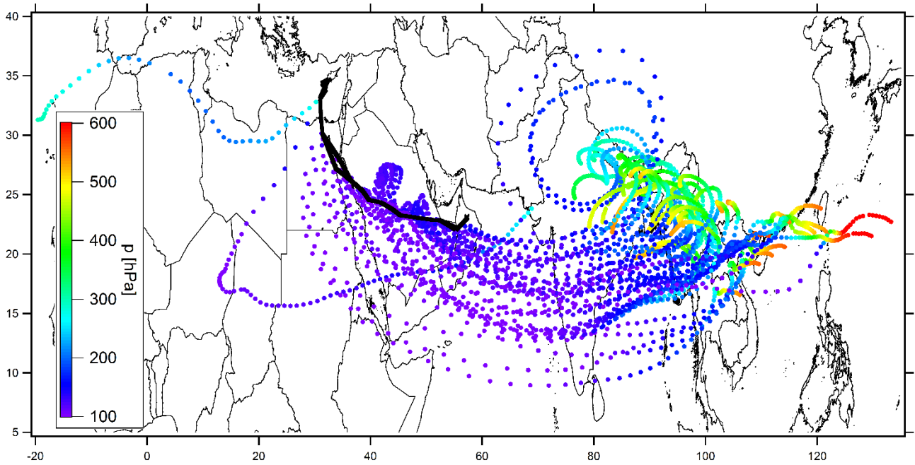
Figure 4: Centroid trajectories for flight 19 (August 13, 2015) with colour coded altitude.
