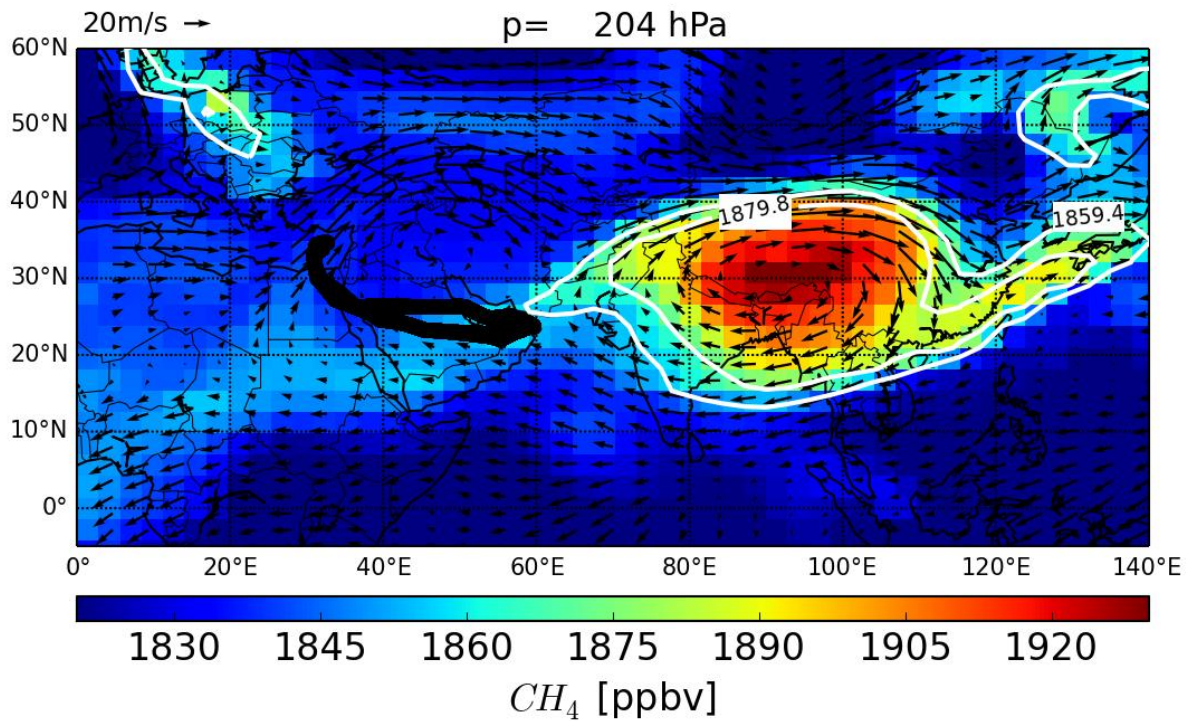
Figure 20: Tibetan anticyclone mode illustrated with wind field and CH_4 EMAC daily means at 204 hPa (August 15, 2015) and the associated flight tracks. White contours represent CH_4 threshold and background values according to section 3.1.
