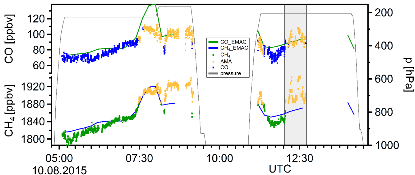
Figure 25: Flight 17/18 (August 10, 2015) in situ CH 4 and CO data and EMAC results along the flight track, as well as the flight altitude. The AMA is colour coded by CH 4 >1879.8 ppbv.
