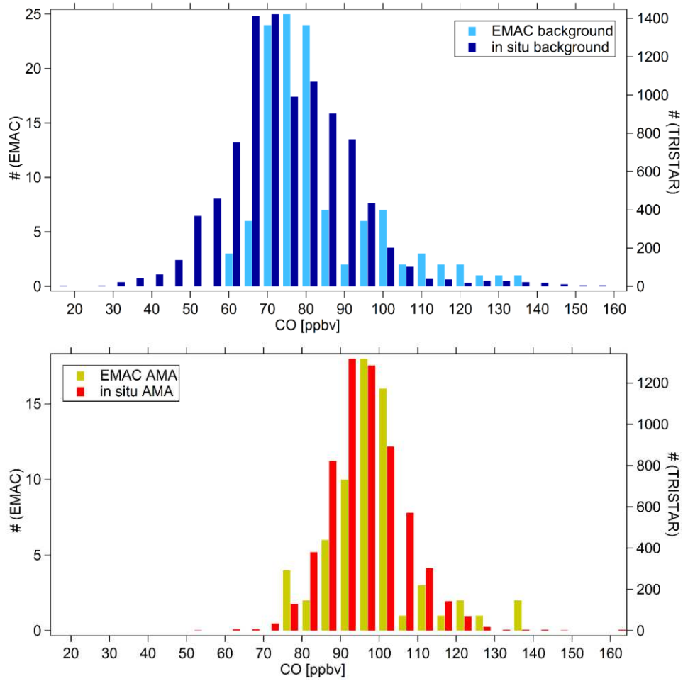
Figure 157: Histogram for in situ measured and EMAC modelled CO within the altitude range 300-140 hPa, both for background and AMA air.
