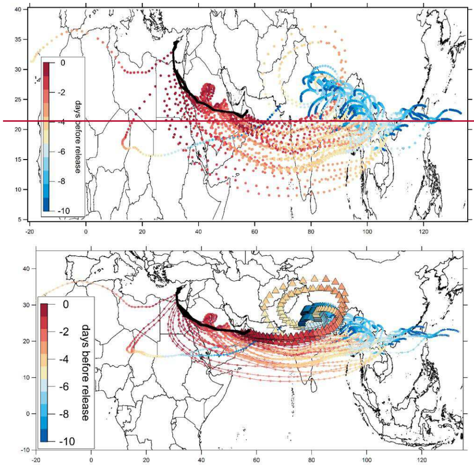
Figure 5: Centroid trajectories for flight 19 (August 13, 2015) with colour coded transport time. Triangles are back trajectories for CH 4 mixing ratios above the CH 4 threshold and circles for below the CH 4 threshold.
