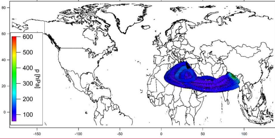
Figure S2: Flight 09 (07.25.2015): measurement flight from Paphos to Paphos over Cyprus.
