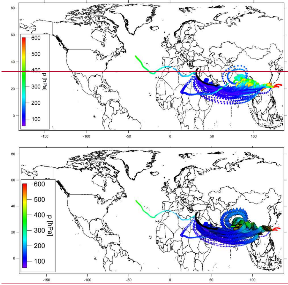
Figure S9: Flight 19 (08.13.2015): measurement flight from Paphos to Paphos towards Oman.
