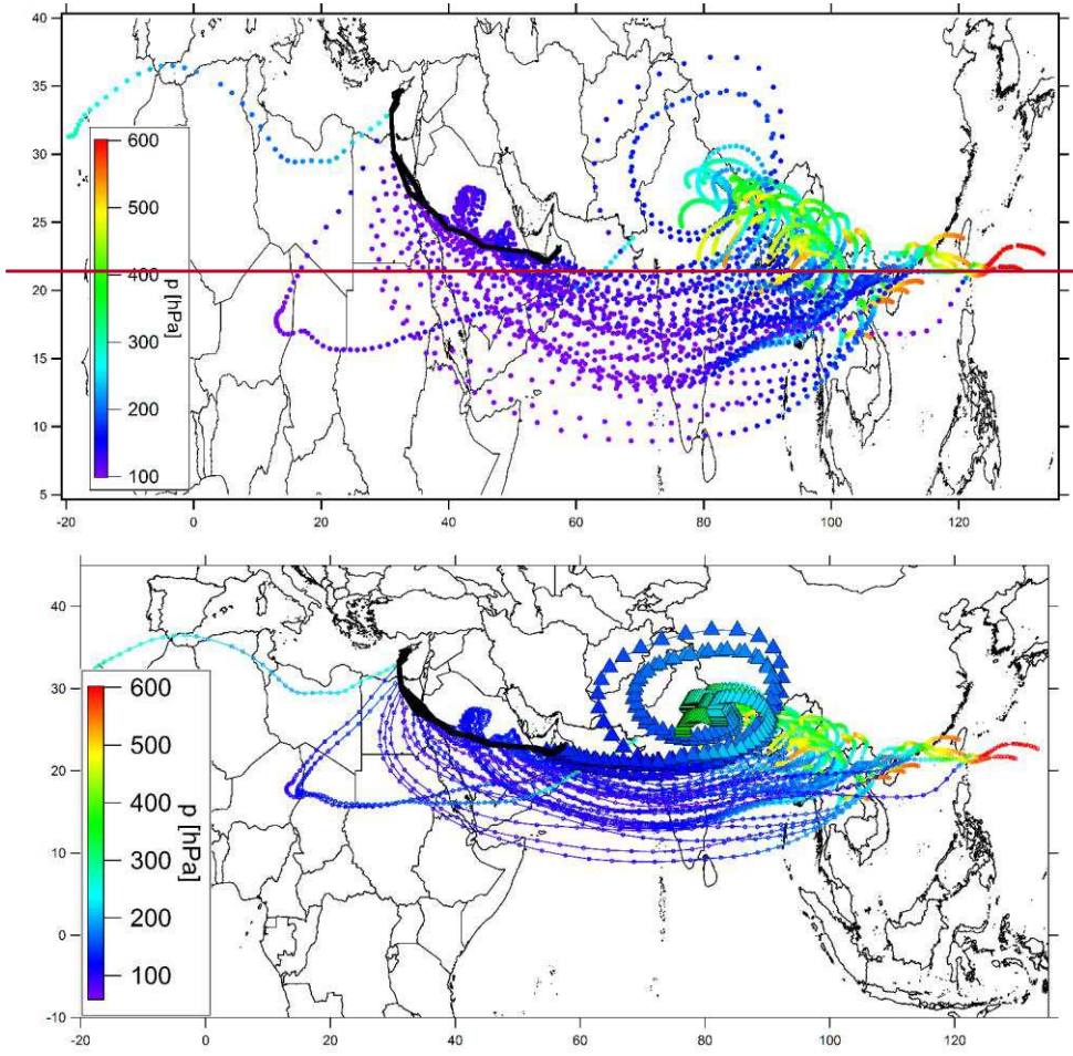
Figure 4: Centroid trajectories for flight 19 (August 13, 2015) with colour coded altitude. Triangles are back trajectories for CH 4 mixing ratios above the CH 4 threshold and circles for below the CH 4 threshold.
