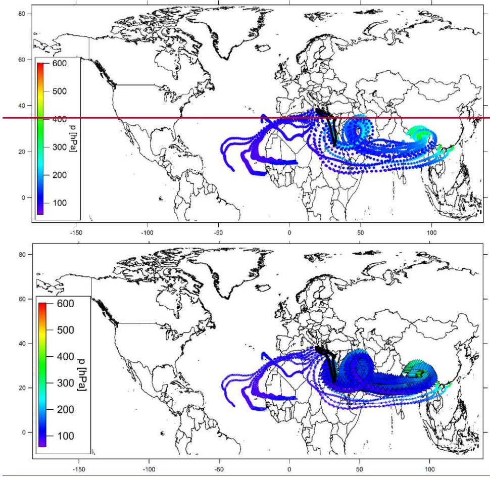
5 Figure S12: Flight 22 (08.23.2015): measurement flight from Paphos to Paphos over Egypt, Greece, the Mediterranean; with profiles over Egypt.
