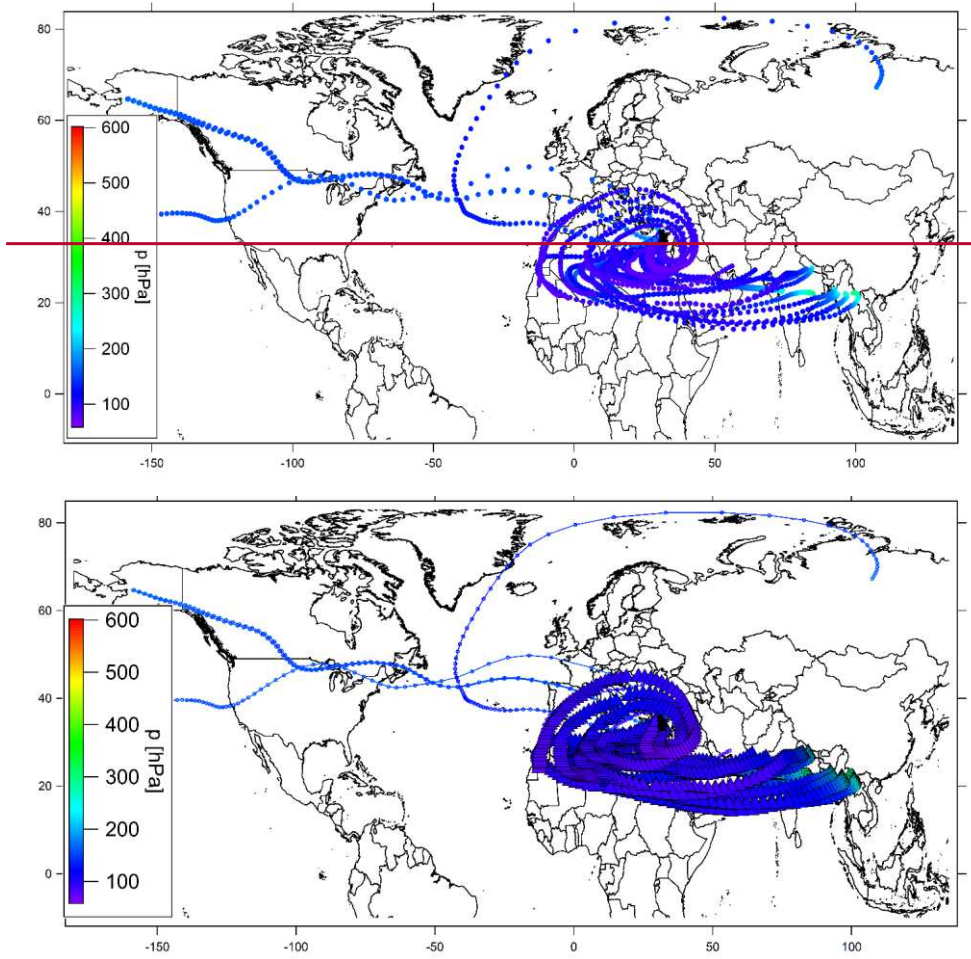
Figure S3: Flight 10 (07.28.2015): measurement flight from Paphos to Paphos over Cyprus.
