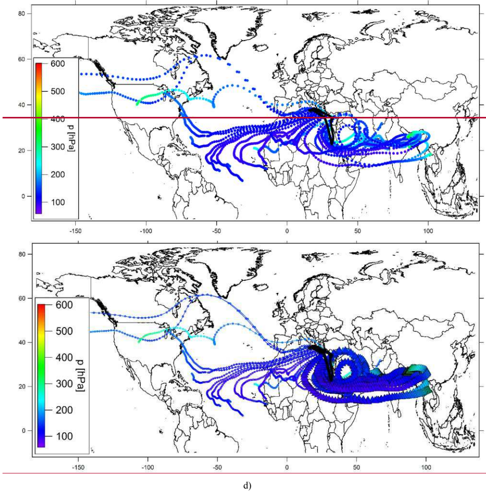
d) Figure S13: Flight 23 (08.25.2015): measurement flight from Paphos to Paphos over Egypt, Etna, the Mediterranean; with profiles over Egypt and low altitude at the Etna.
