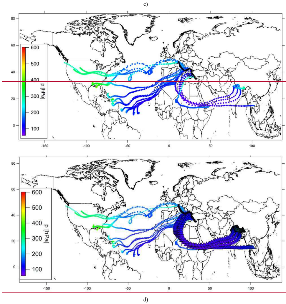
5 Figure S2S1: Flight 08 (07.21.2015): transfer flight from Oberpfaffenhofen to Paphos.
