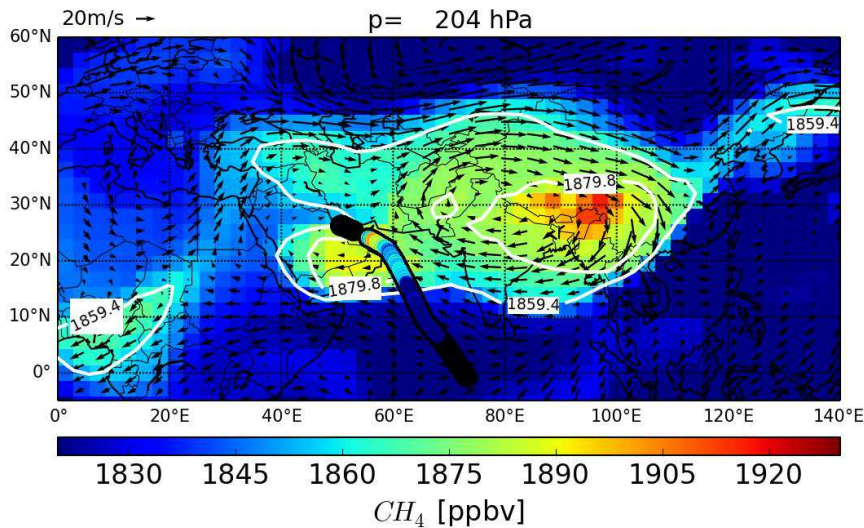
Figure 202: EMAC calculated \text{CH}_4 and wind field; daily means at 204 hPa, and in situ \text{CH}_4 (above 300 hPa) along the aircraft track for flight 12/13 (August 06, 2015). White contours represent \text{CH}_4 threshold and background values according to section 3.1. [The enhanced \text{CH}_4 values over Oman represent the outflow.]
