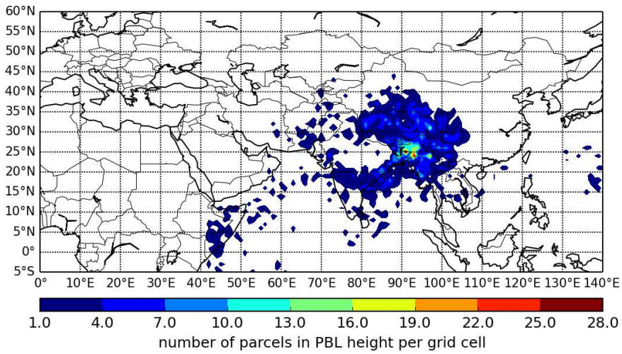
Figure 1|3: Last boundary layer contact of parcels from trajectories, which start along the flight track at locations with CH 4 mixing ratios above the threshold , before they were transported to the track of flight 19 (10 days prior to flight).
