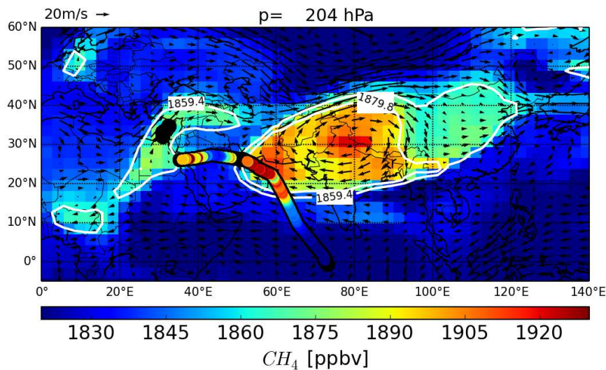
Figure 213: EMAC calculated \text{CH}_4 and wind field; daily means at 204 hPa, and in situ measured \text{CH}_4 (above 300 hPa) along the aircraft track for flight 17/18 (August 10, 2015). White contours represent \text{CH}_4 threshold and background values according to section 3.1. The enhanced \text{CH}_4 values over the Read Sea represent the outflow.
