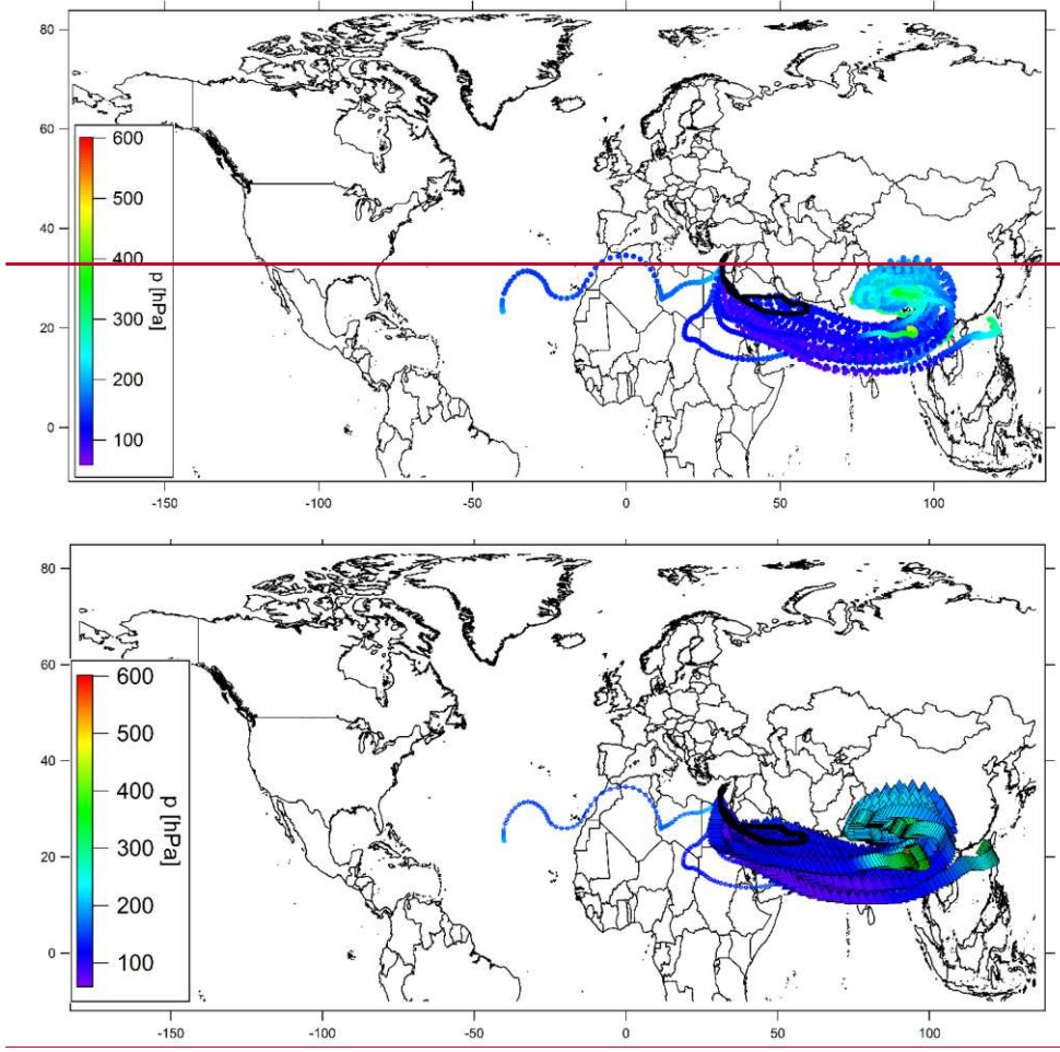
Figure S11: Flight 21 (08.18.2015): measurement flight from Paphos to Paphos towards Oman.
