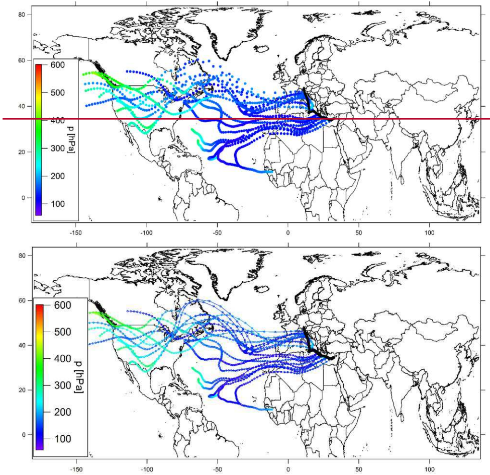
Figure S14: Flight 24 (08.27.2015): transfer flight from Paphos to Oberpfaffenhofen via Etna with low altitude.
