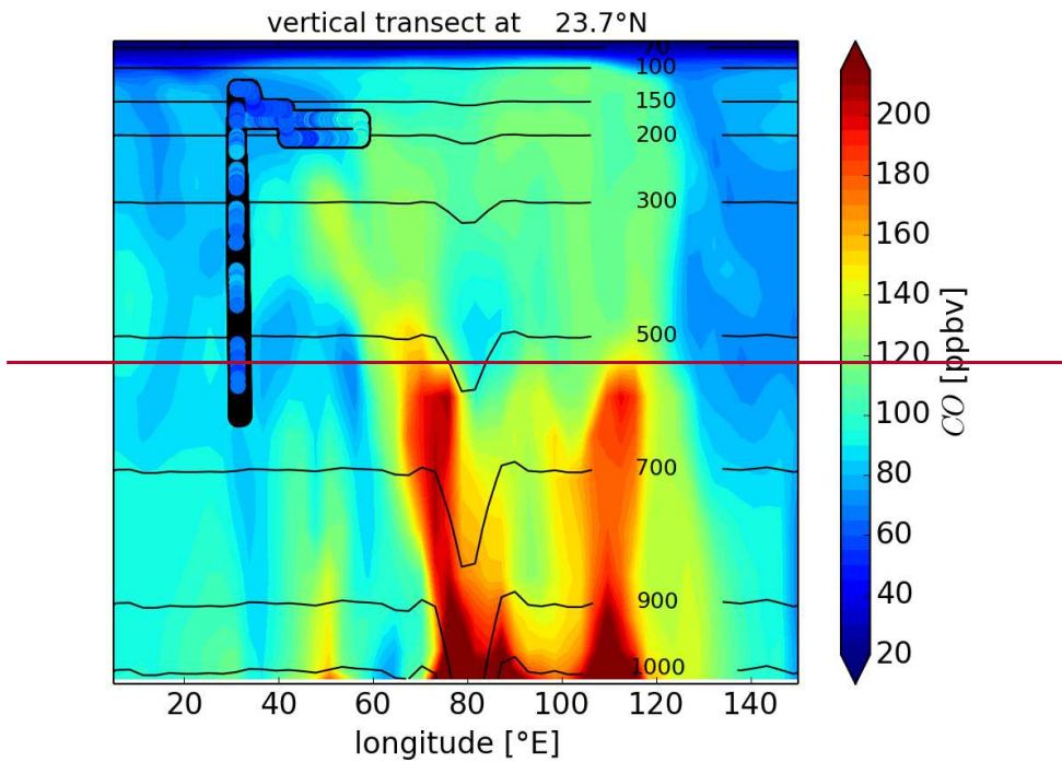
Figure 11: EMAC modelled CO; daily mean transect along 23.7°N, and CO measured along the aircraft track for flight 19.
