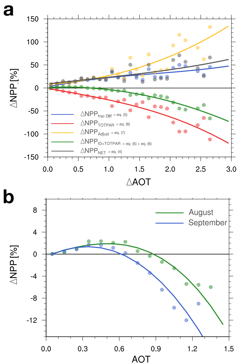
5 Figure 8: Showing on a) the relative changes in NPP ( \Delta NPP_{Neb} in grey), the relative changes in NPP due to the ‘change in diffuse fraction’ ( \Delta NPP_{Frac\ Diff} in blue), ‘reduction in total PAR’ ( \Delta NPP_{TOTPAR} , in red), the sum of ‘change in diffuse fraction and reduction in total PAR’ ( \Delta NPP_{fD+TOTPAR} , in green, i.e. the DFE) and the climate feedback ( \Delta NPP_{Adjust} in yellow) against the anomalies in the AOT at 550nm for the month of August. Showing on b) a zoom on the relative changes in NPP due to ‘change in diffuse fraction and reduction in total PAR’ ( \Delta NPP_{fD+TOTPAR=DFE} ) – i.e. the changes in NPP only due to change in surface radiation (i.e. the DFE), for August (green) and September (blue) as a function of the total AOT at 550 nm. The dashed lines highlight the AOT thresholds where DFE switch from a positive to a negative impact.
