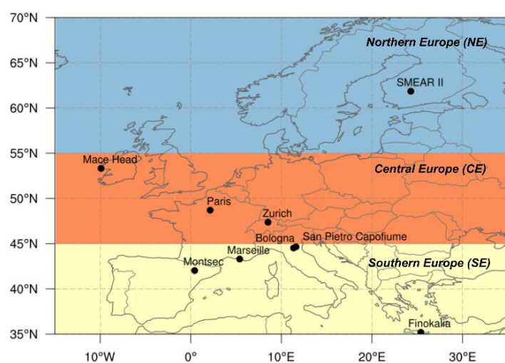
Figure 1. Model domain and location of ACSM/AMS measurement stations.
