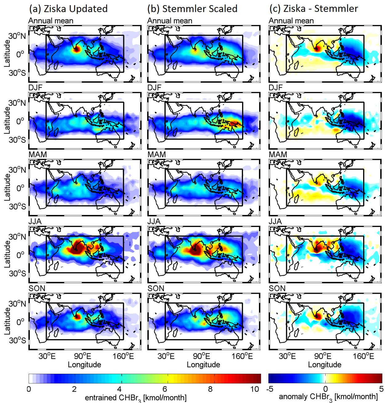
505 Figure 5: Amount of CHBr 3 injected to the stratosphere within 1°x1° grid cells plotted on the geographical location of CPT crossing for monthly averaged bromoform emissions for (a) Ziska Updated and (b) Stemmler Scaled emission inventories. (c) Differences in entrainmentinjection between the two inventories (a) - (b). The black box depicts the Indian Ocean/West Pacific release area.
