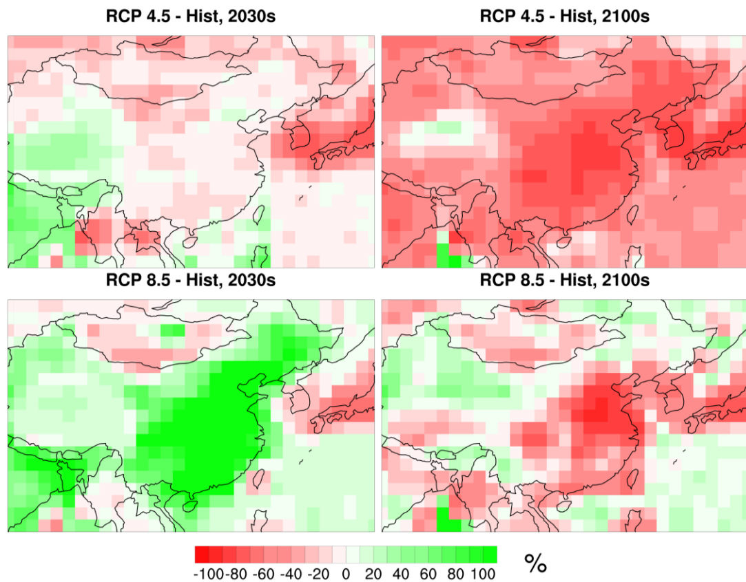
Fig. S1. Spatial distribution of mean annual NO x emission change under RCP 4.5 and RCP 8.5 in relative to historical period (2001-2010).
