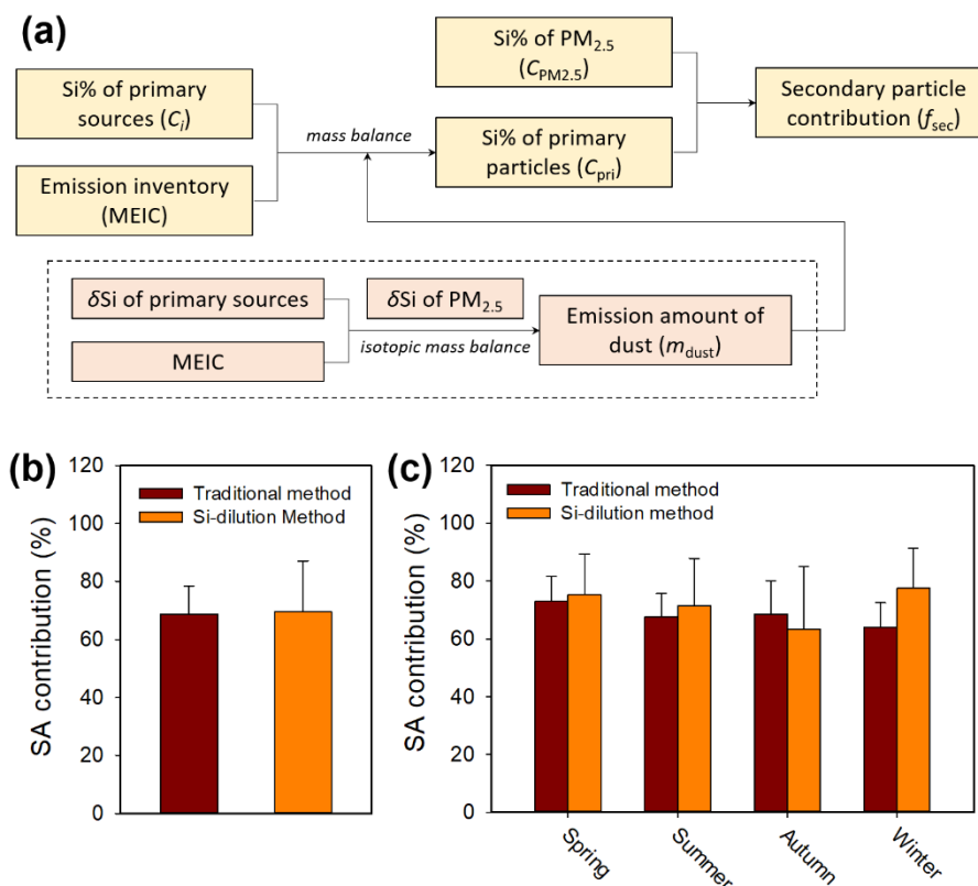
Figure 4. Comparison of the SA estimate results between the Si-dilution method and the traditional method. (a) , A flow chart showing how the f_{sec} was obtained by the Si-dilution method. (b) , Annual mean SA contribution to PM_{2.5} in Beijing. (c) , Seasonal mean SA contribution in Beijing. Note: the error bars for the Si-dilution method include both method uncertainty and the variations of samples on different dates (see Sect. 2.6); while for the traditional method the error bars only represent the variations of samples on different dates (without method uncertainty). Please see text for a more detailed discussion on the uncertainties.
