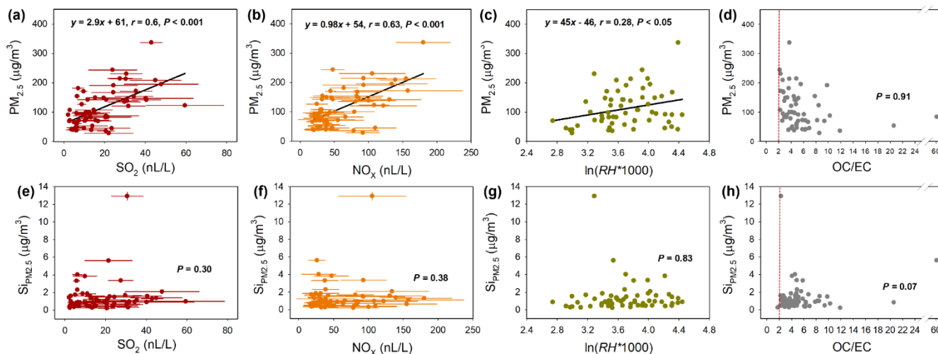
Figure 3. Correlation analysis of PM 2.5 concentration and Si PM2.5 with typical secondary aerosol precursors and relative humidity (RH). (a)-(d), Correlation of PM 2.5 concentration with SO 2 (a), NO x (b), RH (c) and OC/EC ratio (d). (d)-(f), Correlation of Si PM2.5 with SO 2 (e), NO x (f), and RH (g) and OC/EC ratio (h). The red dotted lines in (d) and (h) represent OC/EC = 2, which can be used to indicate the formation of secondary aerosols at OC/EC > 2 (Chow et al., 1994).
