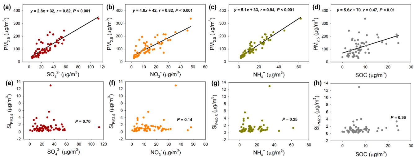
Figure 2. Correlation analysis of PM 2.5 concentration and its Si content (Si PM 2.5 ) with the secondary species in PM 2.5 . (a)-(d), Correlation of PM 2.5 concentration with SO 4 2- (a), NO 3 - (b), NH 4 + (c), and SOC (d). (e)-(h), Correlation of Si PM 2.5 with SO 4 2- (e), NO 3 - (f), NH 4 + (g), and SOC (h).
