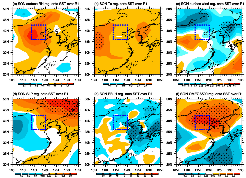
46 Figure S1. As in Fig. 4, but for SST over R1.
