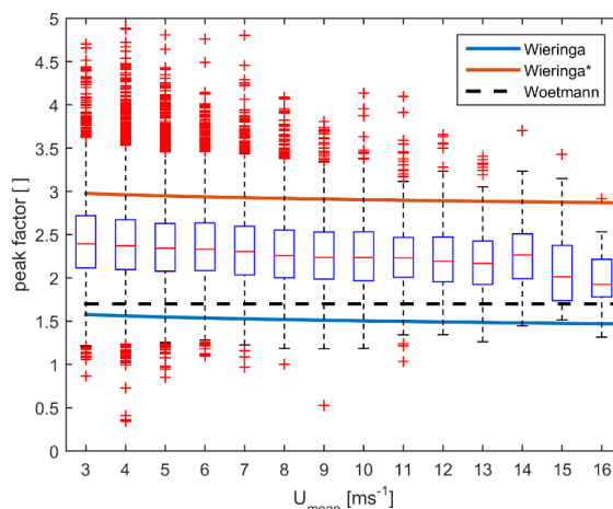
Figure 9: Box plot of gust peak factor ( k_{\text{peak}} ) estimates at 60 m a.g.l. from all nine towers as a function of U_{\text{mean}} . Also shown are estimates from Eq. (9) (Wieringa, 1973) and a revised empirical function in which the leading term in Eq. (9) is increased from 1.0 to 2.4 (Wieringa*) and a constant value of 1.7 value (Woetmann Nielsen and Petersen, 2001).
