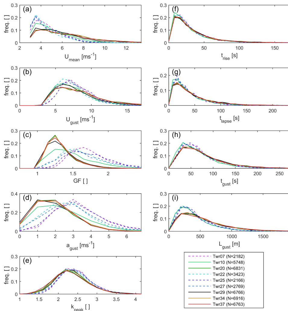
5 Figure 3: Distributions of gust parameters at each of the 9 towers (using data collected at 60 m a.g.l) for 10 minute periods with U_{\text{mean}} > 3 \text{ ms}^{-1} . Valley towers are shown with dashed lines and ridge towers with solid lines. The frames show the (a) 10 minute mean wind speed ( U_{\text{mean}} ), (b) gust magnitude ( U_{\text{gust}} ), (c) gust factor (GF), (d) gust amplitude ( a_{\text{gust}} ), (e) peak factor ( k_{\text{peak}} ) (f) rise time ( t_{\text{rise}} ) (g) lapse time ( t_{\text{lapse}} ), (h) gust duration ( t_{\text{gust}} ) and (i) gust length scale ( L_{\text{gust}} ). The legend reports the sample size (N) for 10 minute periods used to construct the empirical distributions for each tower. The towers are denoted by the color scheme introduced in Figure 1.
