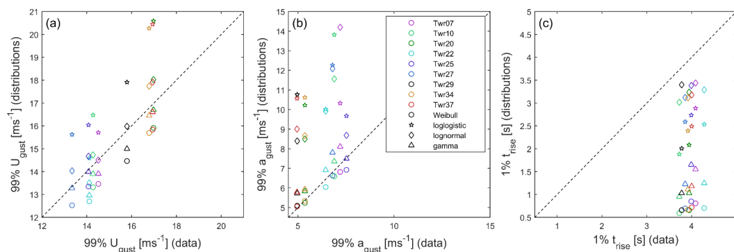
Figure 4: (a) 99 th percentile wind gust magnitude ( U_{\text{gust}} ), (b) 99 th percentile amplitude ( a_{\text{gust}} ) and (c) 1 st percentile rise time ( t_{\text{rise}} ) as derived directly from the observations at 60 m a.g.l. and estimated from the parametric distributional fits (shown by the different symbols). The towers are denoted by the color scheme introduced in Figure 1. The dashed line indicates 1:1 correspondence.
