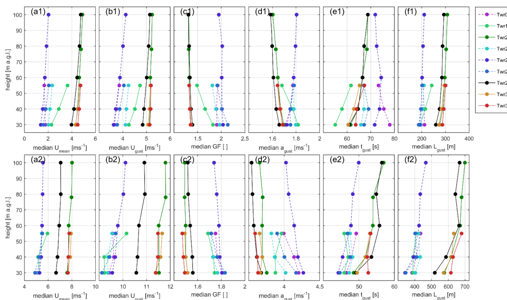
Figure 7: Median values of the gust parameters, by height, at each of the nine towers. Row 1 shows median values computed for all 10 minute periods and row 2 shows median values for 10 minute periods which meet the gust criteria: U_{\text{mean}} > 3 \text{ ms}^{-1} and gust amplitude > 4 \text{ ms}^{-1} . (a) 10 minute mean wind speed ( U_{\text{mean}} ), (b) 3 s maximum wind speed ( U_{\text{gust}} ), (c) gust amplitude ( a_{\text{gust}} ), (d) gust factor (GF), (e) gust duration ( t_{\text{gust}} ), (f) gust length scale ( L_{\text{gust}} )
