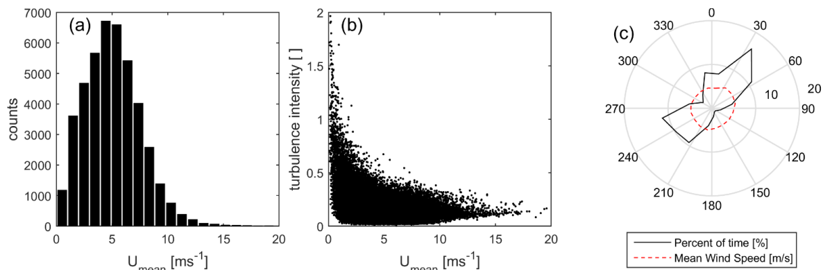
10 Figure 2: Overview of wind conditions at Perdigoão. (a) 10 minute mean wind speed distribution at 60 m a.g.l. on Tower 29. (b) 10 minute turbulence intensities versus mean wind speed at 60 m a.g.l. on Tower 29. (c) Wind rose and mean wind speed from data collected at 60 m a.g.l. on Tower 29.
