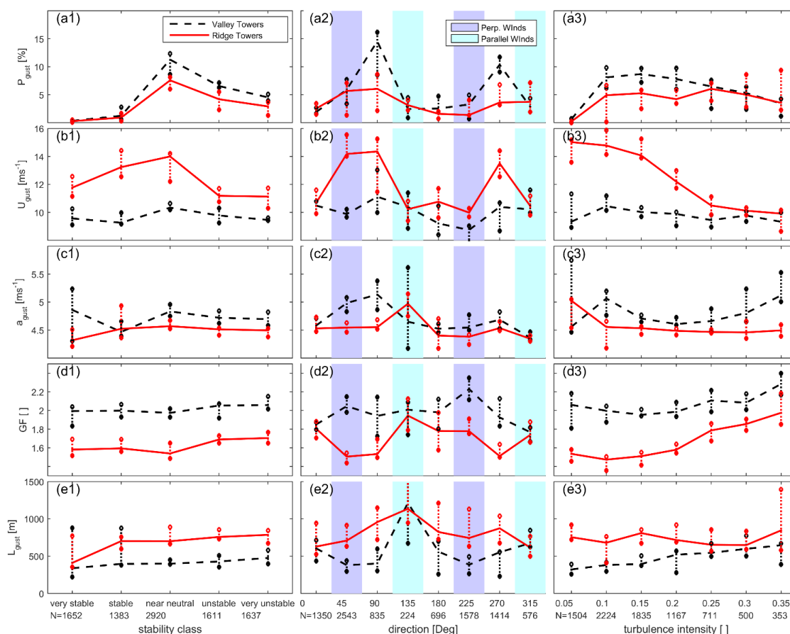
Figure 6: Median gust parameters during gusty conditions ( U_{\text{mean}} > 3 \text{ ms}^{-1} , a_{\text{gust}} > 4 \text{ ms}^{-1} ) at 60 m a.g.l. from ridge (solid red) and valley (dashed black) towers. The data sampled are conditionally sampled by stability classes based on Monin-Obukhov length (column 1), wind direction (column 2) and turbulence intensity (column 3) as measured at Tower 29 (60 m a.g.l.). Vertical whiskers at each data point denote the range of median parameter values for all towers in each class. N values in the second row of x-axis labels are the number of 10 minute periods in each sample. One gust parameter is shown per row: (a) Probability of a gust (i.e. percentage of 10 minute periods that meet the gust criteria), (b) Gust magnitude ( U_{\text{gust}} ), (c) gust amplitude ( a_{\text{gust}} ), (d) gust factor GF, (e) gust length scale ( L_{\text{gust}} ).
