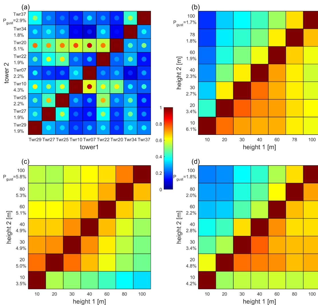
5 Figure 10: Co-occurrence of wind gusts in individual 10 minute periods between sonic anemometers deployed on different towers (frame a) or at different heights on the same meteorological mast (frame b-d). The color scale for each of the four panels indicates probability of a wind gust at anemometer 2 (on the vertical axis) during any 10 minute period that also has a gust at anemometer 1 (on the horizontal axis). The marginal probability of a wind gusts is also shown along the y axis. (a) Co-occurrence probabilities for gusts at 60 m a.g.l. across all 9 towers. Towers are sorted by their distance from Tower 29, colored dots in each square show the probability of co-occurrence when the time window is extended to 30 minutes. Also shown is the co-occurrence of wind gusts at different heights on (b) Tower 20, (c) Tower 25 and (d) Tower 29.
