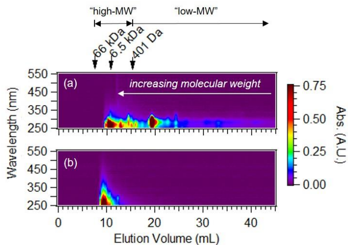
5 Figure 3. Molecular weight separated absorption spectra of a) unreacted water soluble BrC from laboratory generated wood smoke and b) ambient WS BrC from fresh biomass burning emissions (~ 1 hour of atmospheric transport) collected during the 2016 fire season in Crete, Greece. The elution volumes for high-MW and low-BrC and some calibration standards with known molecular weights are provided for reference. Note that molecular weight increases with decreasing elution volumes.
