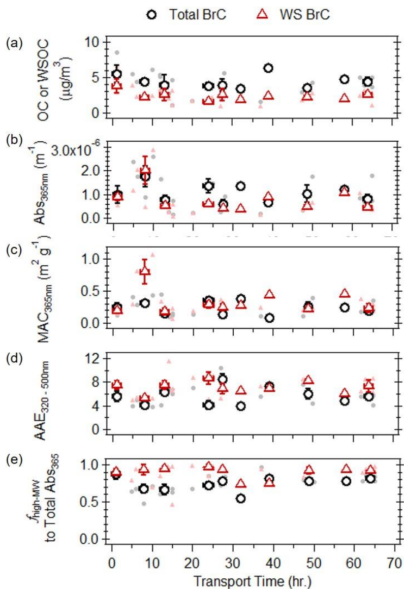
5 Figure 6. a) Organic carbon (OC) or water-soluble organic carbon (WSOC) concentrations, b) light absorption at 365nm, c) mass absorption coefficients at 365nm, d) AAE (in the wavelength range of 320 - 500nm) and e) fractional contribution of high-molecular weight fractions to total light absorption as a function of atmospheric transport time, for MeOH (black circles) and water (red triangles) extractable portion of the ambient filters collected on Crete Island, Greece during the 2016 and 2017 fire seasons. The filled points are individual filter measurements, the open points represent the binned median values and the associated error bars represent the interquartile range.
