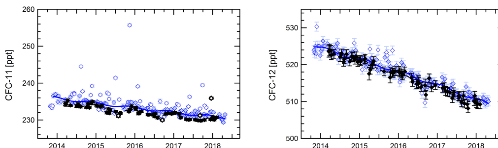
Figure 2. Time series of CFC-11 (a) and CFC-12 (b) at Taunus Observatory (coloured symbols) and Mace Head (black symbols). The solid line represents a 2nd order polynomial harmonic fit to the TO baseline dataset, the dashed line the corresponding fit to the Mace Head data. Open symbols denote samples flagged as outliers.
