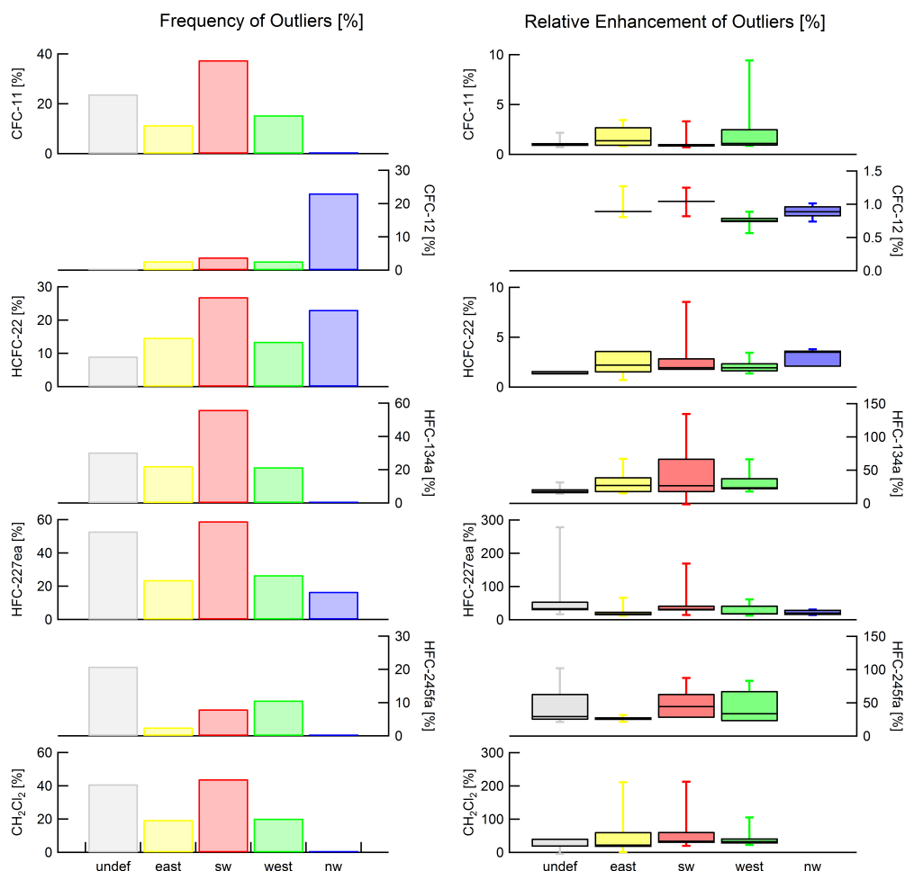
Figure 11. Left: Distribution of samples with enhanced mixing ratios across trajectory origin sectors. Except for CFC-12 outliers occur most frequently when trajectories originate from the south-west. Right: Box-Whisker-Plots of relative enhancement of outlier mixing ratios. Whiskers indicate minimum and maximum enhancements of mixing ratios of samples identified as outliers relative to the baseline fit. Boxes represent 25- and 75-percentiles, bars indicate the median for each sector. Remarkable features are the high relative enhancements of CFC-12 and HCFC-22 when trajectories originate from the north-west sector and high outlier enhancements of dichloromethane under easterly influence.
