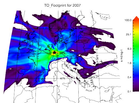
Figure 1. Contour plot of source sensitivity of Taunus Observatory derived from bi-weekly particle dispersion calculation for the year 2007. Taunus Observatory is located at 50.22° N, 8.44° E. Data courtesy of D. Brunner.
