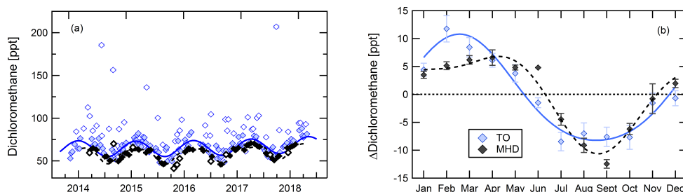
Figure 9. Time series (a) and seasonality (b) of dichloromethane at Taunus Observatory (blue) and at Mace Head (black). Open symbols in the time series indicate samples flagged as outliers. Seasonality is shown as difference of the monthly mean to the mean of the full detrended baseline time series.
