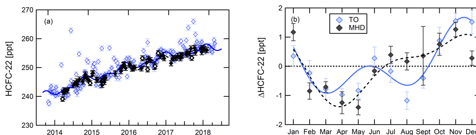
Figure 6. Time series (a) and seasonality (b) of HCFC-22 at Taunus Observatory (blue) and at Mace Head (black). Open symbols in the time series indicate samples flagged as outliers. Seasonality is shown as difference of the monthly mean to the mean of the full detrended baseline time series.
