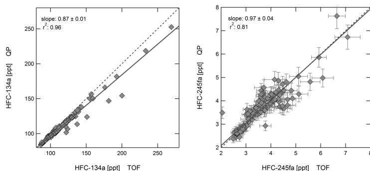
Figure 4. Correlation at Taunus Observatory of HFC-134a and HFC-245 for the mass spectrometers employed, a quadrupole (QP) and a time-of-flight (TOF) mass spectrometer. The solid line represents an orthogonal fit to the data points, the dotted line indicates the 1:1-line. For HFC-134a a non-linearity is observed for the TOF-MS but not for HFC-245fa. Error bars of HFC-134a mixing ratios are smaller than symbol size.
