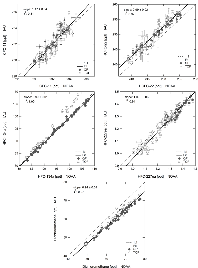
Figure 3. Correlation of CFC-11, HCFC-22, HFC-134a, HFC-227ea, and dichloromethane in Frankfurt flask samples (IAU) with canister samples of the NOAA network analysed by GC/MS (data available at: ftp://ftp.cmdl.noaa.gov/hats/ ) at Mace Head. Results from the Frankfurt GC/MS system are reported on AGAGE scales resulting in a constant offset for some substances. Because of the known non-linearity of the TOF instrument, for HFC-134a the correlation parameters are derived for the QP mass spectrometer only.
