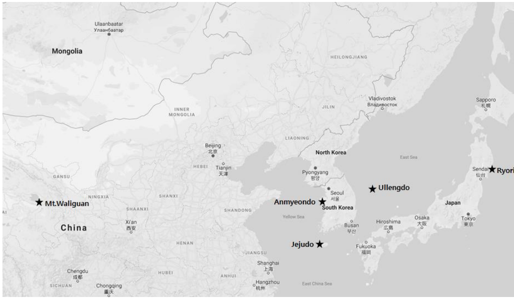
Figure 1. Locations of the three KMA monitoring stations in Korea, and Mt. Waliguan WMO/GAW global station and Ryori WMO/GAW regional station in East Asia.
