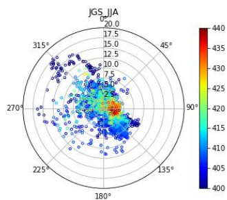
Figure 5. Bivariate polar plots for observed CO 2 (L1) in winter (a), spring (b), summer (c), and autumn (d) at JGS in 2016
