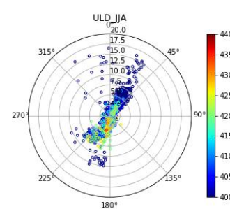
Figure 6. Bivariate polar plots for observed CO 2 (L1) in winter (a), spring (b), summer (c), and autumn (d) at ULD in 2016
