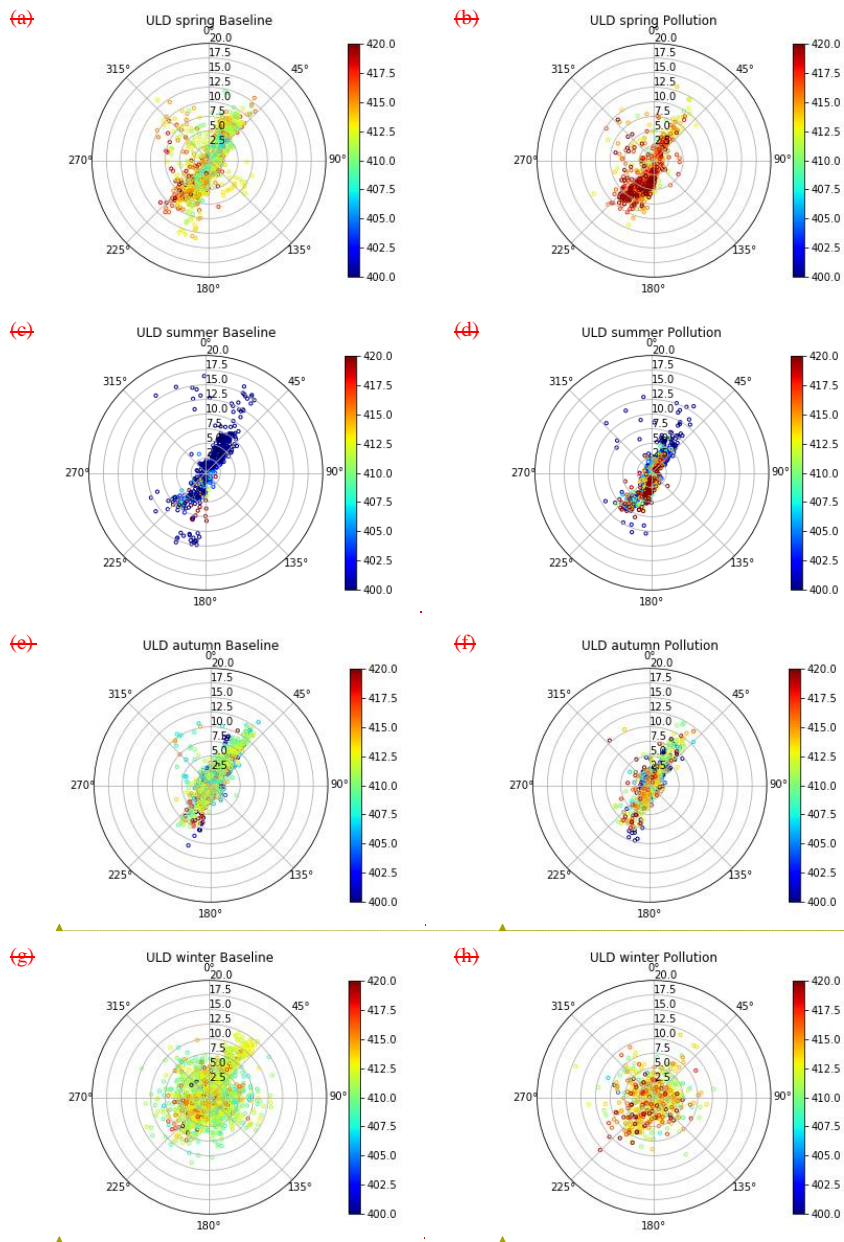
Figure 6. Bivariate polar-plots for (left panel) selected baseline \text{CO}_2 (L2) and (right panel) polluted \text{CO}_2 in spring (L1-L2) (a and b), summer (c and d), autumn (e and f), and in winter (g and h) at ULD in 2016.
