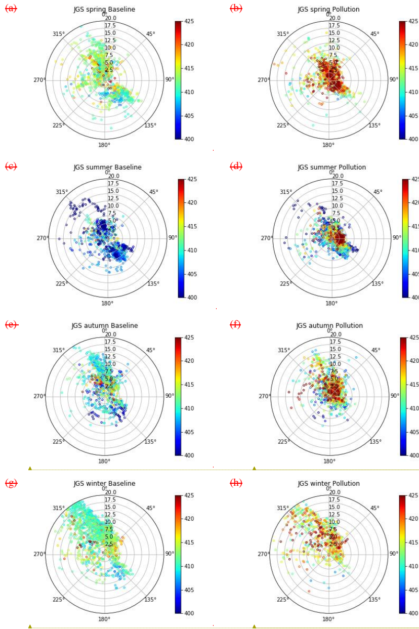
Figure 5. Bivariate polar-plots for (left panel) selected baseline \text{CO}_2 (L2) and (right panel) polluted \text{CO}_2 in spring (L1-L2) (a and b), summer (c and d), autumn (e and f), and in winter (g and h) at JGS in 2016.
