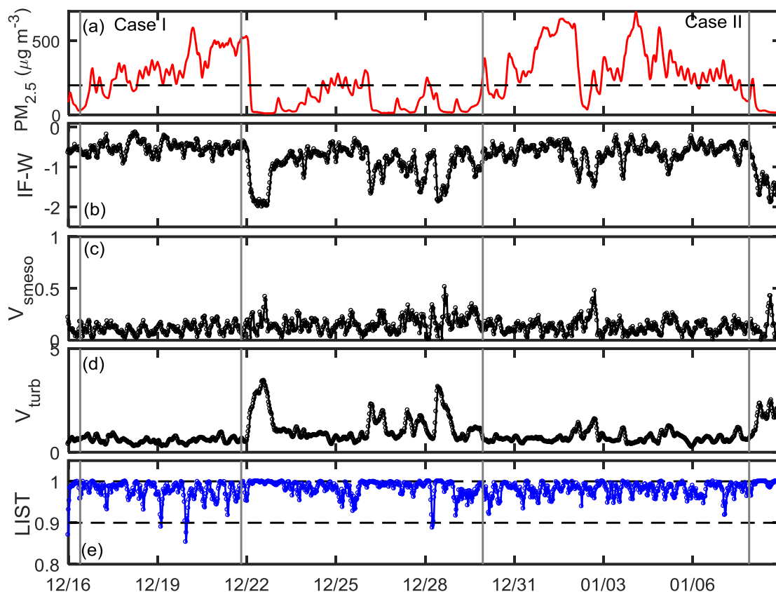
Figure 8: Time series of the (a) PM_{2.5} concentrations, (b) intermittency factor (IF) of vertical velocity, (c) velocity scale of submesoscale motions ( V_{smeso} ), (d) velocity scale of turbulence ( V_{turb} ), and (e) LIST from 16 December 2016 to 8 January 2017 at the city site.
