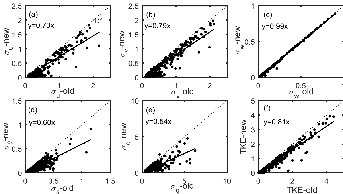
Figure 4: Comparison of \sigma_u (a), \sigma_v (b), \sigma_w (c), \sigma_\theta (d), \sigma_q (e) and TKE (f) from the new half-hour results with those from the old results from 16 December 2016 to 8 January 2017 at the suburban site. The black dotted line represents the 1:1 line in the figures. The black solid line represents the fitted results.
