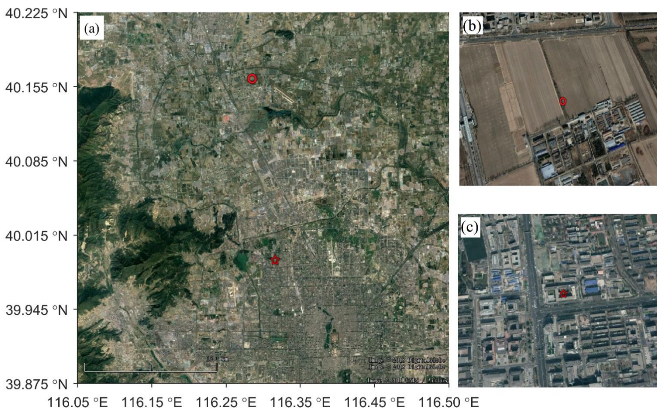
Figure 1: Google Earth map of the observation sites in Beijing: (a) the observation site located in the urban underlying surface region (marked by the red pentagram) and the observation site located in the suburban underlying surface region with a flat terrain (marked by the red concentric circle). The corresponding terrains (within a range of approximately 500 m) around the observation sites are shown in (b) and (c), respectively.
