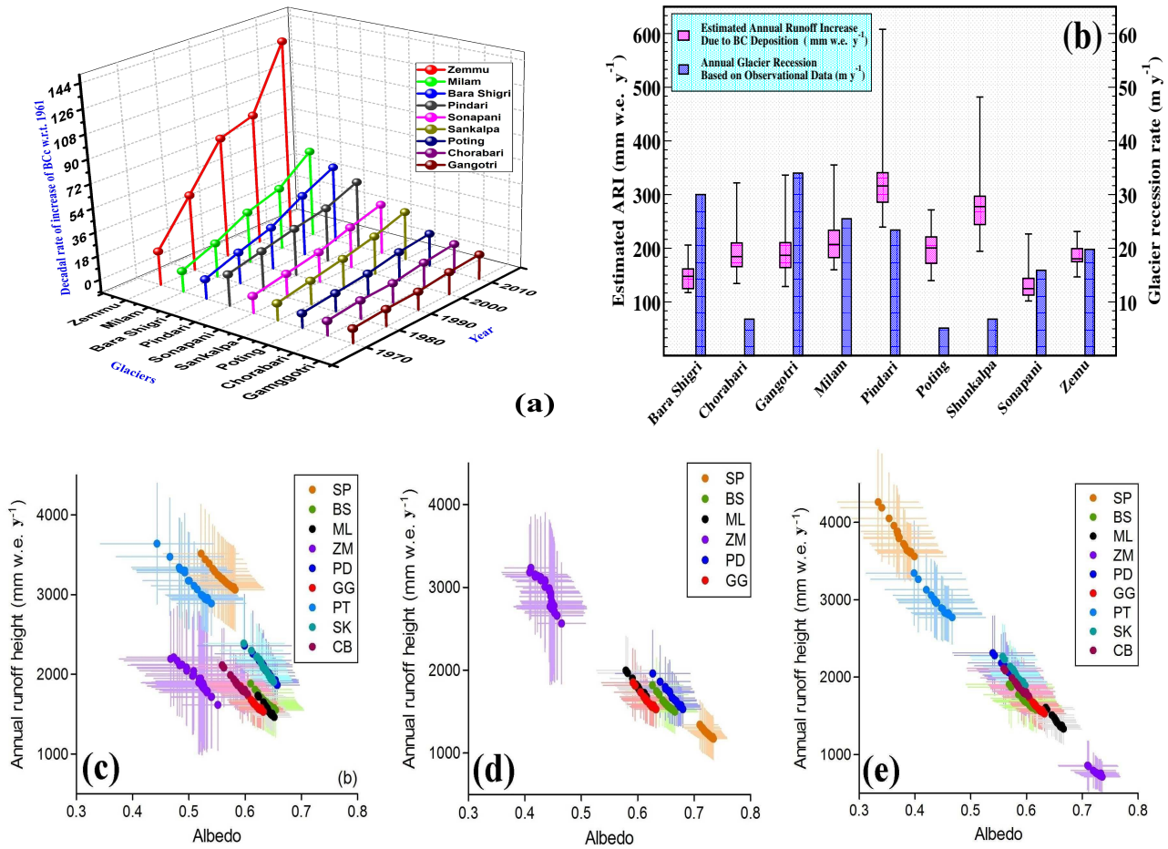
Figure 3. (a) Glacier wise decadal trend (1961–2010, % rate of increase w.r.t 1961) of BC_c based on atmospheric BC concentration ( \mu g\ m^{-3} ) modeled over the glacier using SPRINTARS, (b) Estimated increase in annual glacier runoff ( mm\ w.e.\ y^{-1} ) shown as box-whisker plot and average yearly recession ( m\ y^{-1} ) for the nine glaciers, (c) Simulated impact of summer mean albedo reduction on and annual glacier runoff depth of glaciers, (d-e) Simulated impact and those of albedo reduction on annual glacier runoff sensitivity analysis for (d) a single glacier hypsometry at different ERA-Interim grids and (e) different glacier hypsometries at a single ERA-Interim grid
