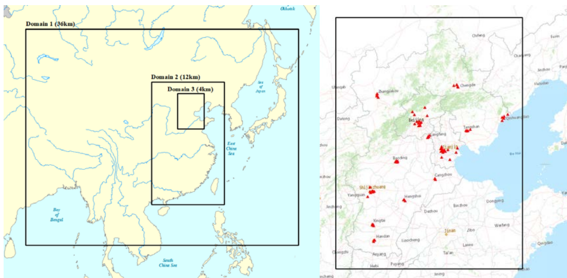
Fig. 1 The three-domain nested CMAQ domain (left) and the observational sites in Beijing-Tianjin-Hebei region (right)
