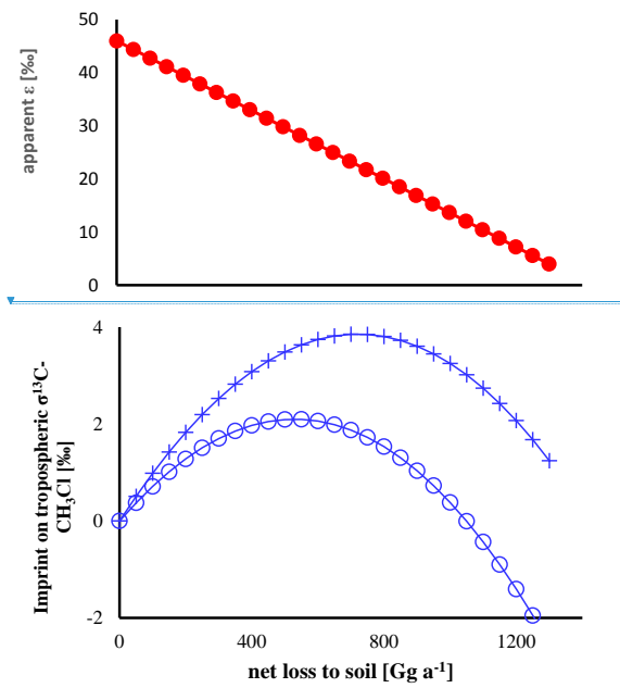
5 Figure 4: The upper panel shows the apparent \epsilon of the soil sink versus the sink strength. The lower panel shows the resulting effect on tropospheric \delta^{13}\text{C} . Crosses show the pure effect e.g. in the absence of any other fractionating sink. Open circles show the resulting effect with an \epsilon of -11.2\% assigned to the OH sink. Total losses were assumed to be fix at 4010 \text{ Gg a}^{-1} .
