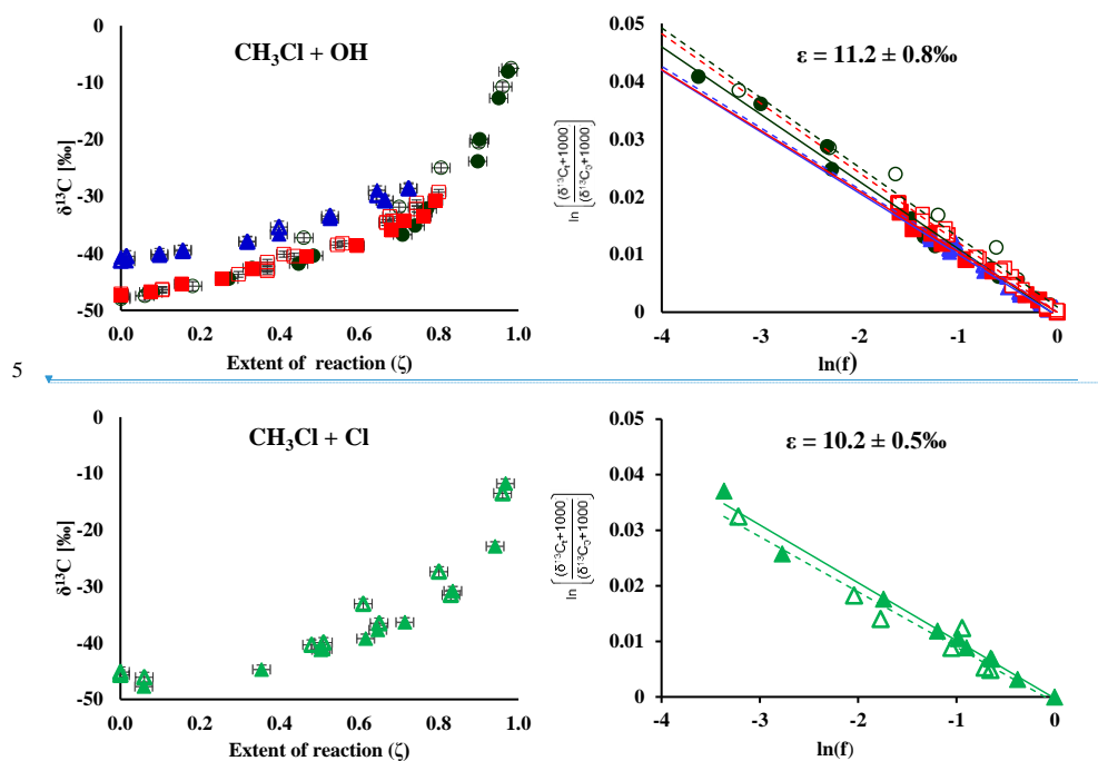
Figure 1: Change in \delta^{13}\text{C} over extent of reaction (left hand side) and corresponding Rayleigh plots (right hand) from the \text{CH}_3\text{Cl} degradation experiments. Filled symbols and regression lines refer to the data from Heidelberg, open symbols and dashed regression lines show data from Hamburg. The colors refer to different degradation experiments (black: experiment 1; red: experiment 2, blue: experiment 4 and green: experiment 7). Errors in \zeta were \pm 2\% on the 1\sigma level. Errors in \delta^{13}\text{C} , as derived from the regression analysis, ranged from \pm 0.4 to \pm 1.4\% on the 1\sigma level.
