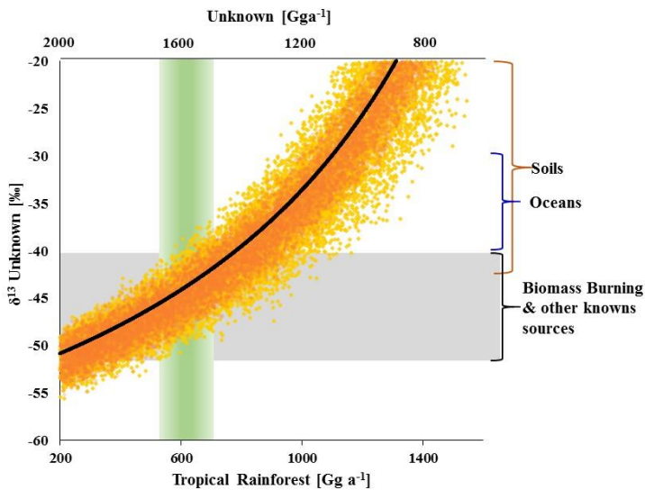
Figure 5: Modeled isotopic composition of the missing source versus tropical rainforest emissions on the lower x-axis and missing emissions on the upper x-axis (rainforest = 2200 – unknown). The black line shows the best estimate derived from the mean isotopic source signatures. Orange dots indicate the range uncertainty ( 1\sigma ) from uncertainties ( \pm 6\% ) in the \delta^{13}\text{C} of biomass burning ( \pm 7\% ), ocean net emissions ( \pm 6\% ) and other known sources ( \pm 6\% ). Yellow dots mark the additional uncertainty from the \delta^{13}\text{C} of the tropical rainforest source ( \pm 10\% ). The green column indicates the carbon density based estimate of the rainforest source and the grey bar indicates the range in \delta^{13}\text{C} of biomass burning and the mean from all sources excluding the tropical rainforest.
