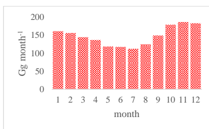
Figure 3: Chloromethane emissions in Gg month -1 for the northern (left side) and southern hemisphere (left side) Upper row panel: Combined emissions from higher plants and the unknown source; second row panel: biomass burning, third row panel: ocean net emission fluxes, fourth row panel total emissions. The emissions from the other known sources are constant over time with 22.8 Gg month -1 in the northern hemisphere and 7.6 Gg month -1 in the southern hemisphere.
