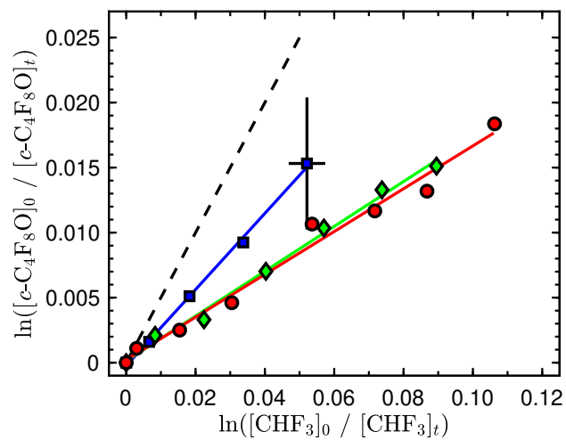
Figure 3. Relative rate data obtained in this work for the O(^1D) + c\text{-}C_4F_8O reaction at 296 K. The different symbols are results from independent experiments and the solid lines are linear least-square fits to the data of the individual experiments. Representative estimated error bars from the infrared spectral analysis are included only on a single data point for improved clarity of the graph. The dashed line represents the upper-limit rate coefficient ratio recommended in this work.
