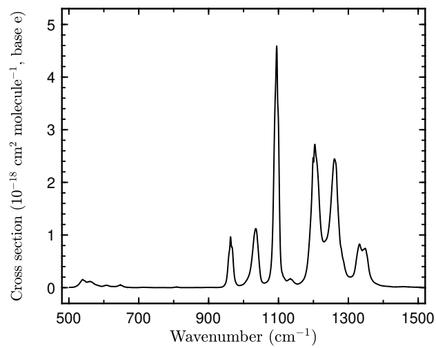
Figure 1. Infrared absorption spectrum of octafluorooxolane ( c -C 4 F 8 O) measured in this work at 296 K at 1 cm -1 resolution.
