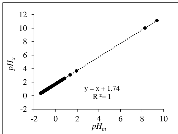
Figure S1. Comparison of pH_x and pH_m
