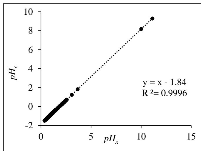
Figure S2. Comparison of pH_x and pH_c
