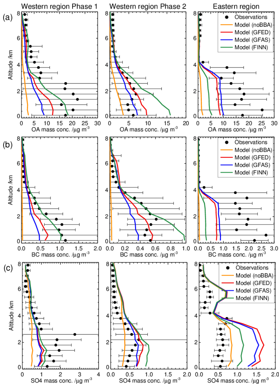
Figure 5. Mean observed and simulated vertical profiles of (a) organic aerosol (OA), (b) black carbon (BC) and (c) sulfate (SO 4 ) during the SAMBBA aircraft campaign, sectioned into 400 m altitude bins. Observations are shown by the black data points; simulated concentrations are shown for the model with FINN1.5 (green), GFAS1.2 (blue), GFED4 (red) emissions and with no biomass burning emissions (noBBA; orange). The simulated data (linearly interpolated to the flight track of the
