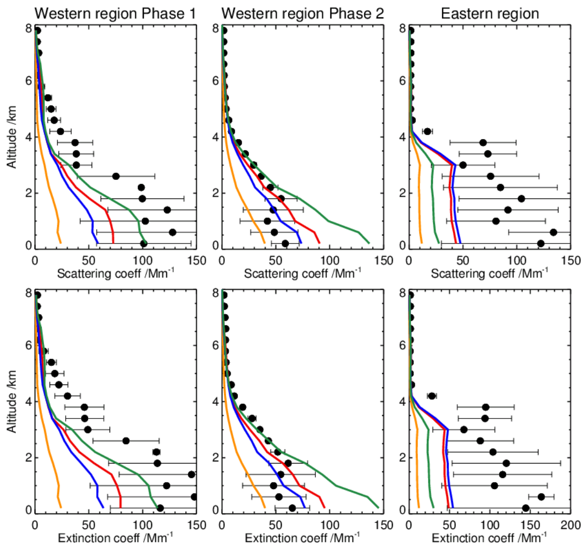
Figure 9. Vertical profiles of observed (black) and simulated (colour) aerosol scattering coefficient at 550 nm (top panel) and extinction coefficient at 550 nm (bottom panel) during the SAMBBA aircraft campaign, sectioned into 400 m altitude bins. Observations are shown by the black data points; simulated concentrations are shown for the model with FINN1.5 (green), GFAS1.2 (blue), GFED4 (red) emissions and with no biomass burning emissions (orange). The simulated data (linearly interpolated to the flight track of the aircraft) and the observations are split into western and eastern regions of the Amazon (Fig. 2) and by time (Phase 1: 13/09/2012 – 22/09/2012, Phase 2: 23/09/2012 - 03/10/2012) for the western region. Error bars show the standard deviation of the observed mean. The NMBF values are given separately for the western region (Phase 1 and Phase 2) and eastern region in Table 2.
