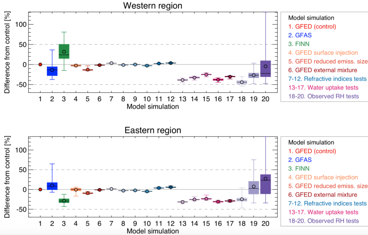
Figure 10. Box and whisker plot summarising the relative difference between simulated hourly mean AOD550 from the control simulation (GFED emissions with ZSR water uptake scheme) and each of the sensitivity simulations listed in Table 3. Simulation numbers in the figure correspond to the simulation numbers in Table 3. Simulations are compared during the SAMBBA campaign period (13 September – 3 October 2012) for the western region (54–68.5°W, 6–12°S; top panel) and the eastern region (43–50°W, 4.5–15°S; bottom panel) separately. Simulations 18, 19 and 20 are compared to the control simulation only on days with available aircraft measurements of RH. Circles show the mean values; whiskers show the minimum and maximum values; boxes show the 25 th and 75 th percentiles; and horizontal lines show the median values.
