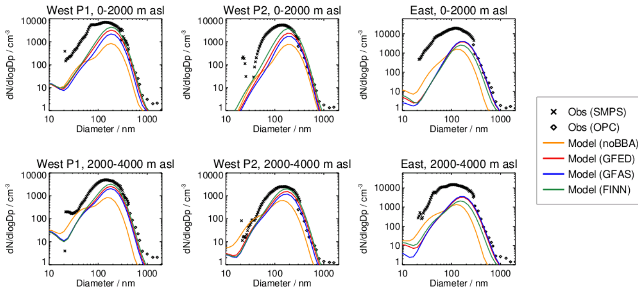
10 Figure 6. Mean observed (black) and simulated (colour) aerosol number size distributions during the SAMBBA aircraft campaign for two altitude bands: between the surface and 2 km (top panel) and between 2 and 4 km asl (bottom panel). The observed number size distribution was measured with Scanning Mobility Particle Sizer (SMPS; black crosses) and a Grimm optical particle counter (OPC; black diamonds). The simulated data (linearly interpolated to the flight track of the aircraft) and the observations are split into western and eastern regions of the Amazon (Fig. 2) and by time (P1: 13/09/2012 – 15 22/09/2012, P2: 23/09/2012 - 03/10/2012) for the western region. Simulated concentrations are shown for the model with FINN1.5 (green), GFAS1.2 (blue), GFED4 (red) emissions and with no biomass burning emissions (noBBA; orange).
