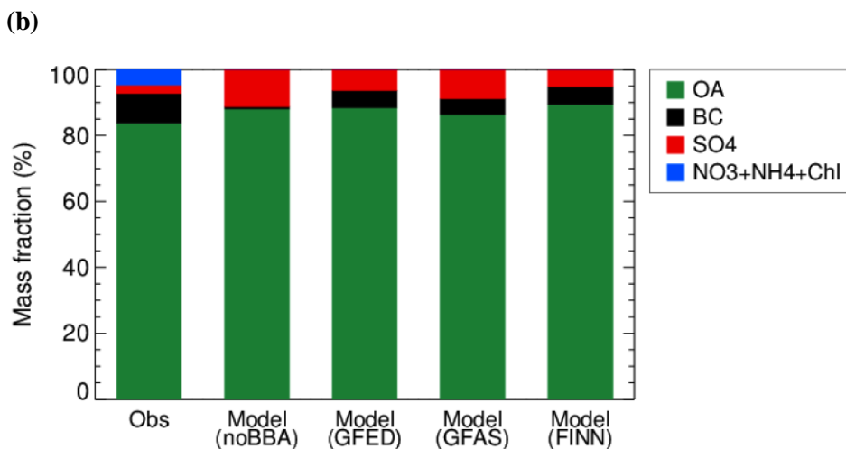
Figure 4. Composition resolved aerosol mass at Porto Velho ground station during the SAMBBA campaign. (a) Time series of hourly-mean observed (black) and simulated (colour) total aerosol mass. The observed aerosol mass is the total mass from the ACSM plus equivalent BC from the aethelometer. Simulated total aerosol mass is shown for the model with FINN1.5 (green), GFAS1.2 (blue), GFED4 (red) emissions and with no biomass burning emissions (noBBA; orange). Numbers on the panel show the NMBF for the SAMBBA campaign separately for Phase 1 (P1) and Phase 2 (P2) (also see Table 2). (b) Bar chart showing observed and simulated average aerosol composition during the campaign: black carbon (BC; black), nitrate+ammonium+chloride (NO 3 +NH 4 +Chl; blue, not treated by the model), organic aerosol (OA; green) and sulfate (SO 4 ; red). 10
