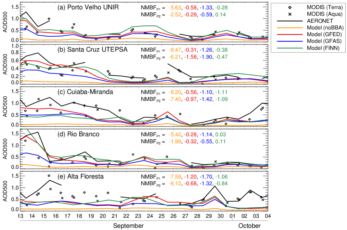
Figure 8. Time series of simulated (colour) and observed (black) daily aerosol optical depth (AOD) during the SAMBBA campaign at 5 AERONET stations in the western and southern Amazon: (a) Porto Velho UNIR (63.94°W, 8.84°S), (b) Santa Cruz UTEPSA (63.20°W, 17.77°S), (c) Cuiaba-Miranda (56.02°W, 15.73°S), (d) Rio Branco (67.87°W, 9.96°S) and (e) Alta Floresta (56.10°W, 9.87°S). Daily mean AOD at 500 nm (AOD500) from AERONET (black line) is compared to AOD500 retrieved by MODIS (Terra: black diamonds; Aqua: black crosses), using grid cells nearest the AERONET station location. Simulated daily mean AOD500 is shown for the model with FINN1.5 (green), GFAS1.2 (blue), GFED4 (red) emissions and with no biomass burning emissions (noBBA; orange). The NMBF values are given separately for Phase 1 (P1) and Phase 2 (P2) of the campaign.
