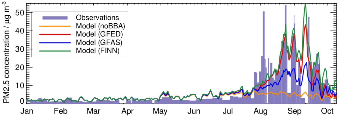
Figure 3. Time series of simulated (lines) and observed (bars) PM 2.5 concentrations at Porto Velho between January and November 2012. Simulated daily mean concentrations are shown with FINN1.5 (green), GFAS1.2 (blue), GFED4 (red) emissions and with no biomass burning emissions (noBBA; orange). Observed PM 2.5 concentrations are averages over sampling periods that ranged from <1 day to 7 days in 2012. The NMBF values are given separately for Phase 1 and Phase 2 of the SAMBBA field campaign in Table 2.
