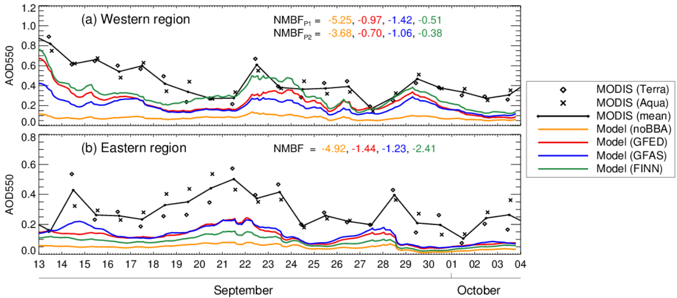
Figure 7. Time series of simulated (colour) and observed (black) aerosol optical depth at 550 nm (AOD550) for the SAMBBA campaign (13 September – 3 October 2012) over (a) the western Amazon (54-68.5°W, 6-12°S) and (b) the eastern Amazon (43-50°W, 4.5-15°S). Observed AOD550 retrieved by MODIS on-board Terra (over pass time: 10:30 local time) is shown by the black diamonds and AOD550 retrieved by MODIS on-board Aqua (over pass time: 13:30 local time) is shown by the black crosses; the black line shows an average value for each day (plotted at midday local time). Simulated hourly AOD550 (plotted at local time for Rondônia, Brazil: UTC-4h) is shown for the model with FINN1.5 (green), GFAS1.2 (blue), GFED4 (red) emissions and with no biomass burning emissions (noBBA; orange). The NMBF values are given separately for the western region (Phase 1 and Phase 2) and eastern region in Table 2.
