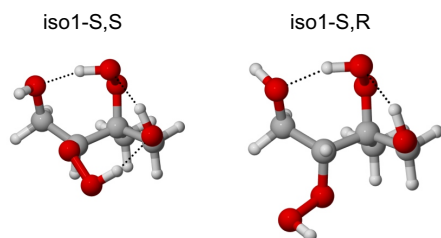
5 Figure 4. Lowest-energy conformers (at the BP/def2-TZVPD/BP/def-TZVP level, with COSMO solvation, using the systematic configurational sampling scheme) of the S,S (left) and S,R (right) stereoisomers of structural isomer 1 of ISO(POOH) 2 . The S,R stereoisomer only has two intramolecular H-bonds in the lowest-energy conformer while the S,S isomer has three. Correspondingly, the saturation vapor pressure of the S,R stereoisomer is predicted to be a factor of 15 lower. Color coding: gray=C, red=O, white=H.
