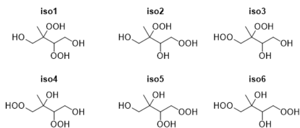
Figure 1. Structural isomers of ISOP(OOH) 2 .
